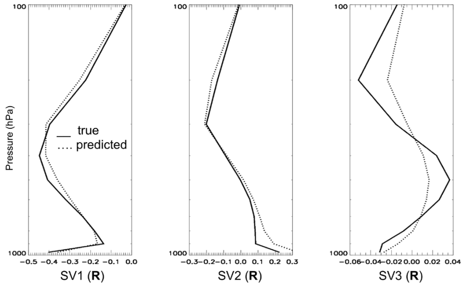
Fig. 9. Example of a test case to evaluate the prediction for singular vectors (SV) for the rotated AK ( \mathbf{R} ) for a single MOPITT observation. Solid lines indicate the true rows of \mathbf{R} from the test case observation; dotted lines indicate the results of the prediction using MR coefficients from the training set and the state parameters from the test case observation as input.
