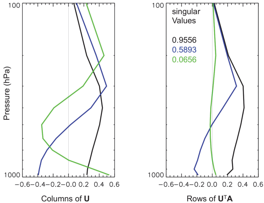
Fig. 5. (Left) Left singular vector ( U ) from the SVD of the MOPITT 2006 CONUS average CO AK (1st 3 ranked columns). (Right) 1st 3 rows of the rotated average AK ( R ) with corresponding singular values.
