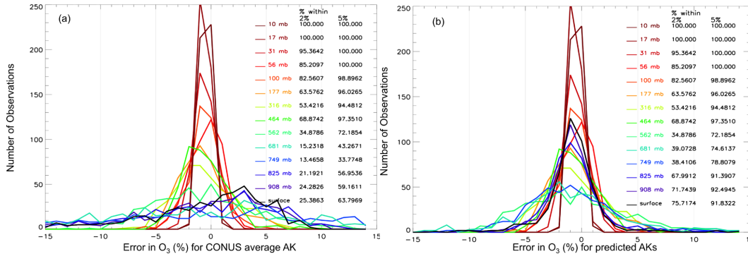
Fig. 16. (a) Performance of CONUS average AK compared to true AKs for TES-OMI test cases. (b) Performance of predicted AKs compared to true AKs for TES-OMI test cases. For pressures below 600 hPa, the CONUS average AK is applied. Histograms of error in O 3 are plotted for each pressure (indicated by colors on the right). Listed on the far right are the percentages of test cases that fall within 2 % and 5 % O 3 error for each pressure.
