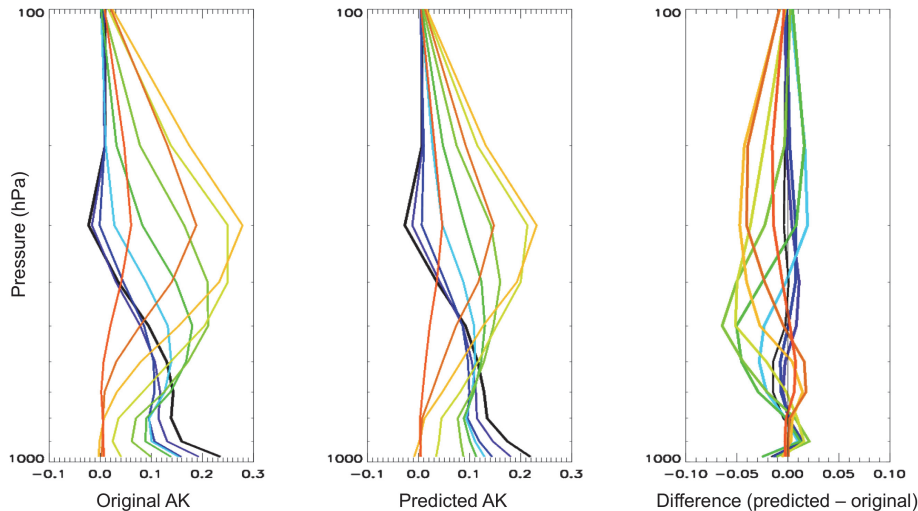
Fig. 10. Example of original MOPITT test case AK and corresponding predicted AK using the results of the MR prediction shown in Fig. 9 to reconstruct the predicted AK. Difference between predicted and original AKs is shown on the right.
