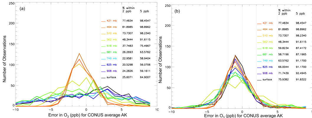
Fig. 17. (a) Performance of CONUS average AK compared to true AKs for TES-OMI test cases. (b) Performance of predicted AKs compared to true AKs for TES-OMI test cases. For pressures below 600 hPa, the CONUS average AK is applied. Histograms of O_3 error in ppb are plotted for each pressure (indicated by colors on the right). Listed on the far right are the percentages of test cases that fall within 2 ppb and 5 ppb O_3 error for each pressure.
