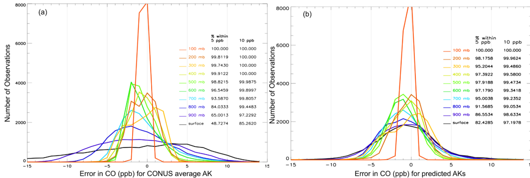
Fig. 15. (a) Performance of CONUS average AK compared to true AKs for MOPITT test cases. (b) Performance of predicted AKs compared to true AKs for MOPITT test cases. Histograms of error in CO are plotted for each pressure (indicated by colors on the right). Listed on the far right, are the percentages of test cases that fall within 5 and 10 ppb CO error for each pressure. See text for description of error calculation.
