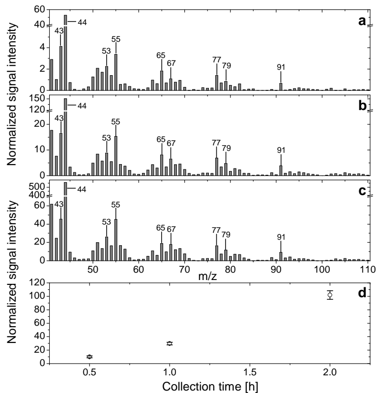
Fig. 6. Mass spectra of organic particles with a diameter of 25 nm from dark ozonolysis of alpha-pinene; (a–c) are spectra after collection times of 0.5 h, 1 h and 2 h, respectively. The lower panel (d) shows the sum of the signal intensities of four major peaks ( m/z 55, 65, 77 and 91) in relation to the collection time.
