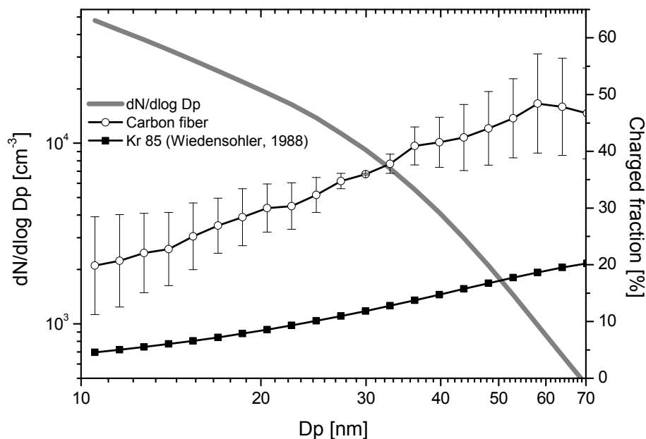
Fig. 2. Size dependent extrinsic charging efficiency of the unipolar carbon fiber corona charger, and singly positive charged particle fraction for the theoretical bipolar charge equilibrium (Wiedensohler, 1988). Additionally, the number size distribution of the aerosol used for characterization is shown.
