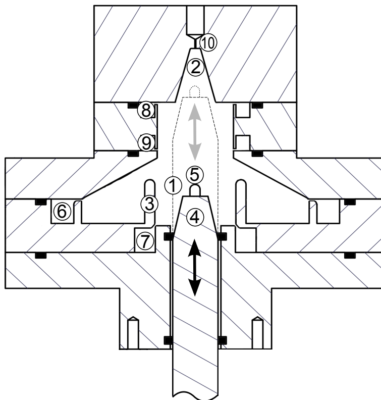
Fig. 4. Schematic of the radial collection and desorption unit with NiCr filament in collection position: (1) collection region, (2) desorption region, (3) collection tube, (4) PEEK piston, (5) collection filament, (6) aerosol inlet, (7) collection flushing inlet, (8) desorption flushing inlet, (9) exhaust and (10) screw connection for transfer capillary. Positions of O-rings are shown in black.
