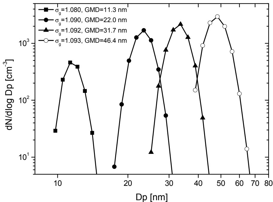
Fig. 3. Examples of quasi monodisperse aerosol particle distributions with geometric mean diameters (GMD) of 11.3 nm, 22 nm, 31.7 nm, and 46.4 nm, separated by the rDMA.
