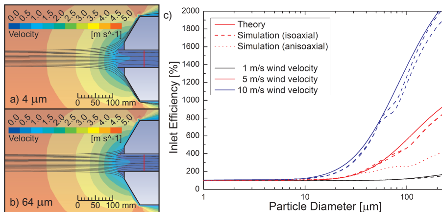
Fig. 3. Simulations of the HOLIMO II inlet. Particle sampling for (a) 4 \mu\text{m} and (b) 64 \mu\text{m} diameter spheres was simulated in a 5 \text{ m s}^{-1} ambient wind field. The detection plane is indicated by a red line in (a) and (b) . In both cases, wind deceleration begins 20 cm ahead of the inlet tip. Due to inertia, the larger particles in (b) deviate from the air flow around the inlet and become enriched in the sample volume. In (c) simulated (dashed lines, multiple runs) and theoretical (solid lines, Paik and Vincent, 2002; Liu et al., 1989) results are compared for three different wind velocities. An additional simulation (red dotted line) is shown for anisoaxial sampling of 15^\circ for a wind velocity 5 \text{ m s}^{-1} .
