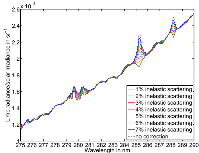
Fig. 6. Result of the Ring effect correction for a tangent altitude of 53.5 km for the ratio I/F . Shown are the uncorrected spectrum and the corrected spectra with different percentages of Raman scattering in the applied method. The emission signals become smaller with this correction and the Mg line at 285.2 nm as well as the Si line at 288 nm, that can not be observed in the region between 90 to 100 km and originates probably purely from Ring effect, nearly vanish for the Ring correction with 4 % of inelastic scattering in the background signal.
