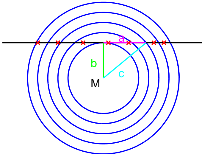
Fig. 15. 2-D intersection of earth's atmosphere, with the center of earth M, and the altitudes as radii of the circles. Path lengths along the LOS for the vertical grid can be found with right-angled triangle algebra. Changes of the latitude in a vertical grid cell are added as additional sides a (red crosses). The path length in each grid cell is the difference of the sides a of neighboring grid cells. Note that depending on the binning of the latitudes, it is possible, that all grid cells only have one latitude.
