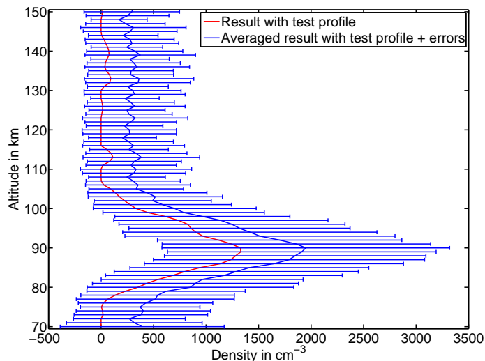
Fig. 24. Retrieval of Mg (285.2 nm). The same methods as in Fig. 21 are applied. However, here the single measurements error is used. As for high relative errors the error propagation can not be approximated to be linear and non-linearities in the forward model lead to a shift of the mean to higher values. Therefore, a certain averaging of the data is needed before applying the retrieval algorithm. Note that the errorbars estimate the error of single measurements while the error for the blue line is a factor \sqrt{1000} \approx 32 smaller.
