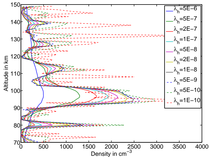
Fig. 26. Single day (7 September 2009) result for \text{Mg}^+ (279.6 nm) in the equatorial region from 15^\circ\text{S} to 15^\circ\text{N} . The same approach to find the optimal constraint strength as for Mg (see Fig. 25) is applied for \text{Mg}^+ . However the variation of the peak density with constraint strength, especially for low strength, is much weaker, so errors from a wrong choice of the constraint strength are smaller. For \text{Mg}^+ the solution with \lambda_h = 1 \times 10^{-7} will be used for further investigations.
