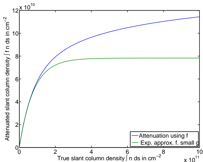
Fig. 20. Plot of attenuated SCDs versus the true SCDs for the Mg 285.2 nm line. The attenuated SCDs are determined using f , respectively the exponential approximation of f for small true SDSs. Typical measured SCDs (y-axis) in the peak region for Mg are 6\text{--}8 \times 10^{10} \text{ cm}^{-2} . The exponential approximation can not be used in the retrieval, since it is already saturated below 8 \times 10^{10} \text{ cm}^{-2} . For Mg the self absorption effect is that strong, that the measured SCDs are a factor 3 to 4 smaller than the true SCDs in the Peak region. For \text{Mg}^+ (not in the plot) the conversion factor is close to 1.
