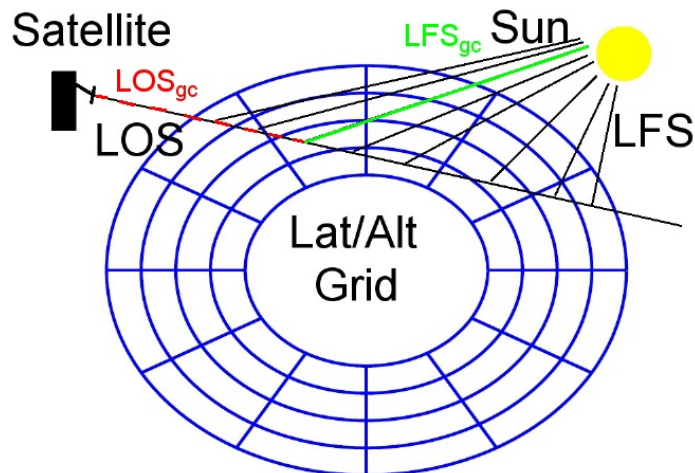
Fig. 13. Scheme of the altitude (radius) and latitude (sectors) grid and the LOS and LFS. Each grid element may have a different LFS. Note that this figure shows only a specific 2-D projection of the atmosphere, along a constant meridian, so that latitude sectors are equally sized. Each grid cell on the LOS has its own matrices for the LFS from the sun to the grid cell and the LOS from the grid cell to the satellite, which are needed for absorption calculations.
