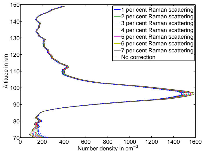
Fig. 31. Plot of Mg + (279.6 nm) average profile of all single day results of the 2-D retrieval in the equatorial region (15° S to 15° N) for different percentages of Raman scattering in the Ring effect correction. For altitudes above 80 km the Ring effect correction is negligible and it is very small above 70 km. In the peak region the emission dominates the background signal. Because of this the peak value rises with higher Raman scattering percentage (as discussed in Sect. 3.2.2).
