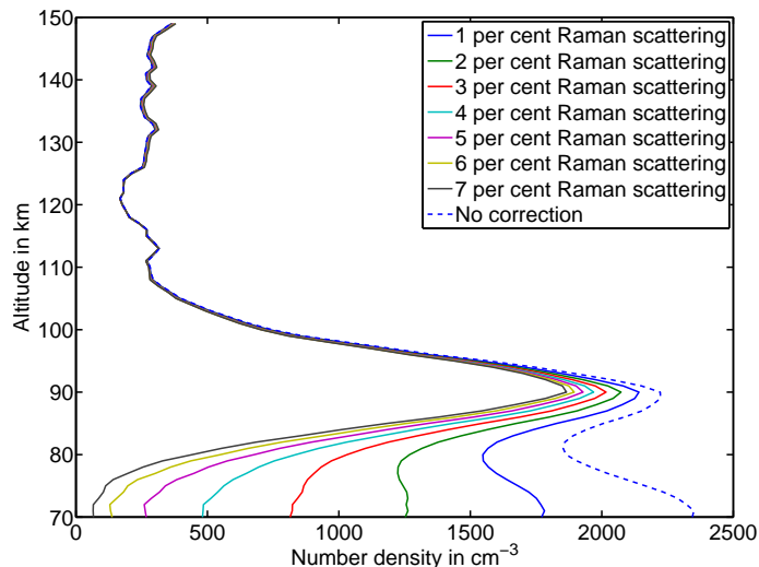
Fig. 30. Plot of Mg average profile of all single day results of the 2-D retrieval in the equatorial region ( 15^{\circ} S to 15^{\circ} N) for different percentages of Raman scattering in the Ring effect correction. The different corrections mainly affect the peak density and the lower peak edge. The peak altitude is nearly unaffected. Differences for variations of 1 % in the Raman scattering percentage vary the lower peak edge altitude by \approx 1 km, for altitudes above 80 km. For altitudes below 80 km the differences drastically raise.
