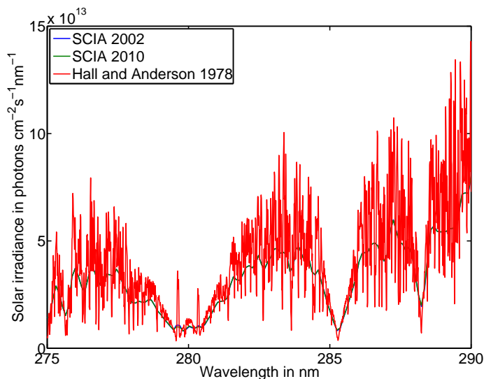
Fig. 9. High resolution solar spectrum from Hall and Anderson (1991) (data from 1978) in comparison to the SCIAMACHY solar irradiance spectrum during high solar activity (2002) and low solar activity (2010). There are especially strong differences between the high resolution spectrum and the SCIAMACHY spectrum in the Fraunhofer lines at 279.6, 280.4, 285.2 and 288.2 nm. When smoothed and scaled, the high resolution spectrum is very similar to the SCIAMACHY spectrum (see Fig. 10).
