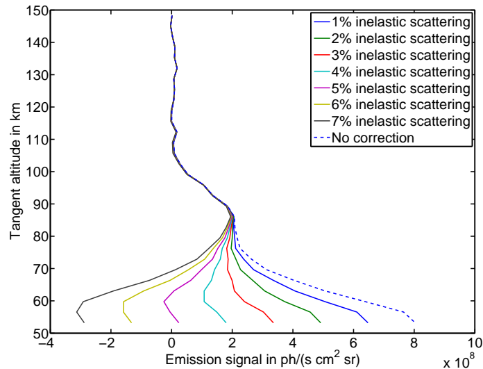
Fig. 8. Vertical SCE profile with different percentage of inelastic scattering in the Ring effect correction. The difference between the corrected and uncorrected profile increases with decreasing tangent altitude below 90 km. Note that the SCE of Mg at 53.5 km is still in the order of 50 % of the SCE at 90 km, for typical recalculations of the forward model from retrieval results.
