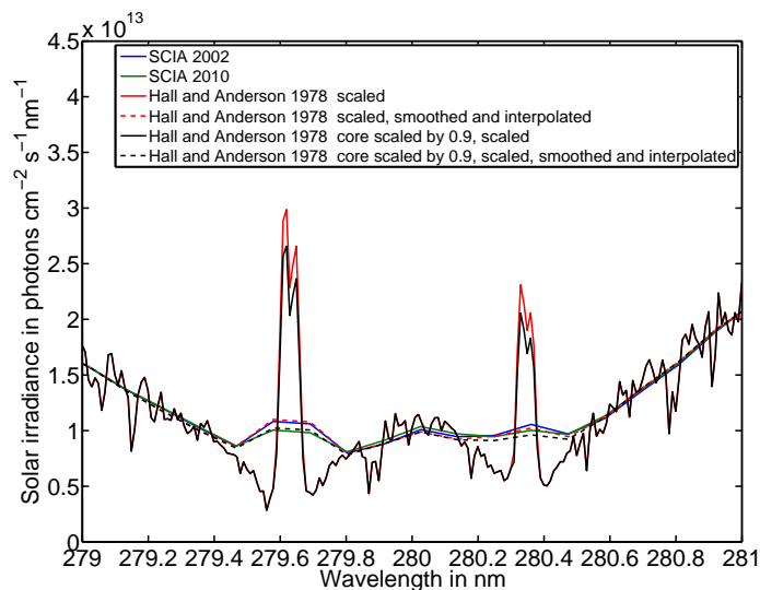
Fig. 12. SCIAMACHY solar spectrum in the \text{Mg}^+ double line region for low (2010) and high (2002) solar activity in comparison with the scaled high resolution reference spectrum. When the high resolution spectrum is smoothed and sampled as the SCIAMACHY spectrum there are only small differences left between both, mainly resulting from different phases of the solar cycle for the different spectra. An adjustment for the solar phase is done by scaling the core of the emission lines. The adjustment has to be done for each line individually. Possible variations of the inner structure of the the emission lines are not considered.
