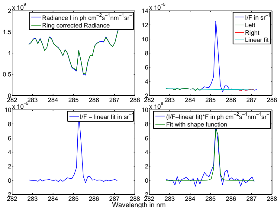
Fig. 3. SCE determination. First the Ring effect correction is applied to the limb radiance I (top left panel). The limb radiance is divided by the solar irradiance F and the wavelength region left and right to the line are used for a linear fit of the background radiation (top right panel). The linear fit is subtracted from the ratio I/F (bottom left panel) and the the spectrum is again multiplied with the solar irradiance F (bottom right panel). Finally the area of the emission line is fitted with the slit function of the instrument.
