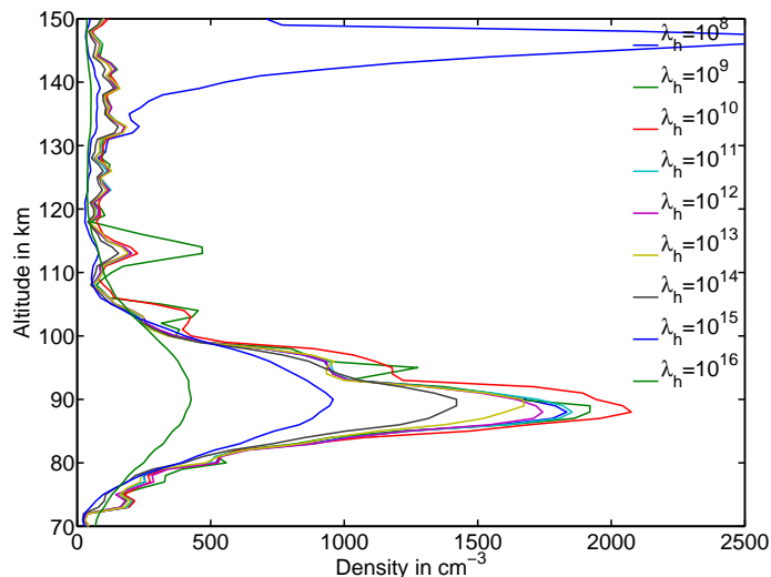
Fig. 29. Retrieval results with a 1-D model, when an error is applied for Mg with the same method as for the blue line in Fig. 21. The constraint strength is varied. Oscillating results start already at much higher constraint strength as for the error free case shown in Fig. 28. Furthermore, the result varies much stronger with changing constraint strength, so that it is once again difficult to find the constraint strength for the optimal solution. For the case of very strong smoothing, the same profiles as in the error free case are retrieved for the same constraint strength.
