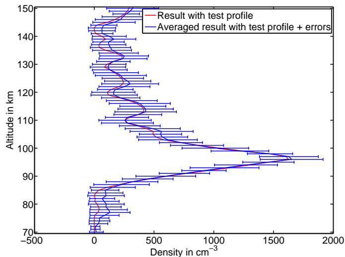
Fig. 23. \text{Mg}^+ (280.4 nm) retrieval result. The same methods as in Fig. 21 are applied. The errors for \text{Mg}^+ are smaller than for Mg and furthermore non-linear self-absorption effects are smaller for \text{Mg}^+ . Therefore, both methods lead to the same mean results.
