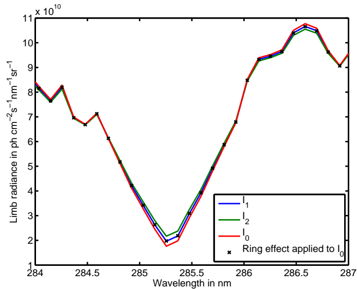
Fig. 4. Ring effect correction for the Mg 285.2 nm line, for a limb measurement with a tangent altitude of 53.5 km. The Ring effect is simulated, using the measured spectrum I_1(\lambda) , to obtain I_2(\lambda) . The filling-in effect is assumed to be small and differences between the first and the second application are therefore also very small. Under this assumption the differences are the nearly the same I_0(\lambda) - I_1(\lambda) \approx I_1(\lambda) - I_2(\lambda) . And by adding I_1(\lambda) the corrected spectrum I_0(\lambda) is obtained as I_0(\lambda) = 2I_1(\lambda) - I_2(\lambda) .
