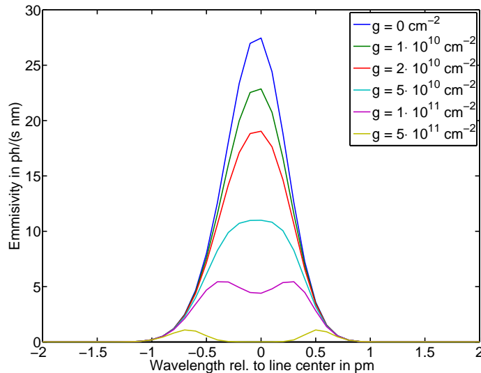
Fig. 17. Calculation of the wavelength specific emissivity for the Mg 285.2 nm line as a function of wavelength difference from the center of line. It is the product solar irradiance attenuated along the LFS and the LOS and the absorption cross section (both shown in Fig. 16). To obtain the emissivity of the spectral line, this spectrum has to be integrated over all wavelengths. For strong absorption the light comes mainly from the edges of the profile instead of the core. This reduces the effective cross section for the total integrated profile.
