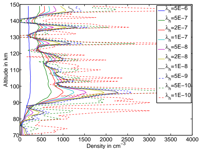
Fig. 27. Result for \text{Mg}^+ (280.4 nm) for the same conditions as in Fig. 26.
