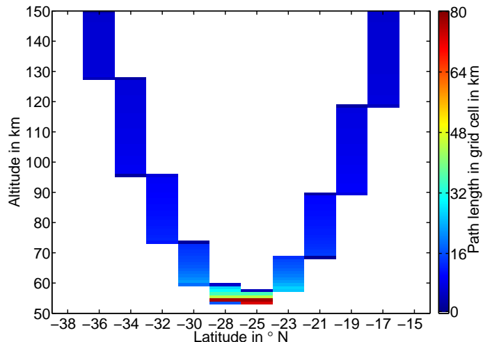
Fig. 14. Path lengths in different grid cells for a typical LOS of a limb measurement. The biggest part of the path lies in the tangent point altitude region, but higher altitudes are also passed. Note that for the contribution of a grid element's emission to the total emission along the LOS the path length in the grid interval as well as the density of the emitters in the grid interval and the absorption of the emitted light along the LOS have to be considered. For measurements with tangent altitudes far below the metal layer peak, where the density is far smaller than in the peak region, the emission signal mainly comes from the region above the tangent altitude.
