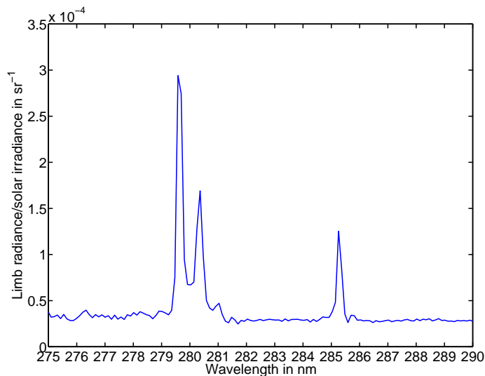
Fig. 1. Limb radiance divided by solar irradiance (average 2008–2012, equator, tangent altitude 89.3 km). Division of both spectra leads to a smooth signal, beside emission lines that are clearly identified. The background signal is separated from the emission lines through a linear fit. Note that beside the strong \text{Mg}^+ at 279.6 and 280.4 nm and the strong Mg line at 285.2 nm very weak NO lines can be observed at the longer wavelength edge of the \text{Mg}^+ lines at 281 nm. However, this influence is negligibly small.
