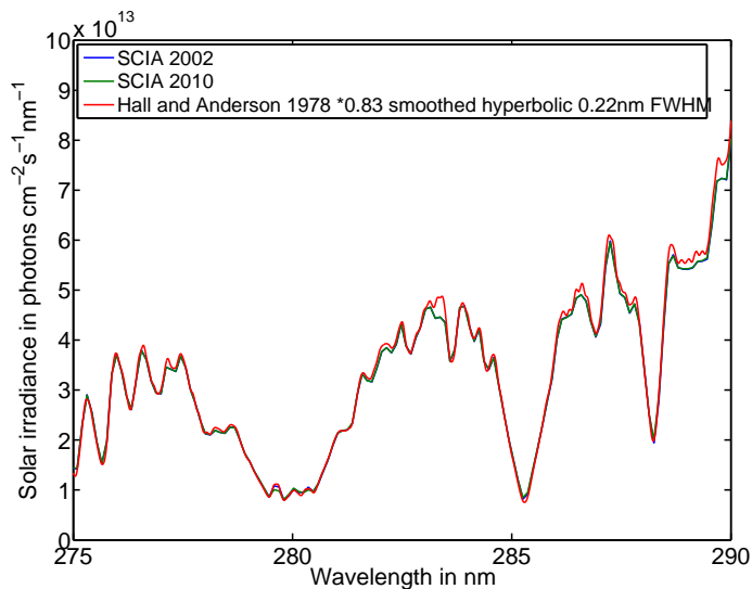
Fig. 10. The high resolution spectrum from Fig. 9 is smoothed and scaled the the SCIAMACHY spectrum by a factor of 0.83, so that the peak edges of the spectra are in agreement.
