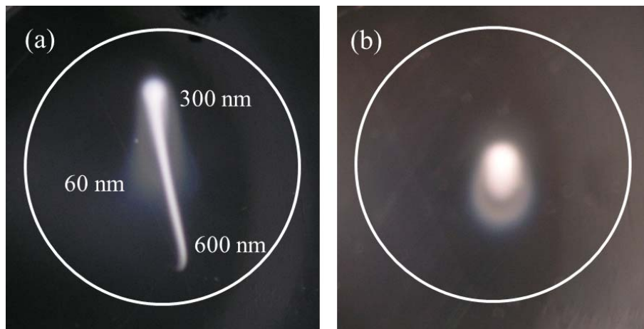
Fig. 6. Deposition patterns of polydisperse \text{NH}_4\text{NO}_3 transmitted by the lens system for (a) HPL SN10 and (b) HPL SN12. The white circle represents the size of the vaporizer. The numbers are approximate particle sizes for different parts of the deposition pattern based on measurements with size selected particles.
