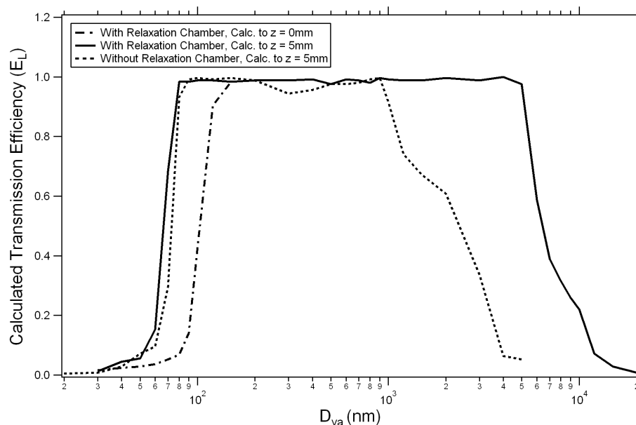
Fig. 3. Calculated transmission efficiency ( E_L ) as a function of particle size with the relaxation chamber, calculated to the exit nozzle ( z = 0 , dash-dot line) and 5 mm past exit nozzle ( z = 5 , solid line), and without the relaxation chamber calculated 5 mm past the exit nozzle ( z = 5 , dashed line).
