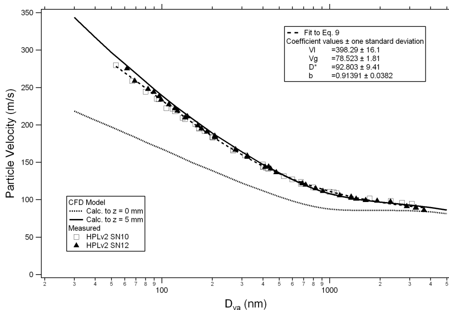
Fig. 4. Calculated velocity as a function of particle diameter with Fluent calculation ending at exit nozzle ( z = 0 , dotted line) and calculation continuing 5 mm past exit nozzle ( z = 5 , solid line). Experimental particle velocity for two different high pressure lenses (squares and triangles) and fit to Eq. (9) (dashed line). The fit parameters are defined in the text.
