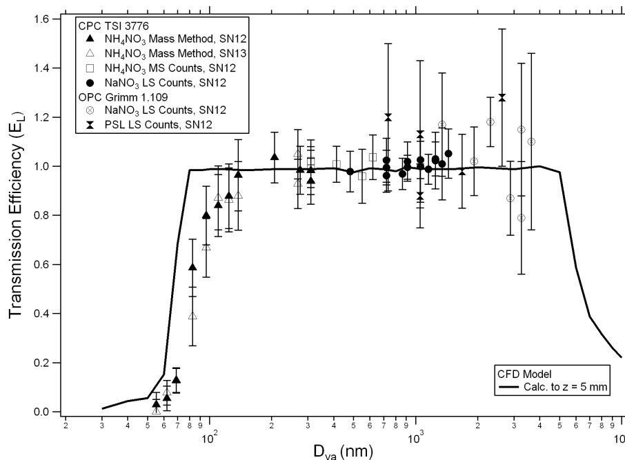
Fig. 5. Experimental transmission efficiency ( E_L ) as a function of particle size for the HPL, using the mass method (triangles) and the count method (other symbols). Particles entering the AMS were counted with a CPC or an OPC, and particles transmitted by the lens were measured with the mass spectrometer or with light scattering signals. The CFD calculation (extending to z = 5 mm past the exit nozzle) is shown with the solid line.
