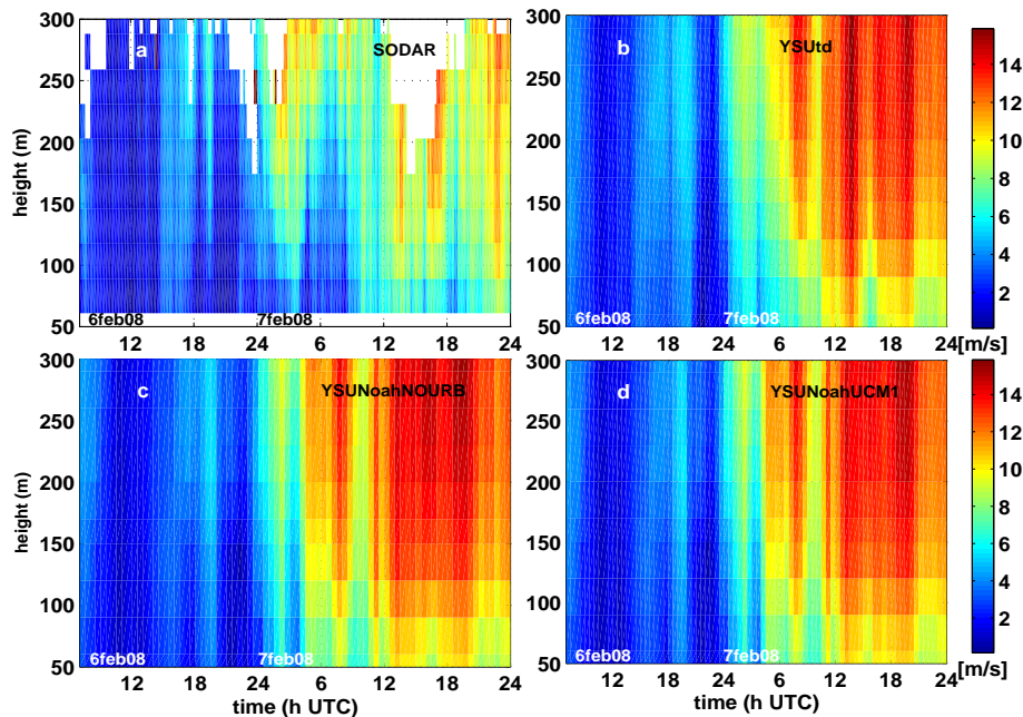
Fig. 10. Time series of the horizontal wind speed vertical profile on 6–7 February 2008 for (a) SODAR measurements, (b) YSUtd, (c) YSUNoahNOURB, (d) YSUNoahUCM1. Time is on x axis and height on ordinate axis.
