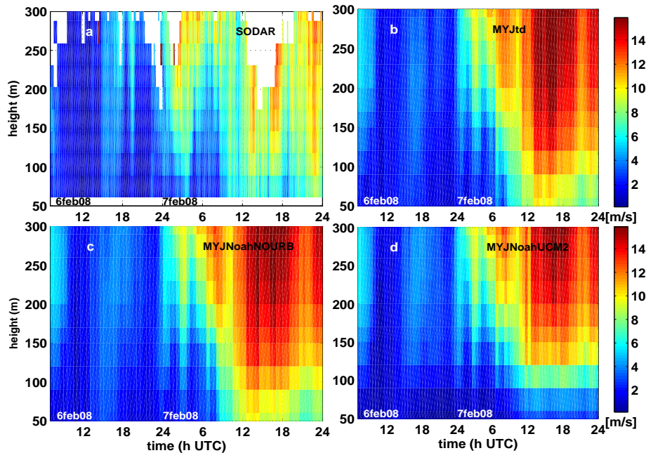
Fig. 11. Time series of the horizontal wind speed vertical profile on 6–7 February 2008 for (a) SODAR measurements, (b) MYJtd, (c) MYJNoahNOURB, (d) MYJNoahUCM2. Time is on x axis and height on ordinate axis.
