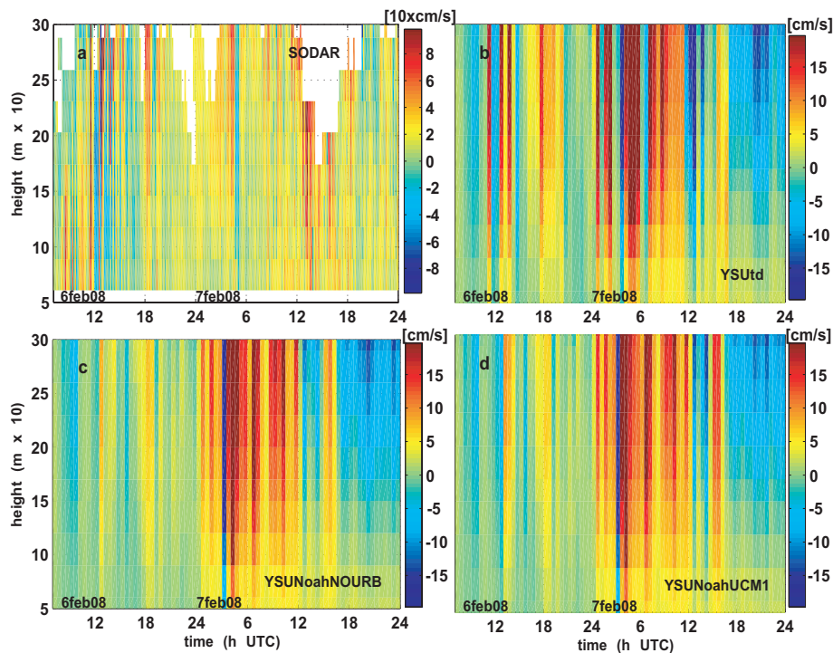
Fig. 12. Time series of the vertical wind speed vertical profile on 6–7 February 2008 for (a) SODAR measurements, (b) YSUtd, (c) YSUNoahNOURB, (d) YSUNoahUCM1. Time is on x-axis and height on ordinate axis.
