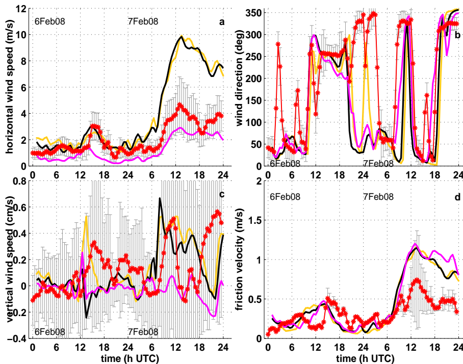
Fig. 7. Time series of horizontal wind speed ( a ), and direction ( b ), vertical wind ( c ), friction velocity ( d ) for 6–7 February 2008. Colours code is: MYJtd (orange); MYJNoahNOURB (black); MYJNoahUCM2 (pink); anemometer (red).
