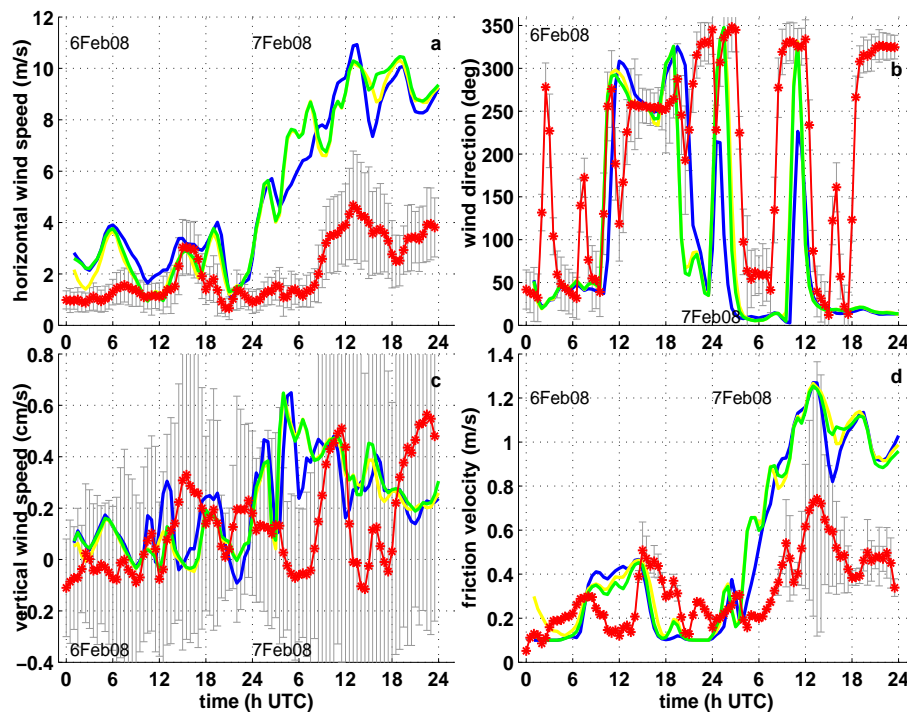
Fig. 5. Time series of horizontal wind speed ( a ), and direction ( b ), vertical wind ( c ), friction velocity ( d ) for 6–7 February 2008. Colours code is: YSUtd (blue); YSUNoahNOURB (yellow); YSUNoahUCM1 (green); anemometer measurements (red) and errors (grey).
