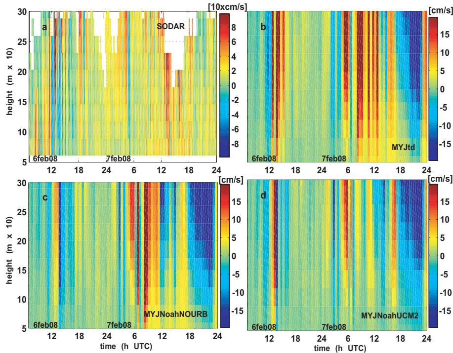
Fig. 13. Time series of the vertical wind speed vertical profile on 6–7 February 2008 for (a) SODAR measurements, (b) MYJtd, (c) MYJNoahNOURB, (d) MYJNoahUCM2. Time is on x-axis and height on ordinate axis.
