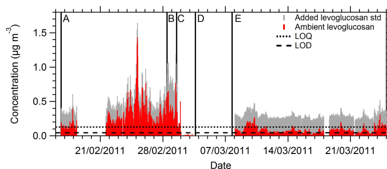
Fig. 3. Ambient levoglucosan concentrations during the campaign and the changes in the analytical conditions. The concentrations of ISTD and standard addition, respectively ( \text{ng mL}^{-1} ): (A) 50 and 50, (B) 50 and 100, (C) 50 and 0, (D) 100 and 0, (E) 100 and 50.
