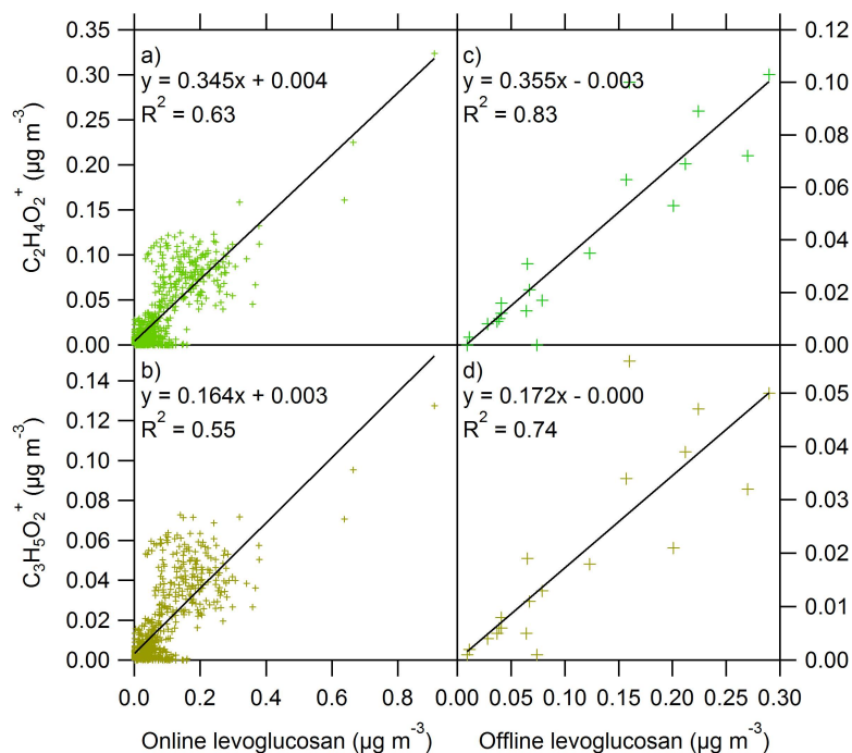
Fig. 7. Comparison of levoglucosan concentrations measured online with the PILS-HPAEC-MS and the biomass burning tracer concentrations measured with the HR-ToF-AMS (the data were averaged with 1 h time resolution) (a-b); and the comparison of levoglucosan concentrations determined offline from the filter samples with the HPAEC-MS and the biomass burning tracer concentrations measured with the HR-ToF-AMS (the HR-ToF-AMS data were averaged according to the filter sampling times) (c-d).
