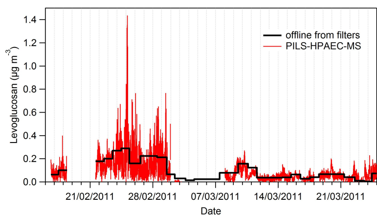
Fig. 4. Time series of levoglucosan measured online with the PILS-HPAEC-MS and determined offline from the filter samples with the HPAEC-MS. The PILS-HPAEC-MS measured with a time resolution of 8 min whereas the sampling duration for the filters varied from 18 to 72 h.
