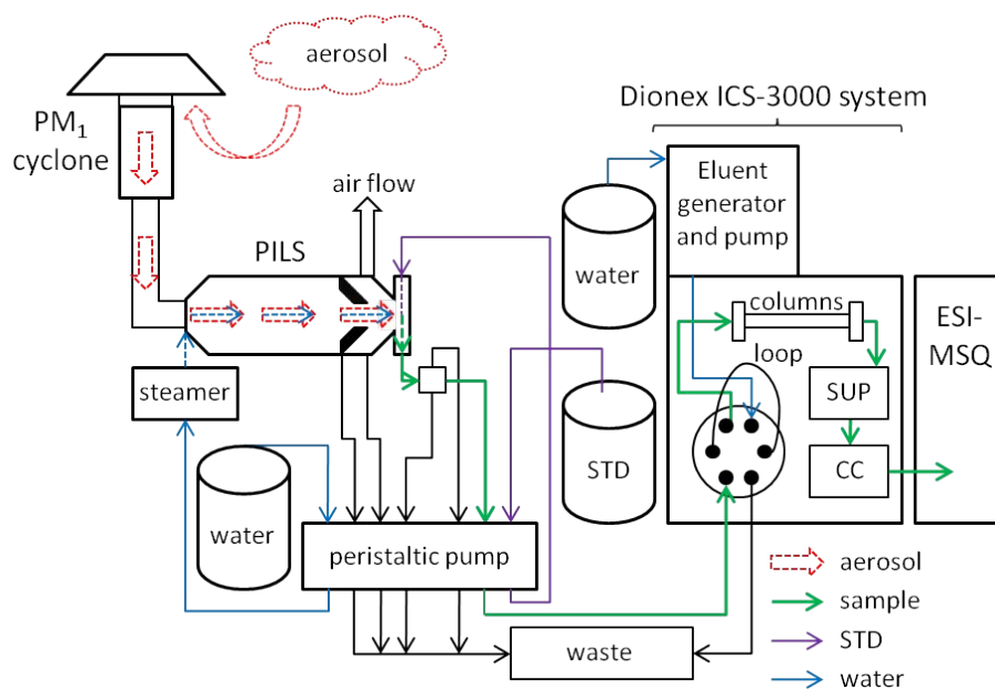
Fig. 1. Schematic representation of the sampling line and the online coupled PILS-HPAEC-MS apparatus. Arrows represent the flow of the aerosol sample and the liquids within the system. STD = standard solution containing internal standard and standard addition of levoglucosan; SUP = suppressor; CC = conductivity cell; ESI-MSQ = quadrupole mass spectrometer with electrospray ionization. The figure is not to scale.
