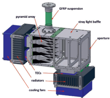
Fig. 3. Design of a GLORIA BlackBody (a) and configuration of the complete GLORIA in-flight blackbody calibration system (b) .
