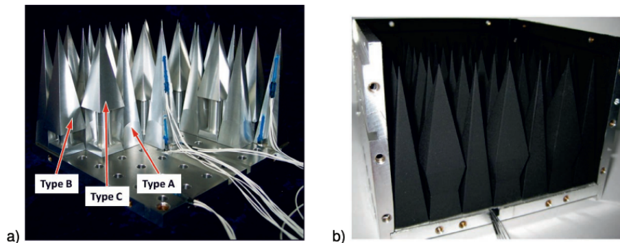
Fig. 4. Design of the optical surface: array of 49 individual pyramids (a) varnished with NEXTEL-Velvet Coating (b) .
