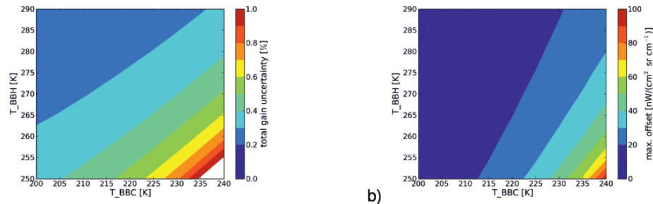
Fig. 9. Radiance uncertainty as a function of GBB-C and GBB-H temperatures: (a) total gain uncertainty and (b) maximum offset uncertainty.
