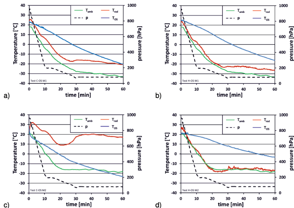
Fig. 13. Thermal behaviour during ascent simulation test. Upper panel: Scenario No. 1 (cold instrument compartment, final T_{amb} = -33^\circ\text{C} ) of (a) GBB-C optical surface with TEC power < 50W and (b) GBB-H optical surface with TEC power < 25W. Lower panel: Scenario No. 2 (warm instrument compartment, final T_{amb} = -18^\circ\text{C} ) of (c) GBB-C optical surface with TEC power < 120W and (d) GBB-H optical surface with TEC power = 0W.
