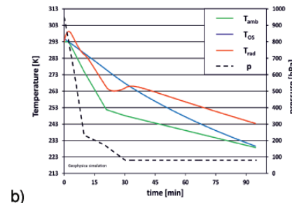
Fig. 8. Model simulation for the thermal behaviour during ascent: (a) the GBB prototype with a constant electrical current of 3 A and (b) optimal cooling of GBB-C optical surface during a Geophysica ascent (calculated for I_{TEC} = 1.5 A).
