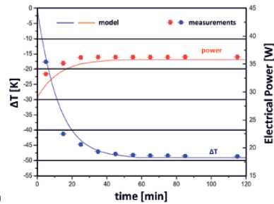
Fig. 8. Model simulation for the thermal behaviour during ascent: (a) the GBB prototype with a constant electrical current of 3 A and (b) optimal cooling of GBB-C optical surface during a Geophysica ascent (calculated for I_{TEC} = 1.5 A).
