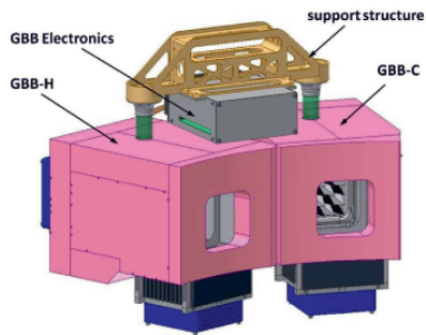
Fig. 3. Design of a GLORIA BlackBody (a) and configuration of the complete GLORIA in-flight blackbody calibration system (b) .
