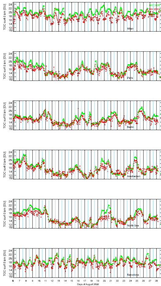
Fig. 6. Same as Fig. 5 but for surface –3 km TOC.
