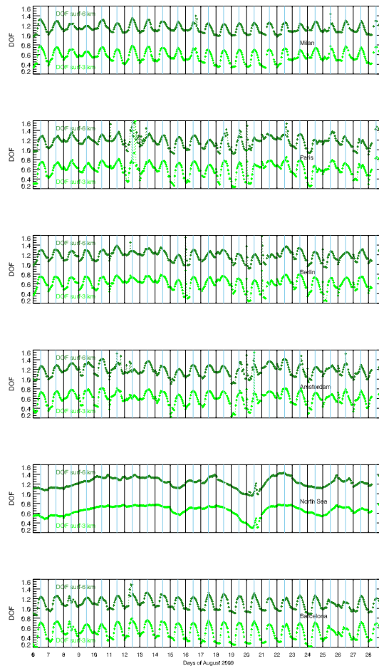
Fig. 7. Time series of the DOF surface –6 km (dark green) and surface –3 km (light green) over Milan, Paris, Berlin, Amsterdam, the marine location West of Norway coast, Barcelona.
