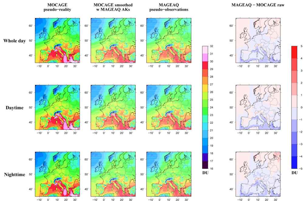
Fig. 3. Average surface –6 km TOC for 5–28 August 2009. From left to right: raw and AK -smoothed MOCAGE pseudo-reality, MAGEAQ-TIR pseudo-observations, differences of MAGEAQ-TIR pseudo-observations with respect to raw MOCAGE pseudo-reality. The average TOC are reported for the whole day (top row), daytime (central row) and nighttime acquisitions (bottom row).
