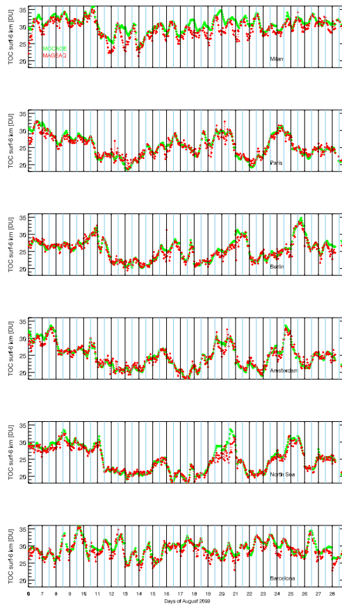
Fig. 5. Time series of MOCAGE surface –6 km TOC pseudo-reality (green), and MAGEAQ-TIR surface –6 km TOC pseudo-observations (red) over Milan, Paris, Berlin, Amsterdam, the marine location West of Norway coast, Barcelona.
