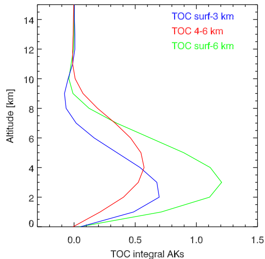
Fig. 2. Mean integral averaging kernel functions for the surface –3 km (blue), 4–6 km (red) and surface –6 km (green) TOCs, for all pixels in the dataset having thermal contrast between 0 and 1.0 K.
