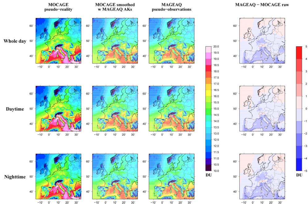
Fig. 4. Same as Fig. 3 but for surface –3 km TOC.
