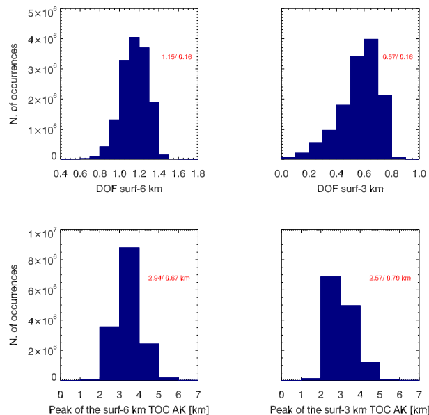
Fig. 1. Histograms of the DOF surface –6 km (top left), the DOF surface –3 km (top right), the altitudes of the maximum of the integrated AK for the surface –6 km TOC (bottom left), and the altitudes of the maximum of the integrated AK for the surface –3 km TOC (bottom right), for MAGEAQ-TIR. Mean values and standard deviations are also reported in red (mean/std). The data cover the whole period of study, on a 1 h revisit time basis.
