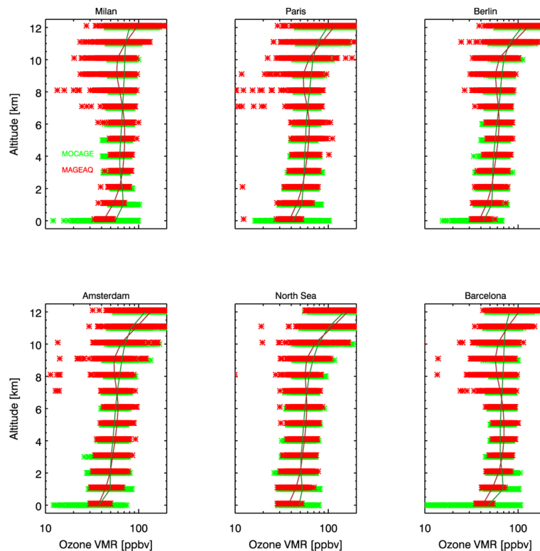
Fig. 8. Tropospheric ozone concentration profiles values for all pixels: MOCAGE pseudo-reality (green) and MAGEAQ-TIR pseudo-observation (red), at Milan (Italy), Paris (France), Berlin (Germany), Amsterdam (the Netherlands), one marine location West of Norway coast ( 55^{\circ} N/ 8^{\circ} E), Barcelona (Spain). The mean tropospheric ozone concentration profiles for both MOCAGE (green) and MAGEAQ-TIR (red) are also shown.
