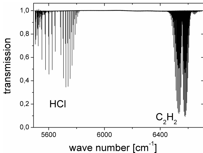
Fig. 3. Transmission spectrum recorded with the C_2H_2 and a TCCON HCl cell in the beam. The band to the right is due to absorption by C_2H_2 , the band to the left is due to HCl absorption. Some H_2O signatures emerging in the lab air path can be detected at wave numbers below 5550\text{ cm}^{-1} .
