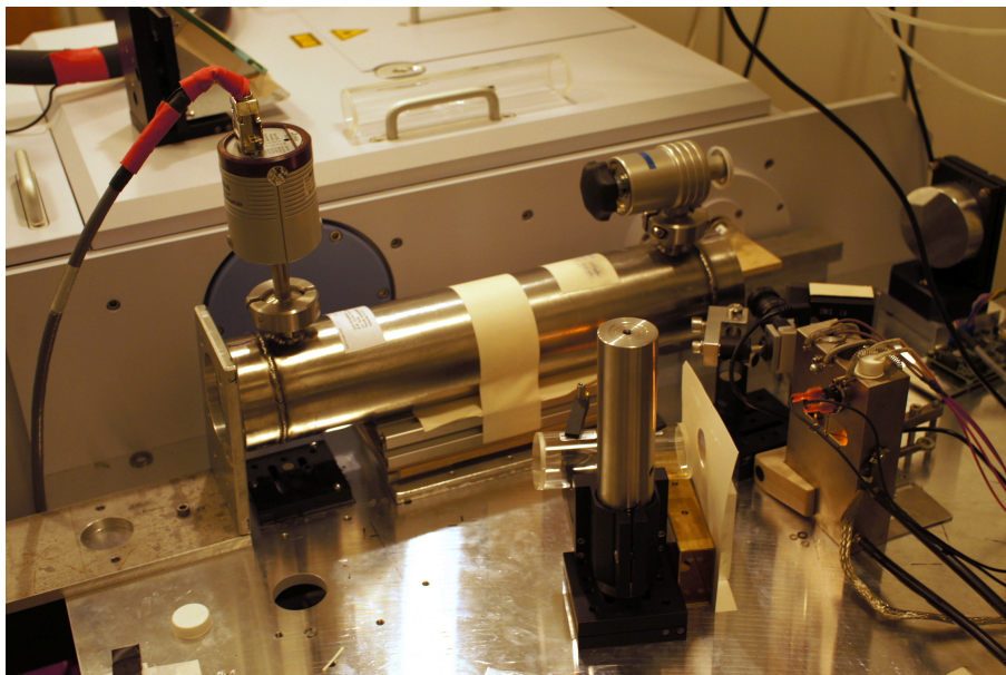
Fig. 2. Setup for HCl cell calibration at the TCCON site Karlsruhe. The source is on the right side in front, left from the source an HCl cell under test is located (protected by a heat shield to limit heating of the cell by the thermal radiation emitted by the source). The first mirror is on the left outside the figure. The long steel cylinder is the pressure monitored C_2H_2 cell, the two mirrors in the rear right corner of the image steer the radiation into the spectrometer.
