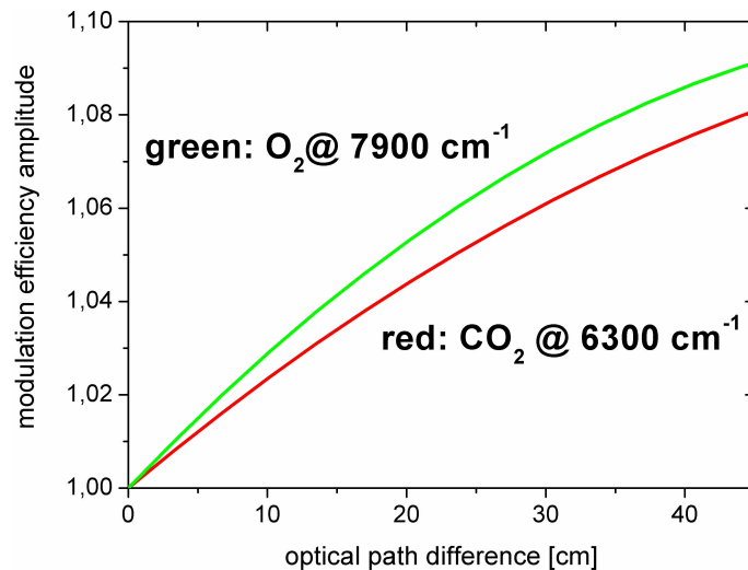
Fig. 1. Disturbance of ME amplitude assumed for characterisation of TCCON XCO 2 product sensitivity with respect to ILS uncertainty.
