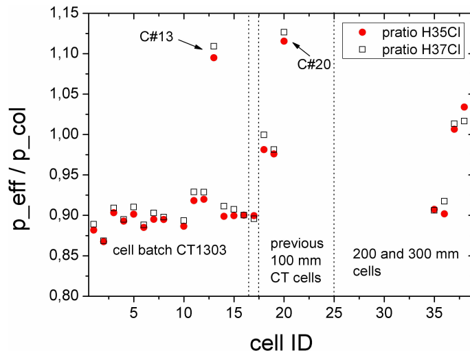
Fig. 8. The effective pressure values ratioed over pressure derived from observed column for the calibrated cells listed in Table 1. The dashed vertical lines separate different batches or different cell dimensions.
