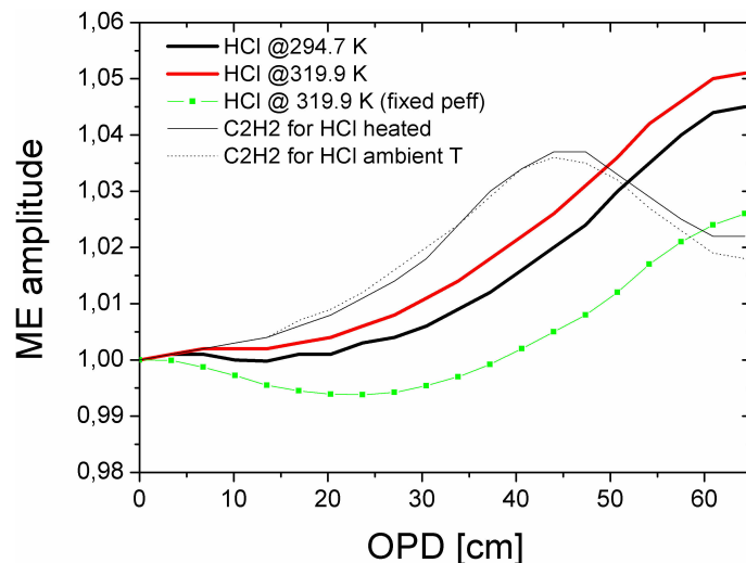
Fig. 7. ME amplitudes retrieved from HCl cell #2 at ambient temperature and heated to about 320 K. The derived ME amplitudes are in good agreement under the assumption that the effective pressure values are proportional to absolute temperature. The ME amplitudes derived from C_2H_2 are also shown and prove that the alignment status of the spectrometer did not change. The dash-dotted green line would result if the effective pressure parameters are kept to their values at 294.7 K in the ILS analysis instead of converting them to the actual temperature.
