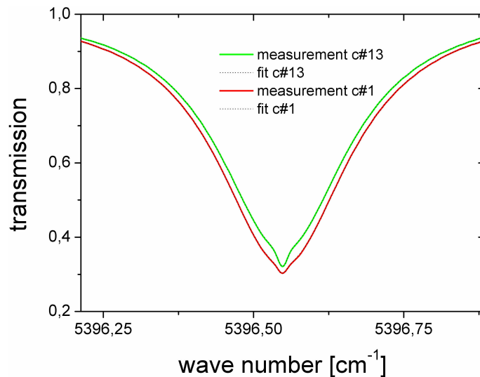
Fig. 9. A \text{H}_2\text{O} line as observed in a calibration measurement. The narrow dip appended to the line center is due to absorption at low pressure, while the strong underlying absorption is generated in the lab air path. The superimposed dashed lines are synthetic spectra generated with LINEFIT.
