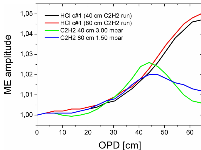
Fig. 4. ME amplitudes retrieved from a 40 cm cell filled with 3.00 mbar of C_2H_2 and two 40 cm cells in a row, each filled with 1.50 mbar of C_2H_2 . For comparison, the ME amplitudes derived from an HCl cell (same cell was used for both measurements, effective cell parameters applied for ILS retrieval) is shown. The HCl results prove that the alignment status of the spectrometer did not change between the two measurements.
