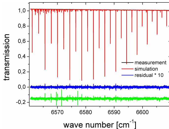
Fig. 5. Typical fit quality achieved for an ILS retrieval using C_2H_2 as described in Sect. 4. The green residual (vertically shifted for clarity) refers to a use of the original HITRAN 2008 line list.
