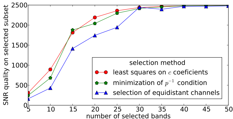
Fig. 9. Results of the mean reconstruction SNR for the three discussed spectral subset selection techniques.
