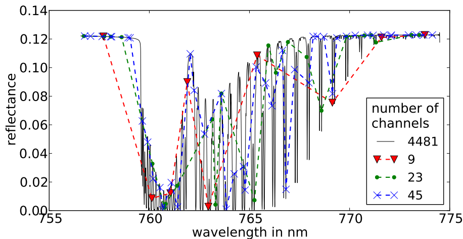
Fig. 7. Similar to Fig. 5, but the position of the spectral channels were chosen with the optimization technique based on the minimization of \mathbf{C} matrix residuals.
