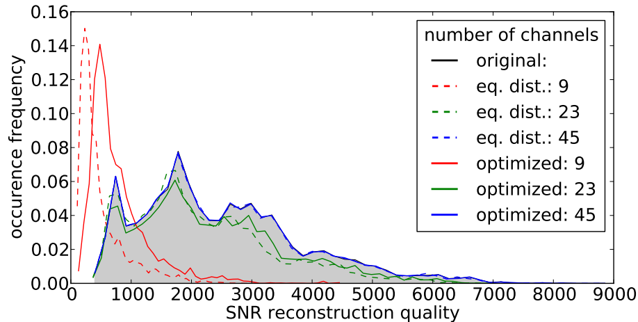
Fig. 12. The grey area shows the reconstruction SNR histograms for the original, i.e. using the full spectral information, reconstruction and two of the discussed reconstruction techniques using small spectral sub samples. The dashed lines show result for the equal sampling technique while the lines show results for the selection based on the minimization of \mathbf{C} matrix residuals. The colors indicate the different size of the spectral sub samples.
