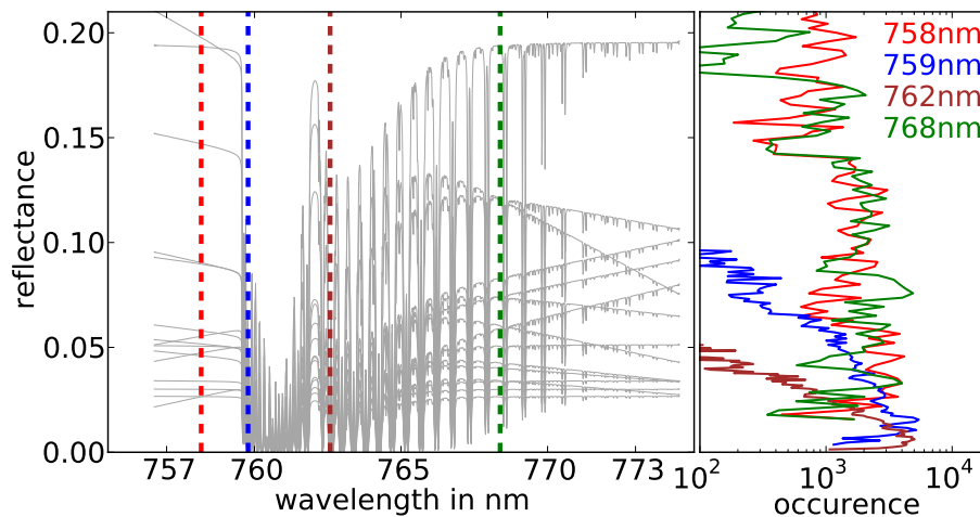
Fig. 1. The left panel illustrates the variability of the used spectral data base with showing some randomly selected spectra. The right panel shares the reflectance axis with the left panel and shows logarithmic histograms for four selected wavelengths.
