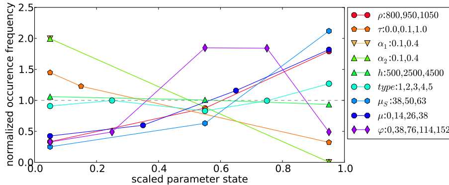
Fig. 4. Normalized histograms for parameter state occurrence in the lowest 10 % fraction of a reconstruction SNR data set based on 500 samples. The occurring states are scaled to a range of [0, 1] such that they can be shown on the same axes. The corresponding values are shown in the legend. The occurrences are normalized by the sample size and multiplied by the number of unique parameter values (e.g. three for surface pressure and five for the aerosol type). A value of one indicates equal representation of this particular parameter value within the data set while larger and smaller values represent over- and under-representation.
