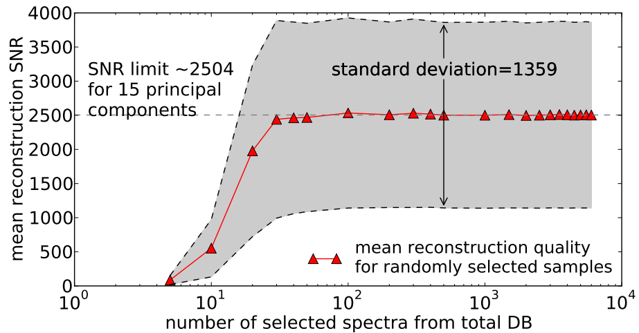
Fig. 2. Reconstruction SNR for a lookup table of top of atmosphere radiances in the oxygen A Band (see Table 1 and Fig. 5 for reference). The reconstruction SNR was defined as the ratio of the standard deviation of the residual and the mean value of the truth where the residual was defined as the difference between truth and reconstruction. The considered index set was randomly chosen and for each step, computations were repeated 50 times and the mean value is shown. Shown is the mean reconstruction SNR which is the mean value over the reconstruction SNR for all cases in the lookup table. The grey shaded area shows the corresponding standard deviation. A histogram for the whole dataset is shown in Fig. 3.
