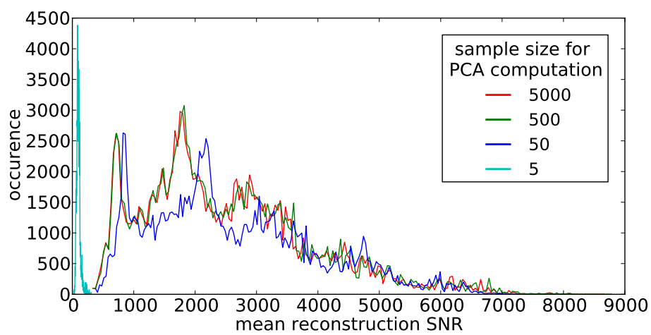
Fig. 3. Histograms of the reconstruction SNR for various sample sizes.
