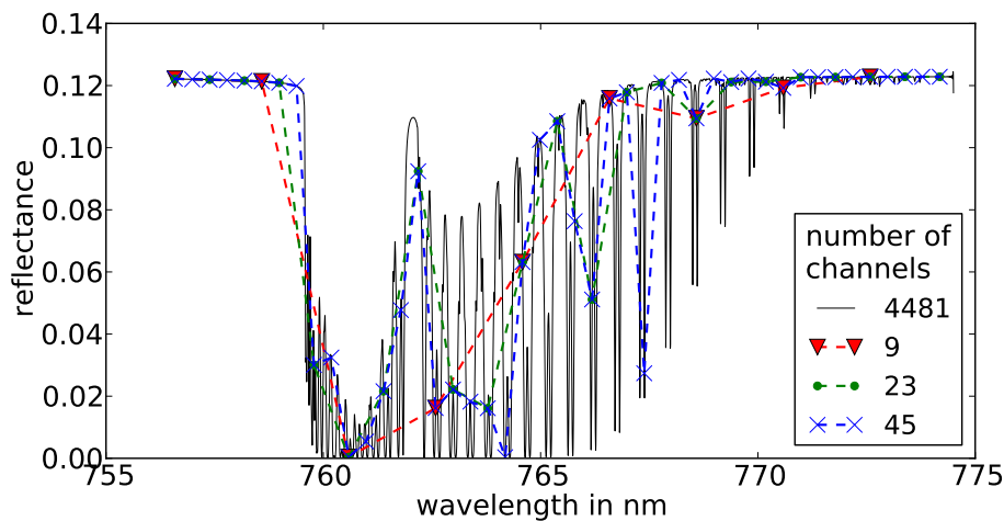
Fig. 5. The grey line shows an example spectrum from the lookup table. The red, green and blue lines are the result if only every 500th, 200th, or 100th channel of the original spectrum is considered.
