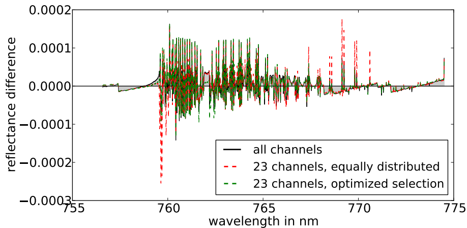
Fig. 11. Similar to Fig. 10, but 23 spectral bands were used.
