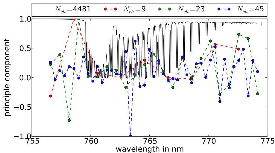
Fig. 6. The grey line shows the first principal component for the complete spectral resolution ( \mathbf{P}_{0,-} ) while the colored lines show the corresponding rows for \bar{\mathbf{P}} for three sample sizes. The equal distribution sampling technique was used.
