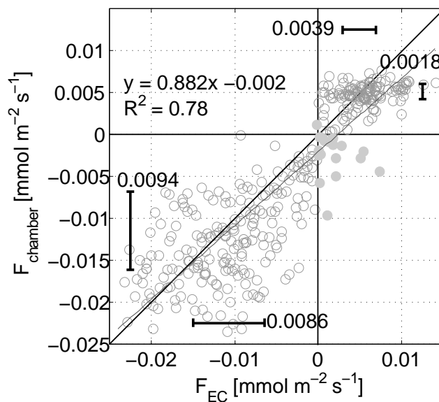
Fig. 1. Scatter plot of EC- and chamber-determined NEE, light grey filled circles represent \text{CO}_2 fluxes with opposite directions, black bars show interquartile ranges of EC-/chamber \text{CO}_2 source and sink fluxes, respectively (opposite \text{CO}_2 fluxes excluded).
