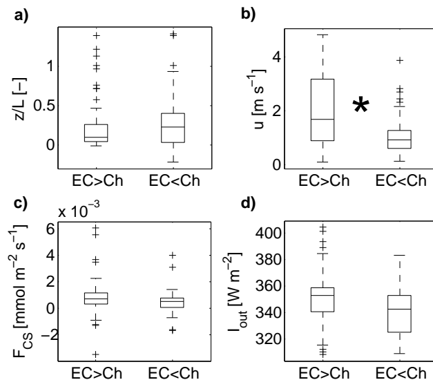
Fig. 4. Comparison of (a) nighttime atmospheric stability ( z/L ), (b) wind velocity ( u ), (c) \text{CO}_2 flux by coherent structures ( F_{CS} ) and (d) long wave outgoing radiation ( I_{out} ) while either EC or chamber \text{CO}_2 fluxes are larger, highly significant difference (Student's t test for dependent samples, * = p < 0.01 ) found only in case of u (as well as u_* ).
