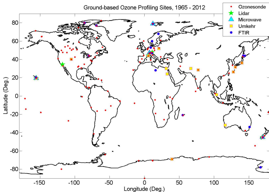
Fig. 1. World map with locations for the long-term ground-based measurement sites: ozone sounding sites (red dots), lidar sites (green stars), microwave sites (light blue triangles), Dobson/Brewer sites with Umkehr measurements (yellow squares), and FTIR sites (dark blue circles).
