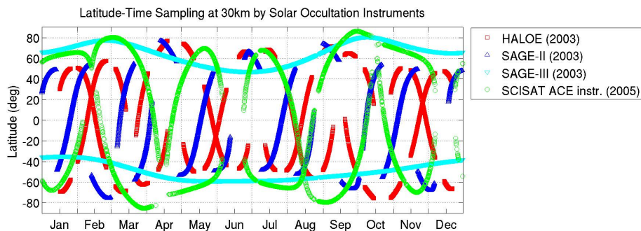
Fig. 4. Latitudinal coverage for the solar-occultation instruments (example years: 2003 and 2005). SAGE I is similar to SAGE II (blue triangles), POAM and ILAS instruments are similar to SAGE III (turquoise triangles).
