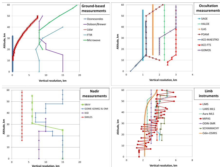
Fig. 3. Vertical resolution shown as function of altitude for each of the described instruments systems: (a) ground-based instruments, (b) solar/stellar occultation instruments, (c) nadir measuring instruments, and (d) limb measuring instruments.
