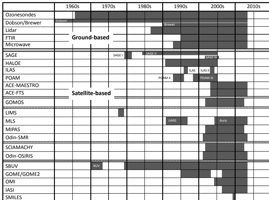
Fig. 2. Temporal coverage of the described ground- and satellite-based measurement systems.
