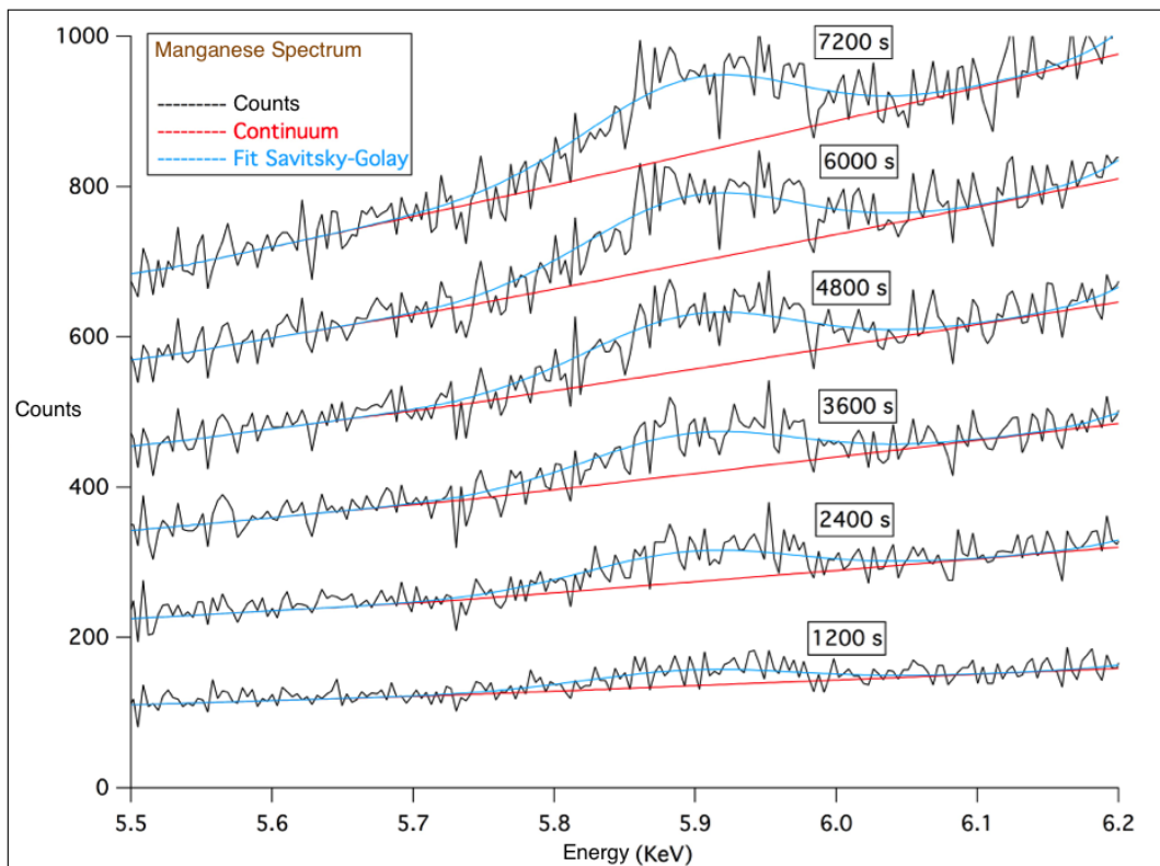
Fig. 1. Study of the peak of Manganese (1)
