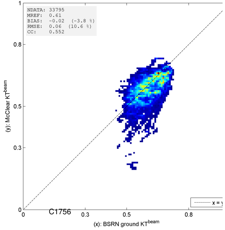
Clear sky Beam Clearness Index ( KT^{beam} ) (2005-2007) [N39.754, E116.962, alt.
