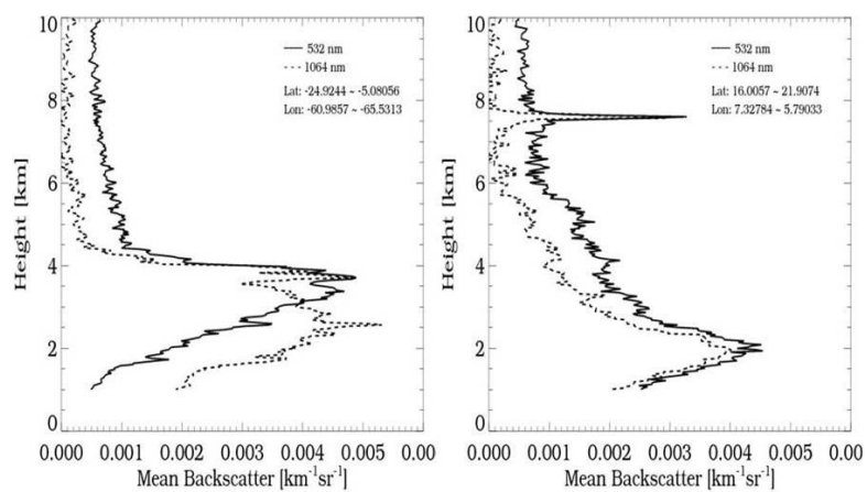
Fig. 4. CALIOP-measured attenuated backscatter profiles at 532 nm (solid line) at 1064 nm (dotted line) over Amazonia (left) and Saharan Desert (right).
