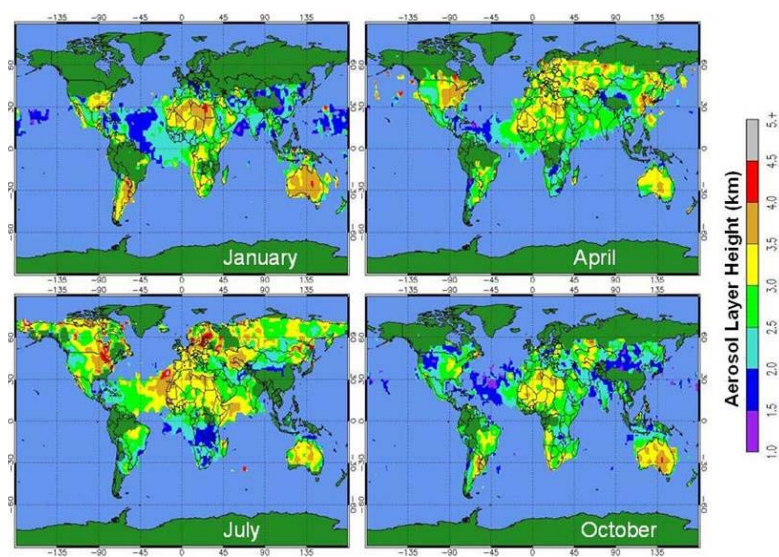
Fig. 6. Monthly average aerosol layer height.
