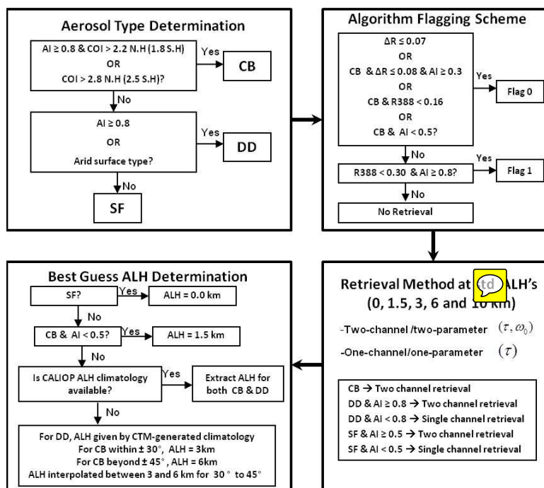
Fig. 1. Graphic description of OMAERUV inversion scheme
