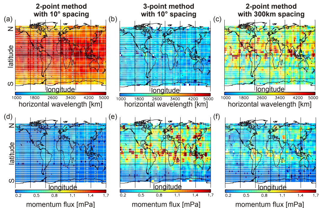
Fig. 1. Projected horizontal wavelength (a and c) and true horizontal wavelength (b) with spacings of 10° (a and b) and <300 km (c) and the corresponding momentum flux d-f.
