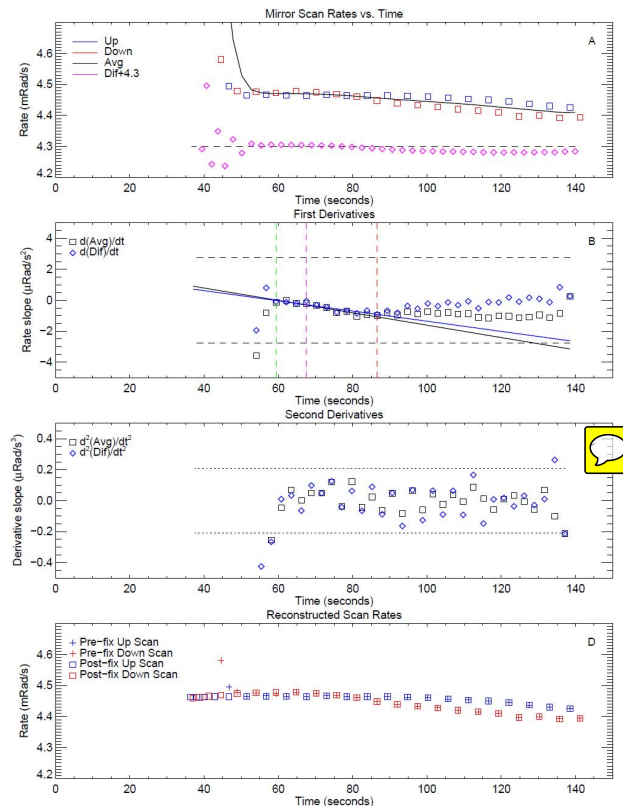
Fig. 13. Scan-mirror rate data for a sunrise event. Fits to the first derivatives of the average scan rate and difference between up and down scan rates are used to reconstruct scan rate data at low altitudes where scan rate data have gone bad. Only the scans just above where rate data go bad are used (between the green and red dashed lines in plot B ). To avoid any programmatic errors with using the second derivative data to determine where rates have gone bad, a limiting altitude of 60 km is used (dashed purple line). The comparison between original and reconstructed scan rates is shown in plot (D) .
