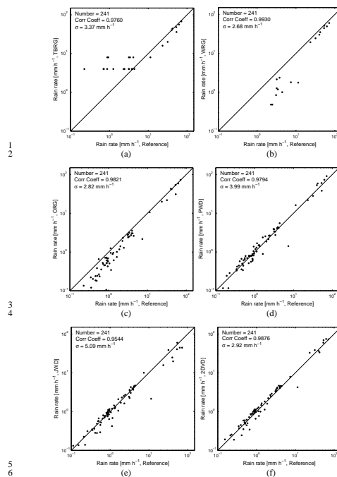
Figure 2. Comparison of individual instruments against the reference rain rate averaged over 3 minutes (January 13 th 2012)
