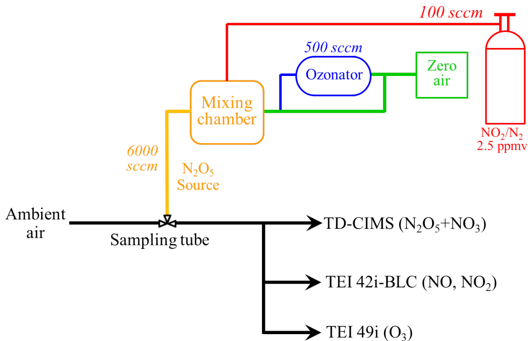
Fig. 2. Schematic diagram for \text{N}_2\text{O}_5 calibration using the on-line synthesis method.
