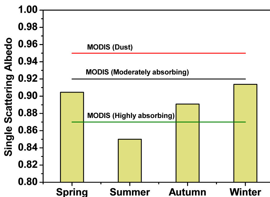
Fig. 1. Seasonal mean single scattering albedo observed over Gadanki at 500 nm along with SSA values being used in MODIS algorithm at 550 nm.
