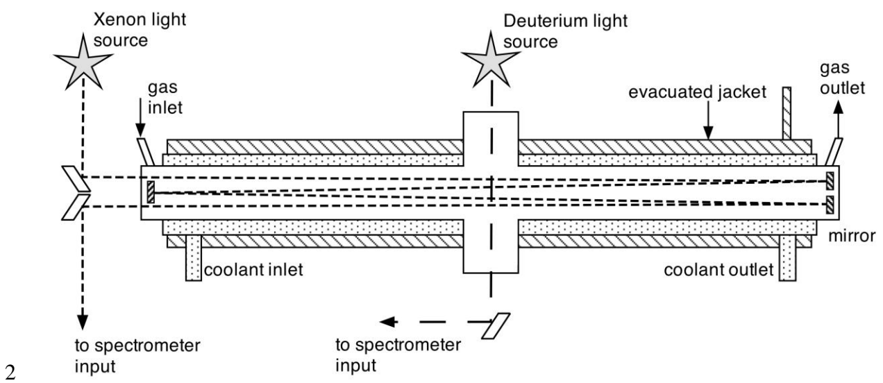
3 Figure 1. Experimental setups. Upper panel: absorption cell coupled to the FTS. Lower panel: 4 White absorption cell coupled to the echelle spectrometer. The shortest path length was 5 achieved using the cross path.
