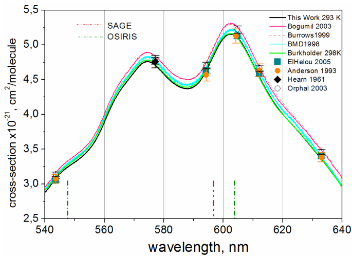
3 Figure 7. Ozone absorption cross-sections in the Chappuis band: (a) near absorption minimum 4 at 380 nm, (b) at the maximum of the Chappuis band. Notations for datasets and spectral 5 channels are the same as in Fig. 3, green solid line – Burkholder and Talukdar (1994).
