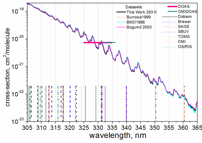
3 Figure 4. Ozone absorption cross-section at room temperature in (a) Hartley band and (b) 4 Huggins band. Notations for datasets and spectral channels are the same as in Fig. 3. 5 Triangles are data from Petersen et al. (2012).
