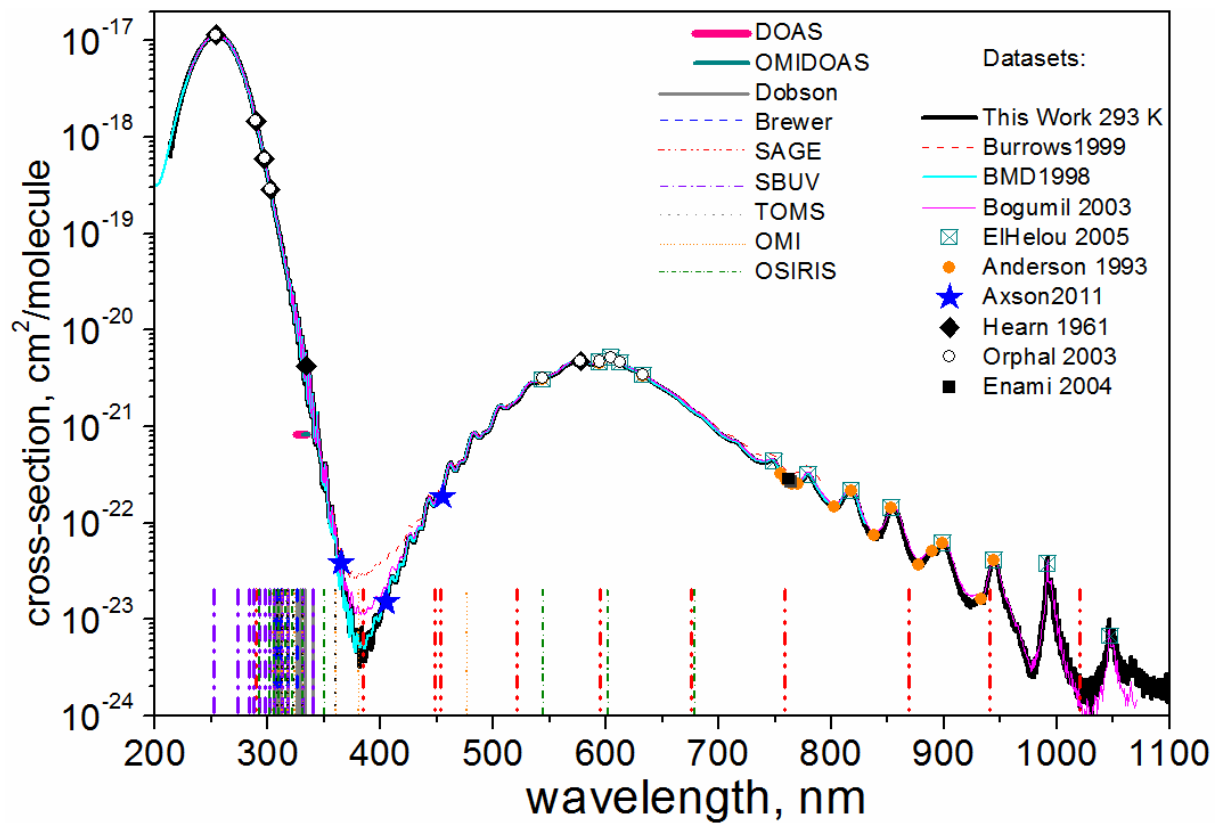
2 Figure 3. Ozone absorption cross-section at room temperature. Notations for datasets: black 3 solid line - this work, magenta solid line – Bogumil et al. (2003), light blue solid line - BMD, 4 dash line – Burrows et al. (1999); symbols: cross – El Helou et al. (2005), closed circle – 5 Anderson et al. (1993), star – Axson et al. (2011), open circle – Orphal (2003), diamond – 6 Hearn (1961), closed square – Enami et al. (2004); notations for instrument channels: solid 7 horizontal lines – DOAS and OMI-DOAS in Huggins band; vertical lines: grey solid – 8 Dobson, dash – Brewer, dash-dot-dot – SAGE, dash-dot – SBUV, dots – TOMS, short dots – 9 OMI, short dash-dots - OSIRIS.
