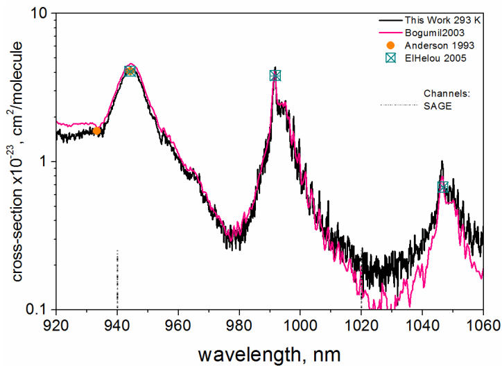
3 Figure 8. Ozone absorption cross-sections datasets in the Wulf band: (a) 750-900 nm, (b) 920- 4 1060 nm. Notations for datasets and spectral channels are the same as in Fig. 3.
