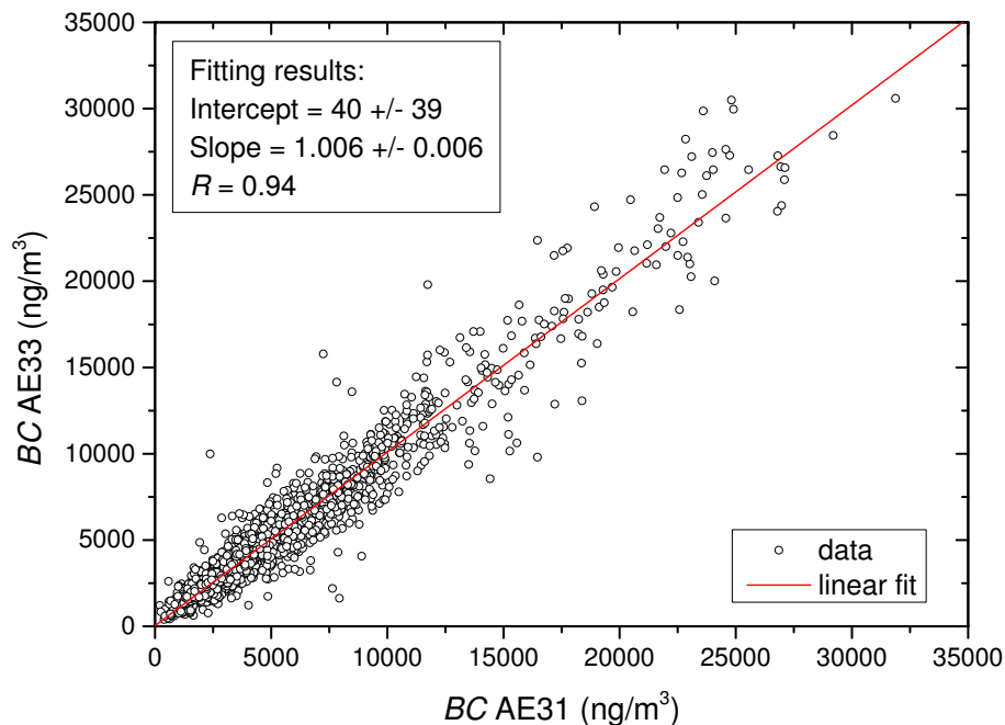
Figure 10. The correlation of BC measurements (2 weeks, Klagenfurt, Austria) between the Aethalometers AE31 (using quartz filter) and AE33 (using TFE coated glass fiber filter), showing 5 min averages of data compensated for the loading effect.
