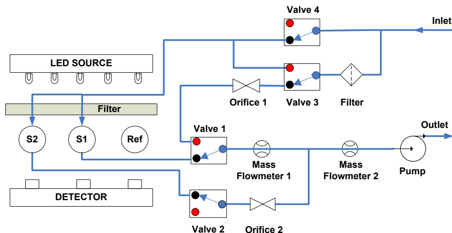
Figure 1. The AE33 flow diagram. During measurement, the inlet air passes through filter spots S1 and S2, each with a different flow rate, as set by the orifice 2. Air flow through S1 is measured by the mass flowmeter 1, flow through S2 is calculated as a difference between the total flow (flowmeter 2) and flow through S1. The valves are used for routing of air flow during different modes of operation.
