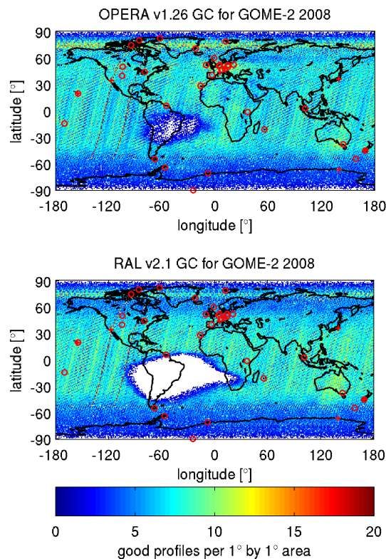
Figure 1. Spatial distribution of “good” (not screened) GOME-2 profiles (2008 only) in the OPERA v1.26 and RAL v2.1 global coverage (GC) datasets. Contributing ozonesonde and lidar stations are indicated by red circles and crosses, respectively.
