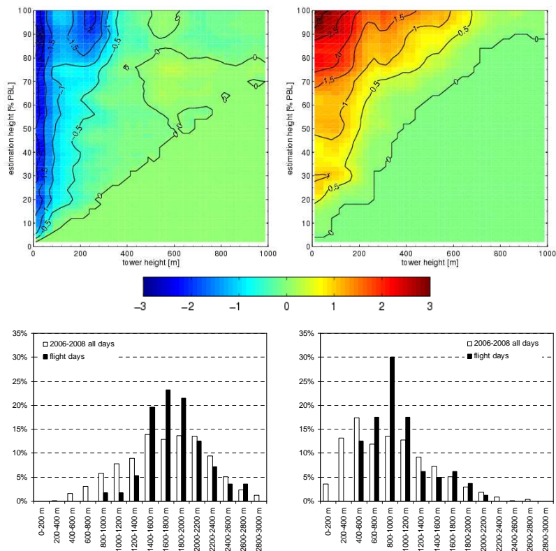
Figure 1. The median bias between the true CO 2 mole fraction and the estimated one as a function of the height of the hypothetical tower (tower height) and the relative height within the PBL for which the mole fraction is extrapolated (“estimation height”) from the measurements at the top of the tower ( \mu\text{mol mol}^{-1} ). Negative sign means underestimation by the measurements. Left: summer; right: winter. Bottom panels show the 12:00 UTC PBL-height statistics for all days during the period of 2006–2008 and for the days of the flights.
