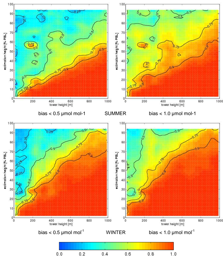
Figure 6. Empirical probability of the cases when the bias does not exceed 0.5 (left) or 1.0 μmol mol -1 (right) at the application of the VTT concept as the function of the height of the tower and the estimation height relative to the height of the PBL in summer (top) and winter (bottom).
