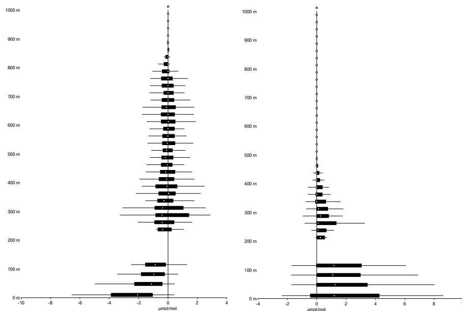
Figure 2. Empirical frequency distribution of the differences between the CO 2 mole fraction measured at a given height (tower height) and the mid-PBL CO 2 mole fraction determined from the aircraft vertical profiles for summer (left) and winter (right). Whiskers represent the lowest value still within 1.5 interquartile range (IQR) of the lower quartile and the highest value still within 1.5 IQR of the upper quartile, respectively.
