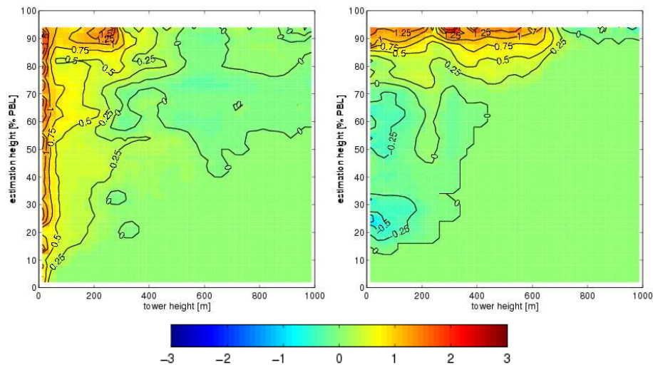
Figure 5. Difference of the median biases of the estimations applying and not applying the VTT concept ( \mu\text{mol mol}^{-1} ). Positive sign indicate that the application of the VTT concept improves the estimation. Left: summer; right: winter.
