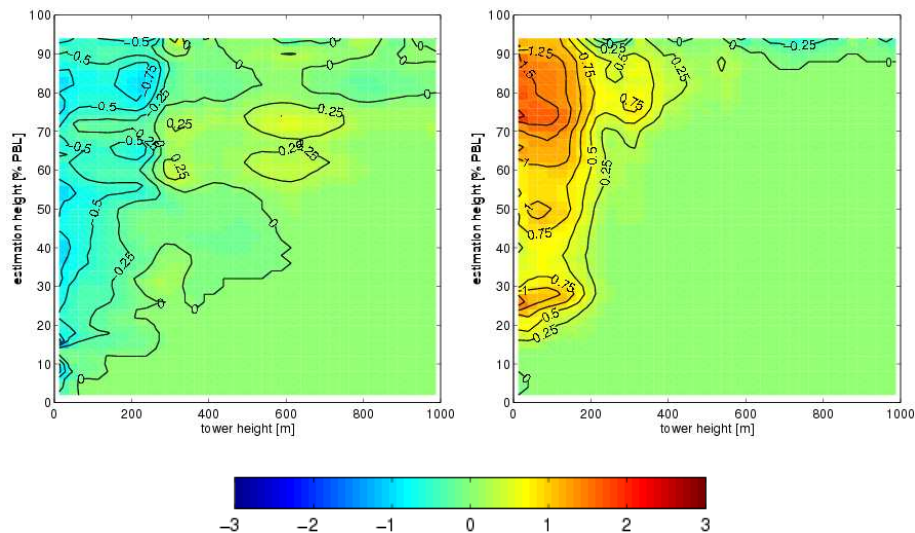
Figure 4. The median bias between the true CO 2 mole fraction and the estimated one using the VTT concept as a function of the height of the hypothetical tower (tower height) and the relative height within the PBL for which the mole fraction is extrapolated (“estimation height”) from the measurements at the top of the tower ( \mu\text{mol mol}^{-1} ). Negative sign means underestimation by the measurements. Left: summer; right: winter.
