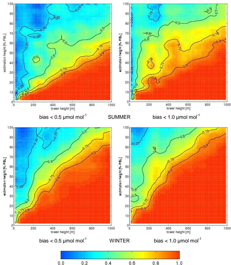
Figure 3. Empirical probability of the cases when the bias does not exceed 0.5 (left) or 1.0 \mu\text{mol mol}^{-1} (right) as the function of the height of the tower and the estimation height relative to the height of the PBL in summer (top) and winter (bottom).
