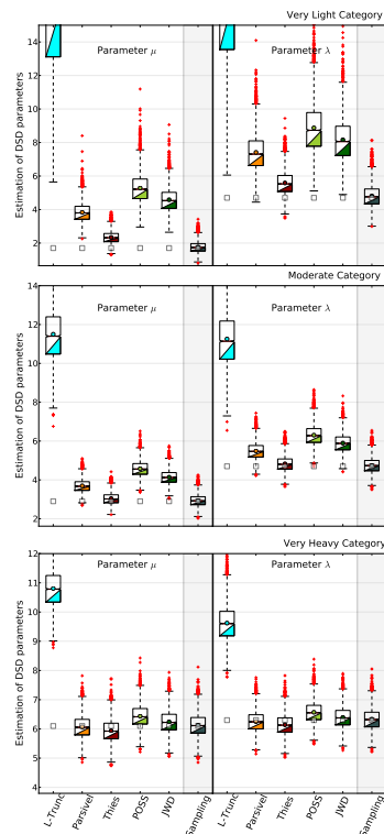
Fig. 6. The predictions are compared by means of the MLE method for several binning methods. The Left-Truncated and OSP provide results similar to those of MM012, thus the OSP is omitted in this figure. Additionally, the Left-Truncated is not entirely visualised to allow for a better visualisation of the detailed differences between the disdrometers shown here. Similarly, the 2DVD case is located between that of the Thies device and sampling, and it is omitted. The box-plots are based on 5000 samples.
