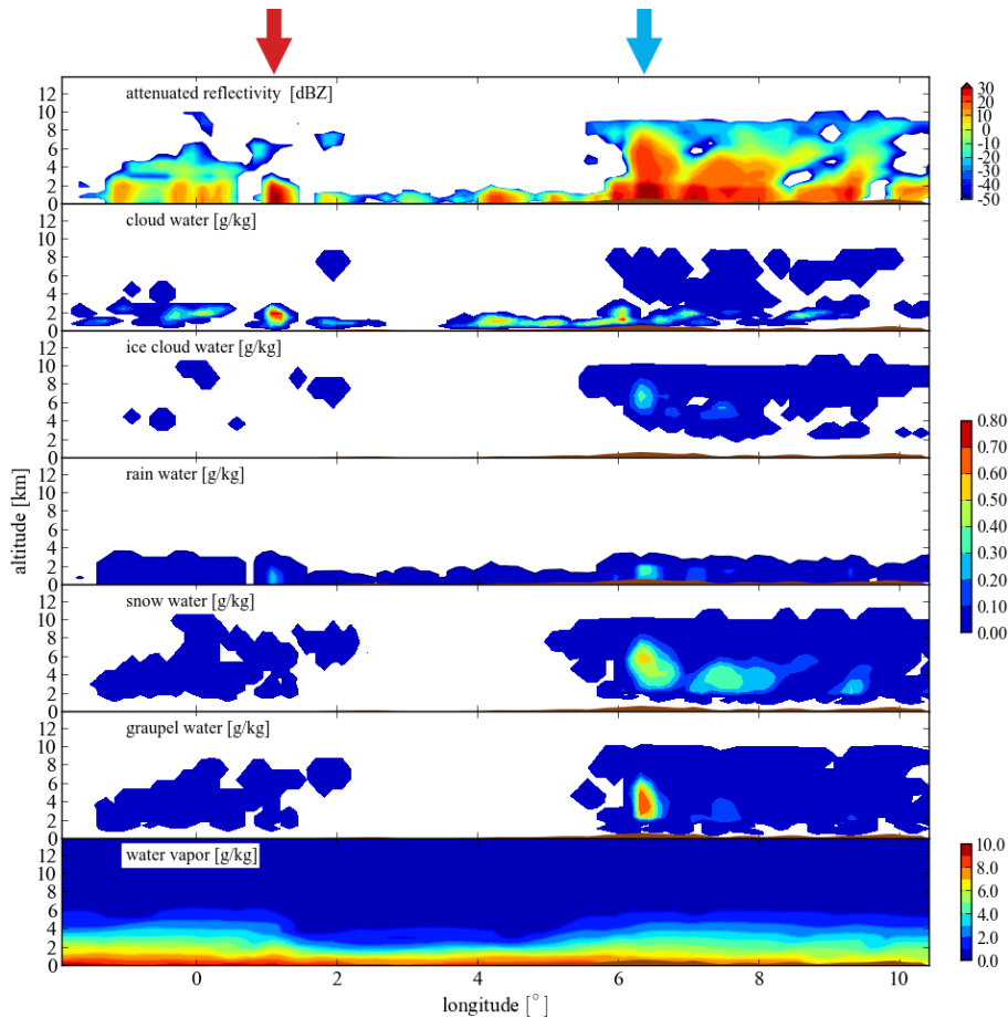
Fig. 6. Attenuated reflectivities (top) and hydrometeor and water vapor contents along the same cross section as in Figs. 4 and 5.
