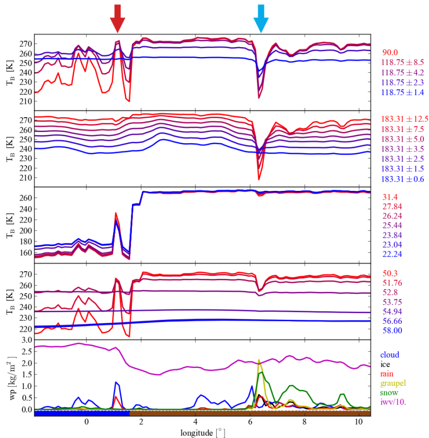
Fig. 5. Integrated hydrometeor contents (bottom row) and simulated brightness temperatures along a cross section from West to East through a long lasting precipitation event on 19 September 2001 at 18:00 UTC over Hoek van Holland (see Fig. 4). For detailed description see text.
