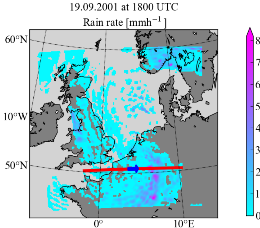
Fig. 4. Simulated rain rates in \text{mmh}^{-1} for the Hoek van Holland case on 19 September 2001 at 18:00 UTC. The red line and blue arrow indicate the artificial flight path show in Figs. 5 and 6.
