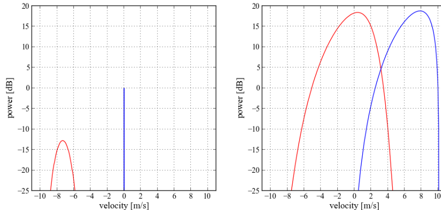
Fig. 2. Original (blue) and aircraft affected (red) Doppler spectra for monodisperse cloud (left) and typical rain particle distribution (right). Aircraft speed is 210 \text{ m s}^{-1} and pitch angle 2^\circ . Marshall–Palmer size distribution with rain rate of 5 \text{ mm h}^{-1} is assumed.
