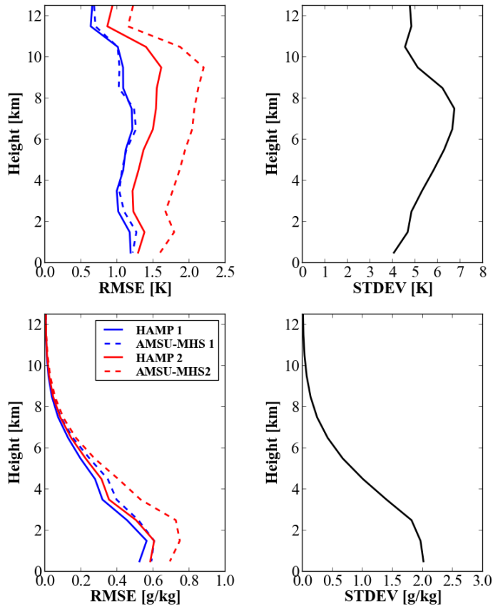
Fig. 7. Retrieval RMSE (left) and test data set standard deviation (right) for temperature [K] (top panel) and water vapor mixing ratio over ocean [ \text{g kg}^{-1} ] (bottom panels) for the HAMP (solid line) and AMSU-MHS (dashed line) instruments with two different assumptions on T_B uncertainty. See text for details.
