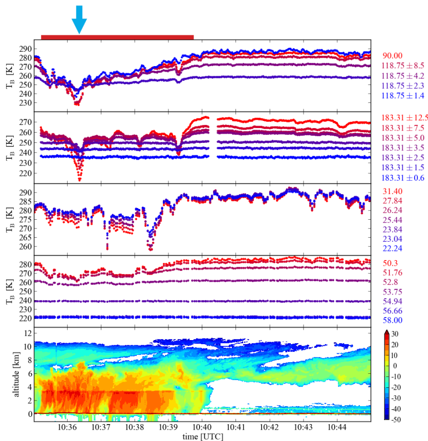
Fig. 8. Measurements taken by HAMP on 24 July 2013 over western Germany. Upper four panels show the measurements taken by the radiometer modules. Lower panel shows the reflectivities in dBZ captured by the MIRA-36 cloud radar.
