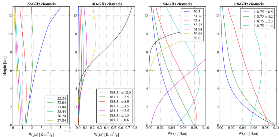
Fig. 3. HAMP clear air weighting functions (nadir downward-looking). Shown are the water vapor (two left most) and the temperature (two right most) weighting functions for a HALO ceiling height of about 13 km. The US 1976 Standard Atmosphere over a black surface was assumed for the calculations.
