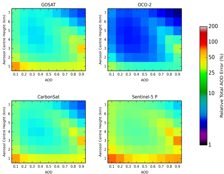
Figure 9. Relative AOD error as a function of aerosol centre height and AOD for the parameterized aerosol retrieval for a SZA of 30° and albedo of 0.5. Intensity offset is included.
