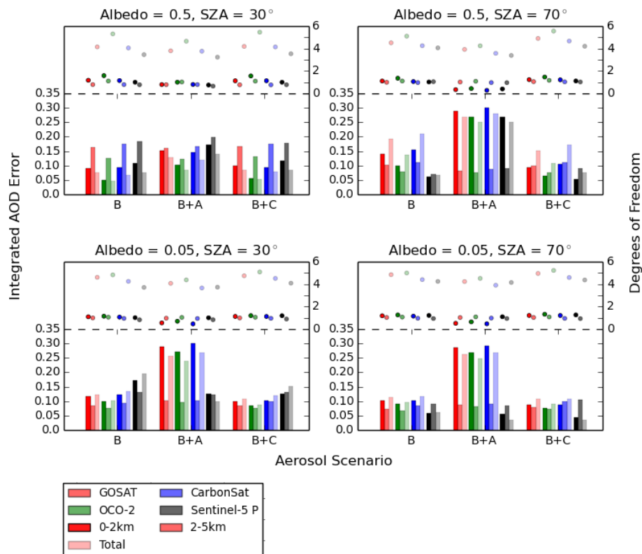
Figure 7. As Fig. 6 but for the aerosol scenario B and combined aerosol scenarios B + A and B + C. Note that scenario B + A is identical to A + B from Fig. 6.
