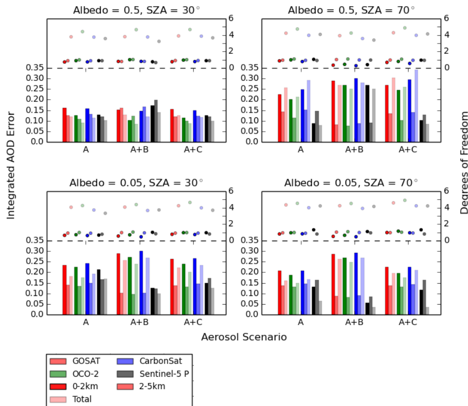
Figure 6. AOD error and DoF for the aerosol profile retrieval for surface albedos of 0.05 and 0.5 and SZAs of 30° and 70° for the four instruments when integrating over the 0–2 km and 2–5 km ranges as well as the total column for aerosol scenario A and combined aerosol scenarios A + B and A + C. Intensity offset is included.
