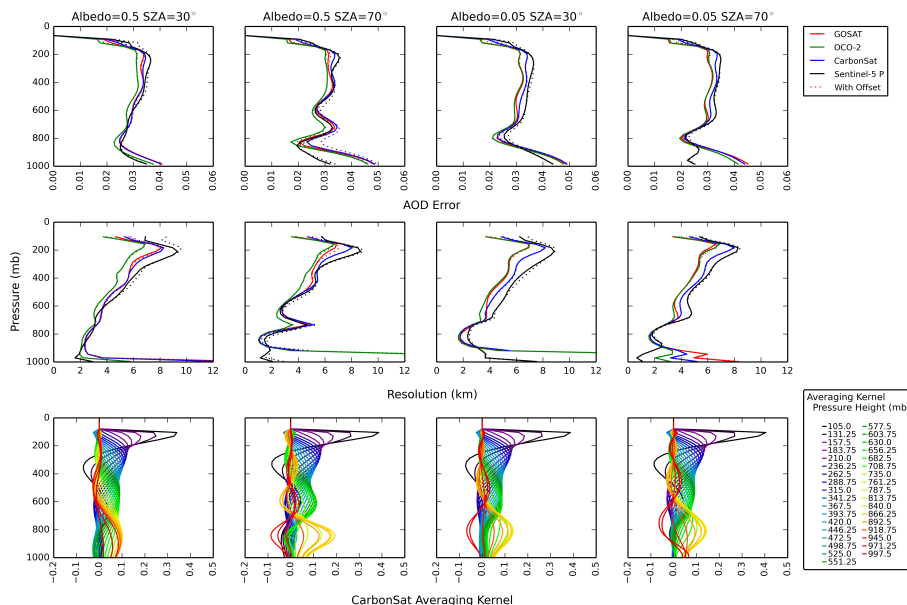
Figure 4. Error of LAOD (top panel) and vertical resolution (middle panel) as a function of pressure for the aerosol profile retrieval for scenario A for surface albedos of 0.05 and 0.5 and SZAs of 30° and 70° for the four instruments without an intensity offset. The results for a retrieval with intensity offset is shown by the dotted lines. The bottom panels show the averaging kernels for CarbonSat for the profile retrieval with intensity offset. Note that the top four pressure levels are not shown.
