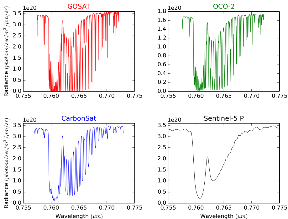
Figure 1. Simulated spectra for GOSAT, OCO-2, CarbonSat and S-5 P for a solar zenith angle of 30^\circ and a surface albedo of 0.5. An aerosol layer with optical depth of 0.3 at a height of 1 km with a width of 1 km is assumed.
