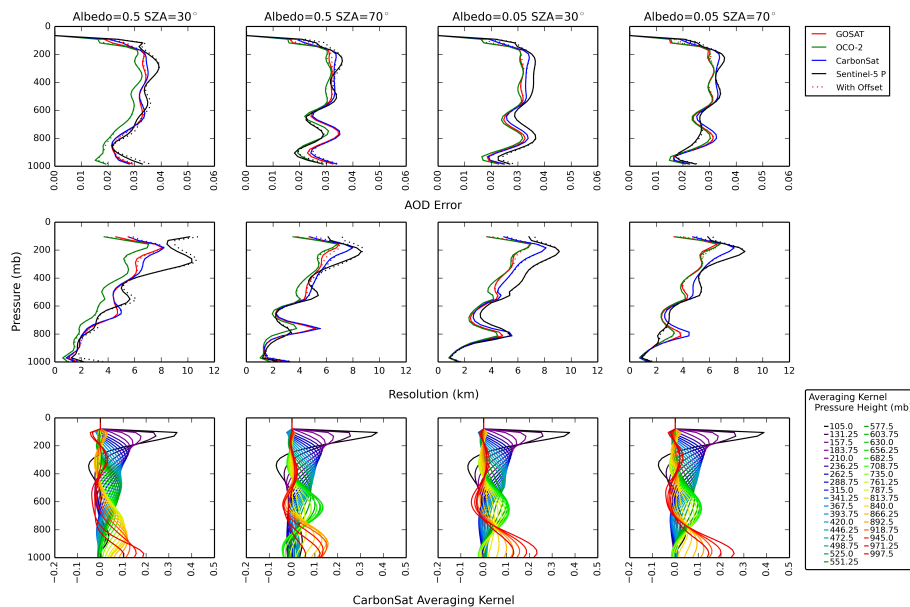
Figure 5. As Fig. 4 but for scenario B.
