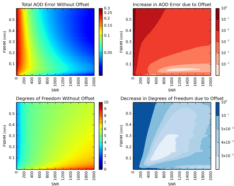
Figure 3. Total AOD error (top left panel) and DoF (bottom left panel) for the aerosol profile retrieval for scenario A, SZA 30° and albedo 0.5 as a function of continuum SNR and spectral resolution (as given by the FWHM of the ILS) without including an intensity offset in the retrieval. The panels on the right show the change in total AOD error and DoF when including an this offset.
