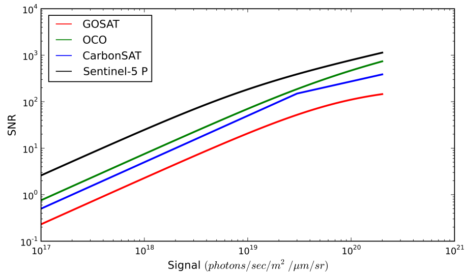
Figure 2. Assumed signal-to-noise (SNR) models for the four instruments GOSAT, OCO-2, CarbonSat and S-5 P.
