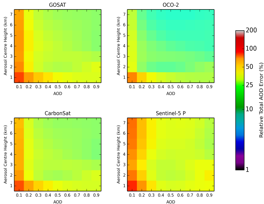
Figure 8. Total AOD error (given as a relative error) as a function of aerosol centre height and AOD for the four instruments for a SZA of 30^\circ and albedo of 0.5. Intensity offset is included in the retrieval.
