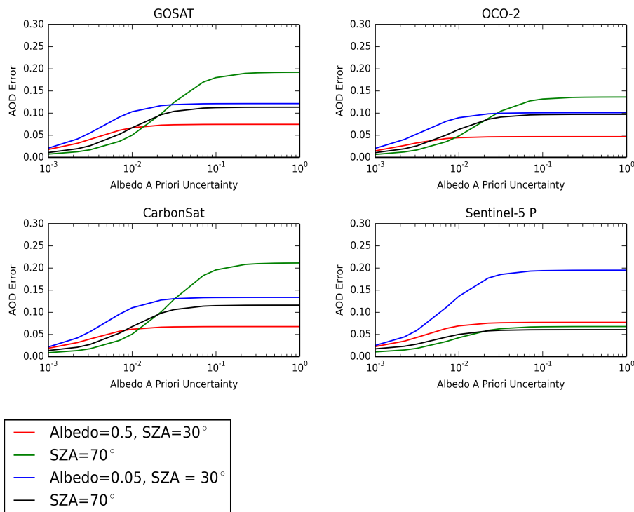
Figure 11. Total AOD error for the aerosol profile retrieval for scenario A for different albedo constraints given by the a priori uncertainty.
