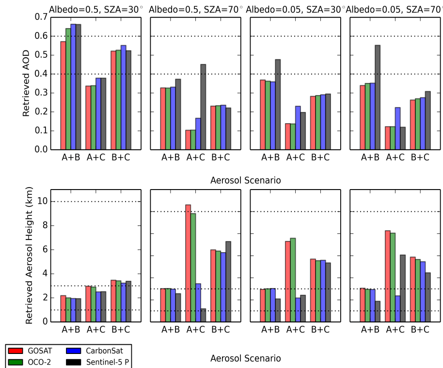
Figure 10. AOD and height errors for the parameterised aerosol retrievals for the combined aerosol scenarios A + B, A + C and B + C. In the top row the horizontal lines indicate the true AOD values for each case, i.e. the sum of both layers. In the bottom row they show the heights of each individual layer as a reference noting that the prior value for each scenario is the lowest layer height.
