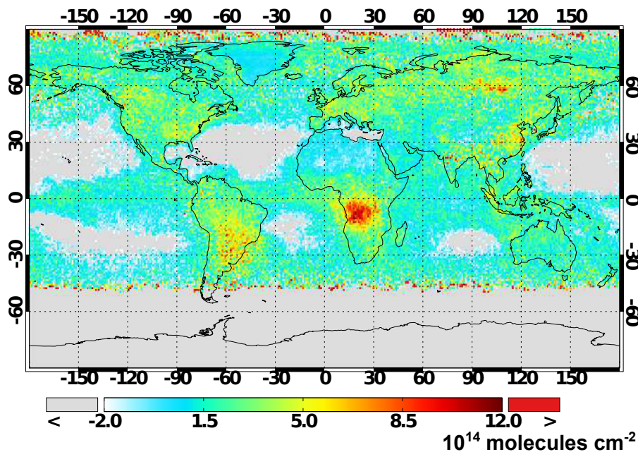
Figure 13. Monthly mean glyoxal slant column densities retrieved for July 2006 ( \text{molecules cm}^{-2} ).
