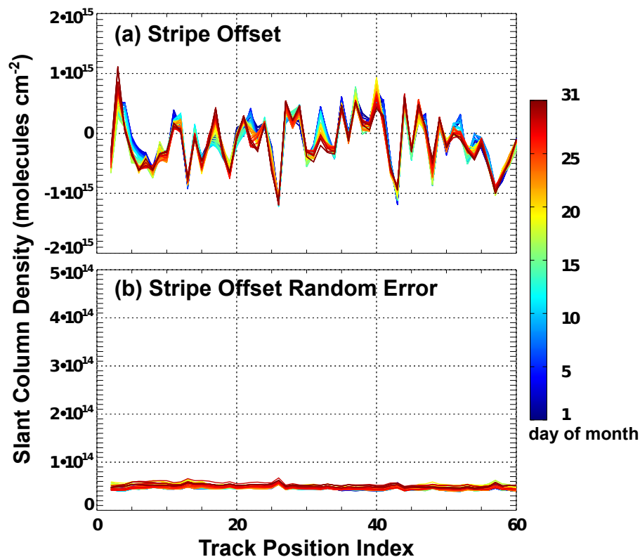
Figure 7. (a) Stripe offset (molecules cm -2 ) derived from a running 5 day mean of the slant columns retrieved over the sahara (20–30° N, 10° W–30° E) for July 2006 as a function of cross track position. Lines are color coded by day of the month. (b) Estimate of random SCD error (molecules cm -2 ) for (a) induced from noise in the measured radiances.
