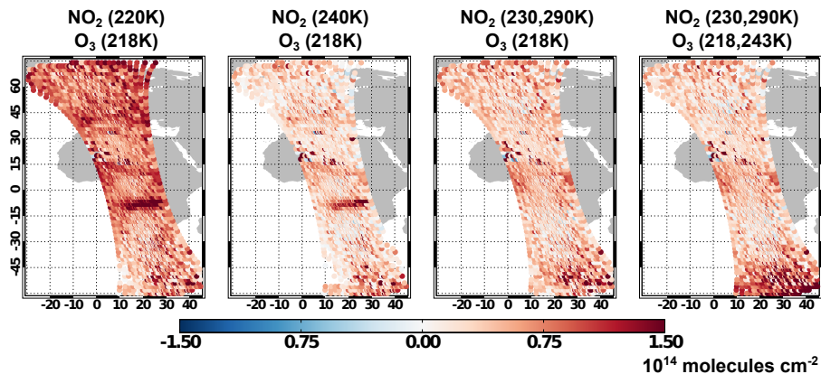
Figure 4. Differences between simulated and true glyoxal slant column densities ( \text{molecules cm}^{-2} ) retrieved using \text{NO}_2 and \text{O}_3 RCSs at different temperatures. Plot titles indicate temperatures of the RCSs used in the retrieval.
