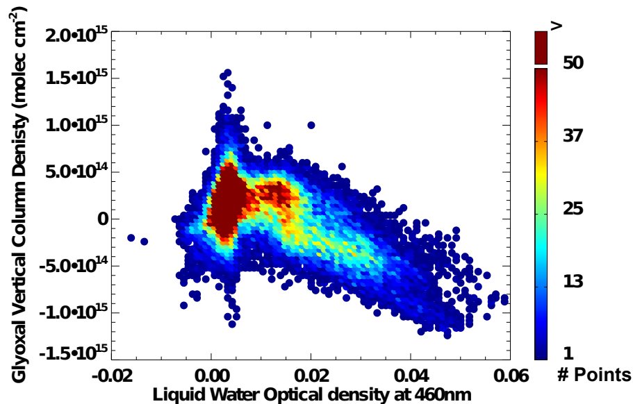
Figure 14. Scatterplot of glyoxal slant column densities (molecules cm -2 ) retrieved for July 2006 and liquid water optical depth at 460 nm. Points are color coded by the number of pixels falling within the grid cell corresponding to the point in the figure.
