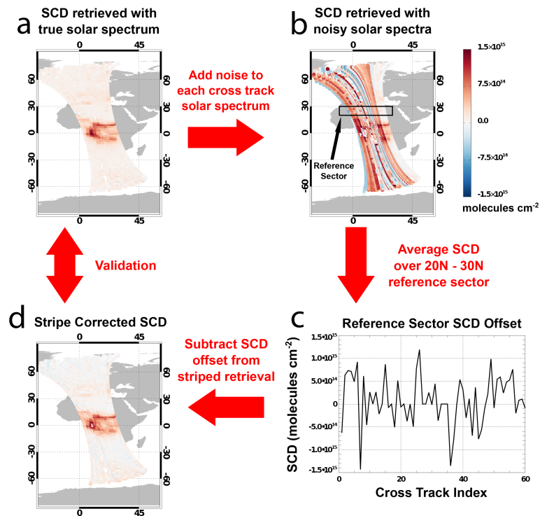
Figure 6. Simulation of stripes in the glyoxal retrieval OSSE. (a) Slant column densities ( \text{molecules cm}^{-2} ) retrieved from synthetic spectra, using a noise free solar spectrum. (b) Slant column densities ( \text{molecules cm}^{-2} ) retrieved from synthetic spectra, retrieved from synthetic spectra using solar spectra with a 3000 signal-to-noise ratio. (c) Mean slant column ( \text{molecules cm}^{-2} ) retrieved in the region 20\text{--}30^\circ\text{N} , 10^\circ\text{W}\text{--}30^\circ\text{E} from (b) . (d) The stripe corrected retrieval, derived from subtracting the mean slant columns in (c) from the columns retrieved using the noisy solar spectra.
