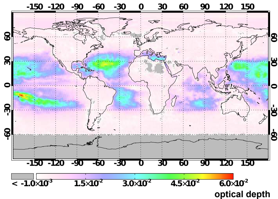
Figure 10. Retrieved liquid water optical depth at 460 nm for July 2006.
