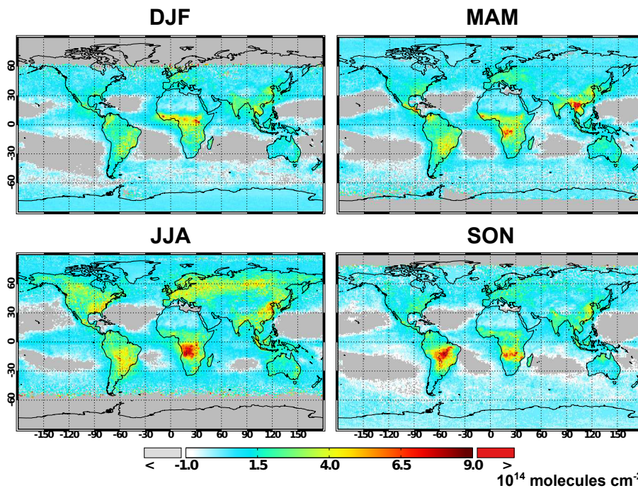
Figure 15. Seasonally averaged glyoxal VCDs ( \text{molecules cm}^{-2} ) retrieved from OMI for 2007.
