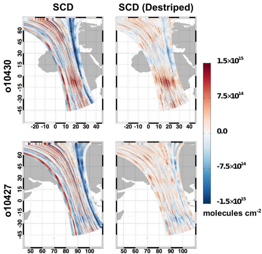
Figure 8. Left: retrieved glyoxal slant column densities ( \text{molecules cm}^{-2} ) using OMI data from orbits o10430 and o10427. Right: retrieved slant column density ( \text{molecules cm}^{-2} ) corrected for striping by subtracting the mean retrieved slant column between 20–30° N for each cross track position.
