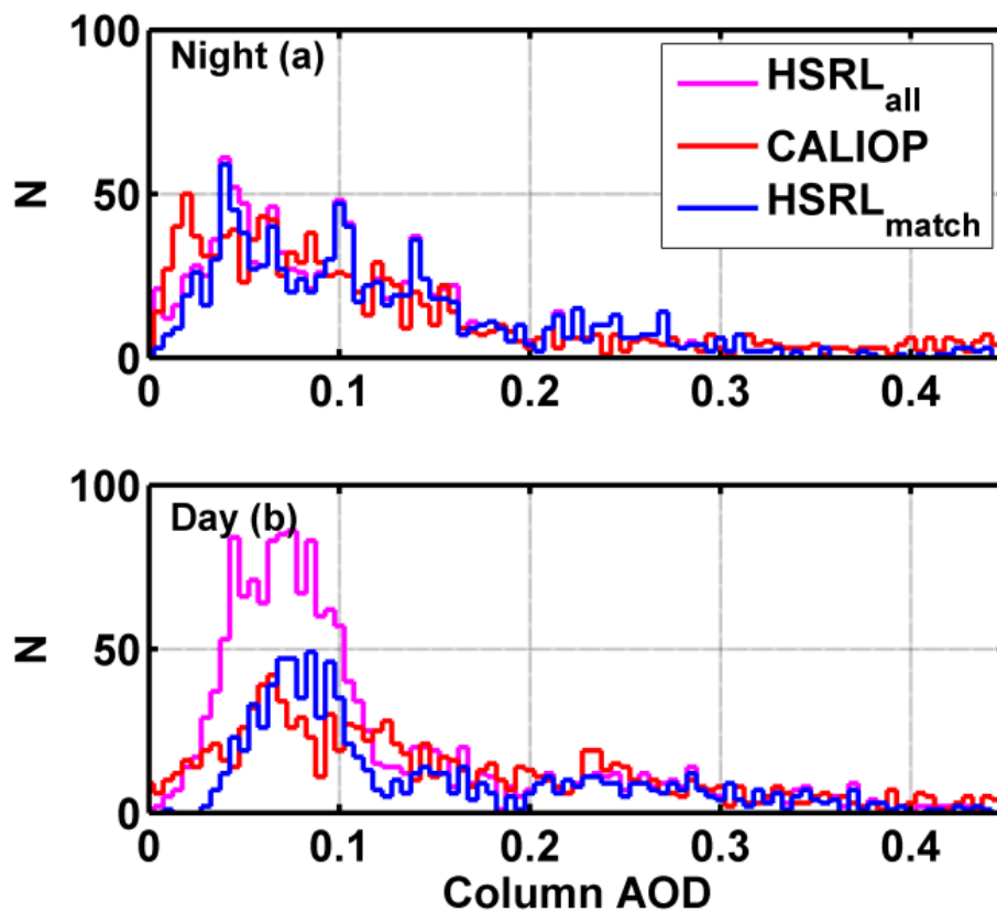
Figure 8. Night (a) and day (b) distributions of all HSRL 5 km column AOD (magenta), CALIOP column AOD (red), HSRL column AOD limited to scenes in which CALIOP detected features (blue).
