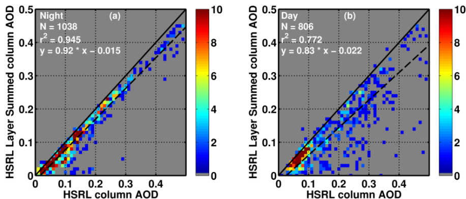
Figure 7. Night (a) and day (b) regressions of HSRL column and layer summed AOD. The solid black line is the one-to-one line and the regression is the dotted line.
