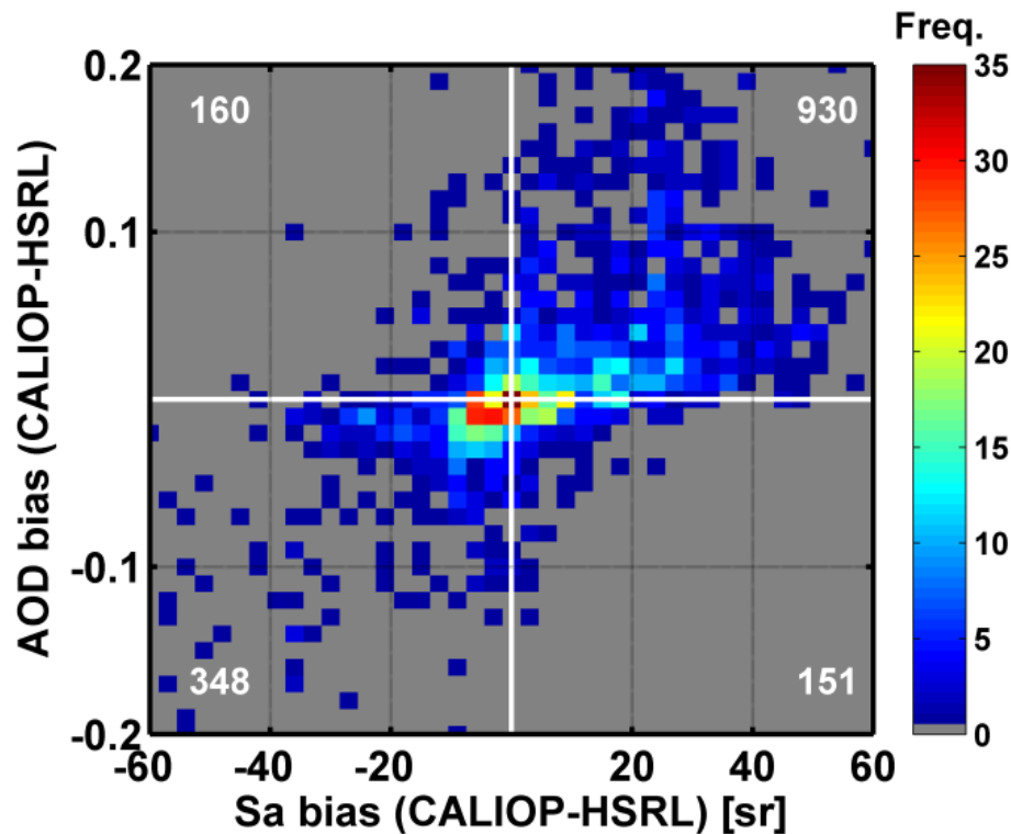
Figure 9. Layer AOD bias dependence (CALIOP – HSRL) as a function of layer lidar ratio bias (CALIOP – HSRL). Both day and night data are included, and the numbers represent the number of points in each quadrant.
