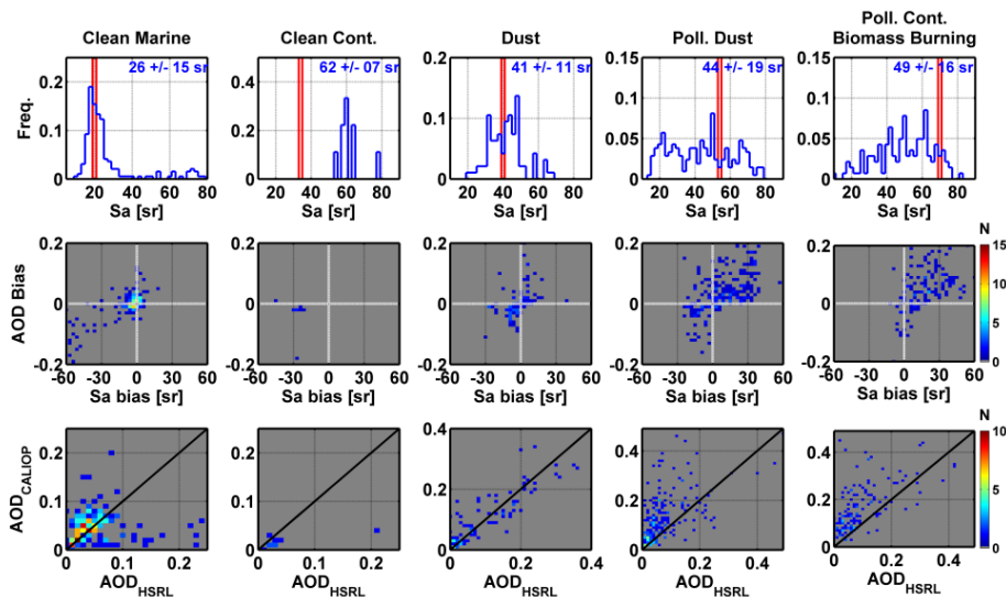
Figure 10. Daytime histograms of lidar ratio (top row), AOD bias (CALIOP – HSRL) vs. Sa Bias (CALIOP – HSRL) (middle row), and AOD (middle row) with AOD scatter plots (bottom row) for each CALIOP aerosol type (columns). The numbers in the top row are the means and standard deviations of the lidar ratios measured by the HSRL.
