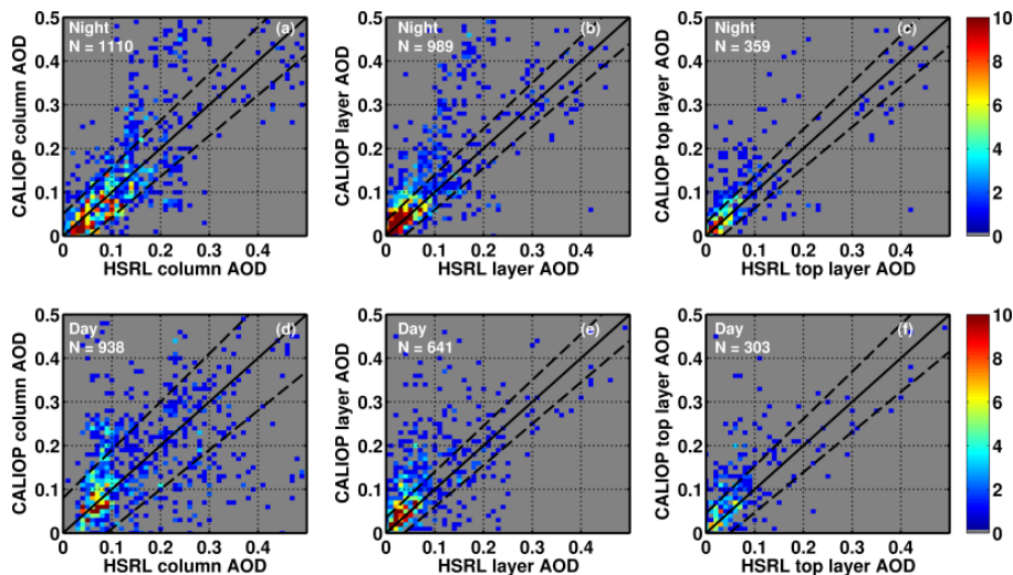
Figure 5. Scatter plots of column AOD ( a , d ), individual layer AOD ( b , e ), and top layer only AOD ( c , f ). The top row shows night lighting conditions and the bottom row shows daytime lighting. The color bar indicates the number of points in each grid cell. The one-to-one line is in solid black on all figures and the dashed lines represent the error estimates reported in Table 3.
