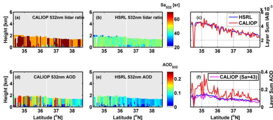
Figure 4. The CALIOP layer lidar ratio time series (a) and corresponding HSRL layer lidar ratio time series (b) from 07 February 2009. The corresponding CALIOP and HSRL layer AOD time series (d and e, respectively) , the layer summed IAB from CALIOP and HSRL (c) , and the column (layer summed) AOD from CALIOP and HSRL (f) . In (f) , the magenta line represents the CALIOP level 2 column AOD analyzed with a lidar ratio of 43 sr (see text).
