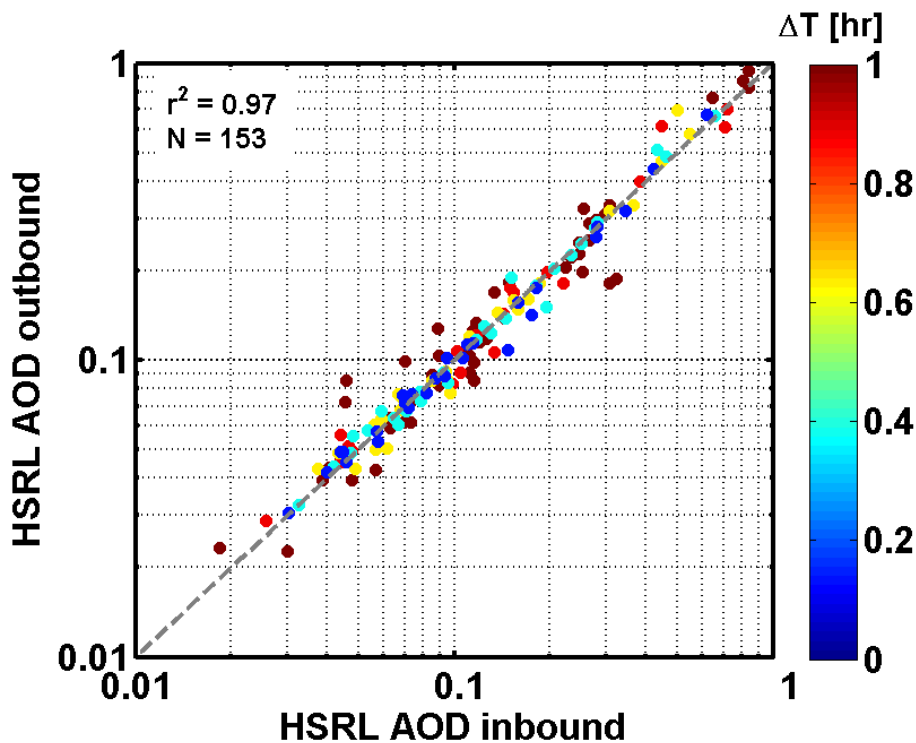
Figure 2. Spatially matched HSRL AOD measurements from out and back tracks with the colorbar indicating the temporal separation of the measurements. The dashed line is the 1–1 line.
