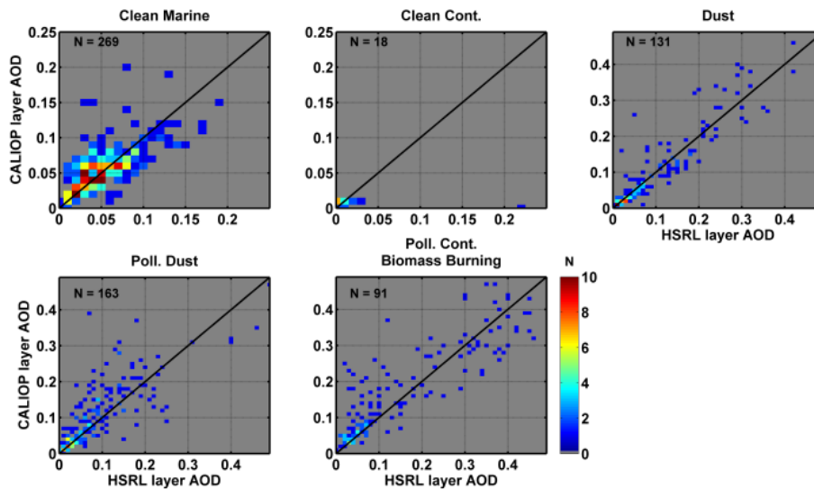
Figure 12. Combined daytime and nighttime scatterplots of CALIOP layer AOD and HSRL layer AOD for each aerosol type with the restriction that the CALIOP lidar ratio is within 30 % of the HSRL lidar ratio.
