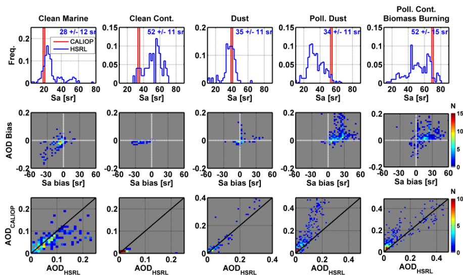
Figure 11. Nighttime histograms of lidar ratio (top row) AOD bias (CALIOP – HSRL) vs. Sa Bias (CALIOP – HSRL) (middle row), and AOD scatter plots (bottom row) for each CALIOP aerosol type (columns). The numbers in the top row are the means and standard deviations of the lidar ratios measured by the HSRL.
