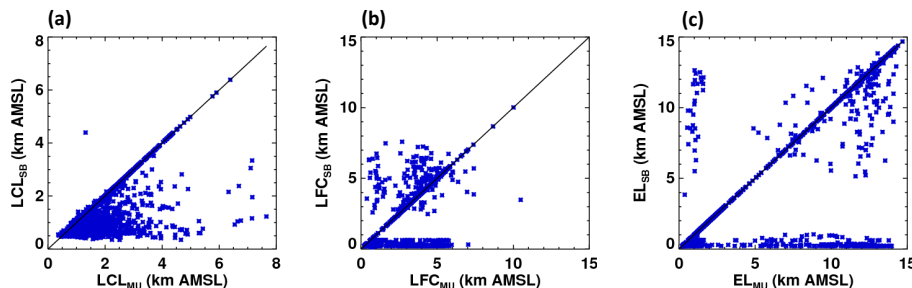
Figure 12. Scatter plots of convective levels, computed using RH corrected soundings, comparing estimates for surface parcel characteristics defined by the level with the maximum virtual temperature in the lowest kilometer (MU) and the lowest level in the sounding (SB) for (a) LCL, (b) LFC and (c) EL.
