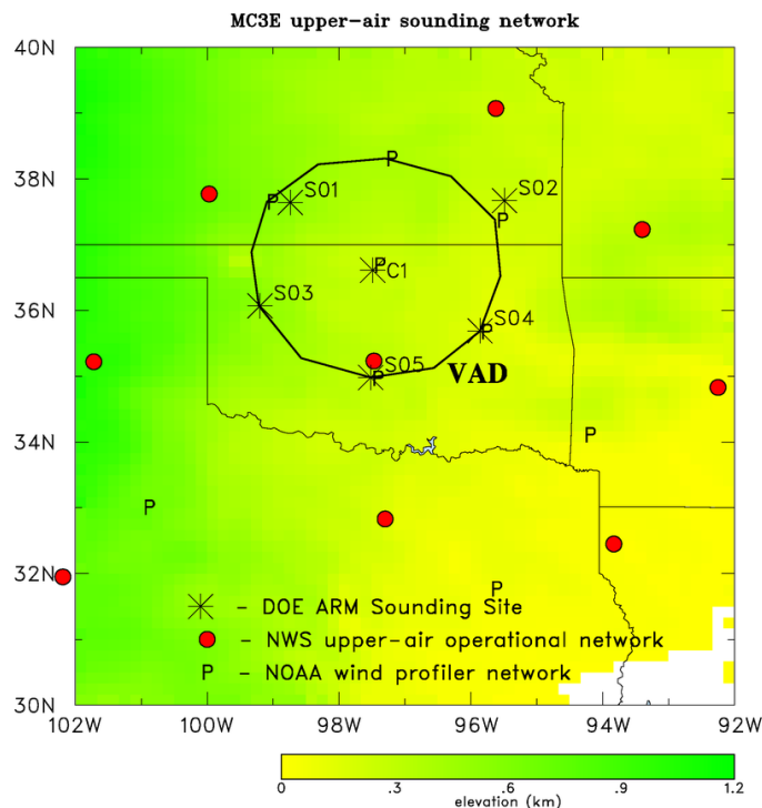
Figure 1. Map of the MC3E ground-based observing domain including the outer sounding domain: Central Facility [C1 Lamont, Oklahoma (OK) 36.695° latitude, −97.485° longitude] S1 Pratt, Kansas (KS) [37.7, −98.75]; S2 Chanute, KS [37.674, −95.488], S3 Vici, OK [36.071, −99.204]; S4 Morris, OK [35.687, −95.856]; and S5 Purcell, OK [34.985, −97.522]. Also shown on this map are surrounding sites from the NWS operational sonde network and NOAA profiler network. Variational analysis domain (VAD) is indicated with polygon. Shading indicates elevation with scale at bottom.
