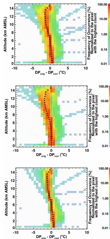
Figure 6. Two-dimensional histogram of humidity differences – Dew Point (DP) difference between the original sounding and the humidity corrected sounding for all soundings (top), day-time soundings (middle) and nighttime soundings (bottom). The dotted black curve represents the median value at each height.
