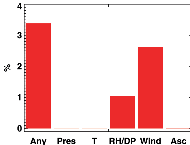
Figure 5. Histogram summarizing the percentage of observations for all sites outside of data quality check limits as defined in Table 4. Any = All data quality checks combined, Pres = Pressure, T = Dry Bulb Temperature, DP = Dew Point Temperature, RH = Relative Humidity, Wind = Horizontal wind speed and direction, Asc = Ascent Rate.
