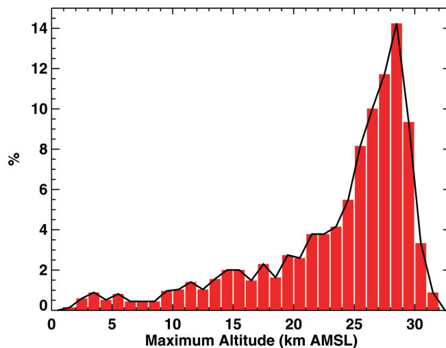
Figure 4. Frequency of occurrence (normalized by the total number of soundings) of the maximum height obtained by MC3E soundings, for all sites.
