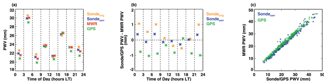
Figure 7. Diurnal variation of PWV at site C1 – (a) Retrieved from an uncorrected sounding profile (yellow), a corrected sounding (blue), MWR observations (red) and GPS observations (green) averaged over all sondes in 3 h time windows, (b) absolute differences between retrieved PWV estimates and (c) scatter plot of retrieved PWV from corrected radiosonde profiles and GPS.
