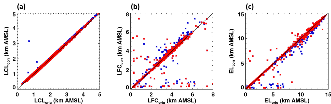
Figure 10. Scatter plots of convective levels comparing original (orig) and humidity corrected (corr) soundings for (a) LCL, (b) LFC and (c) EL. Daytime soundings (12:00–23:00 UTC) are indicated with red markers while nighttime soundings are blue. Convective indices are computed using the level of maximum virtual temperature in the lowest kilometer a.g.l. of the sounding.
