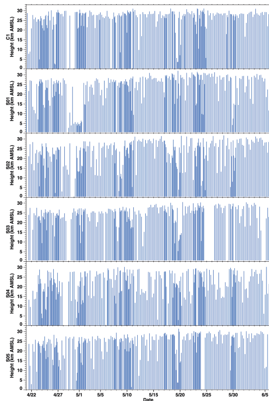
Figure 3. Sounding inventory summarizing the time of each launch and maximum height attained by each sonde for C1 (top), S1, S2, S3, S4, S5 (bottom). Each bar is color coded to represent nominal data quality (blue = good, red = indeterminate or bad).
