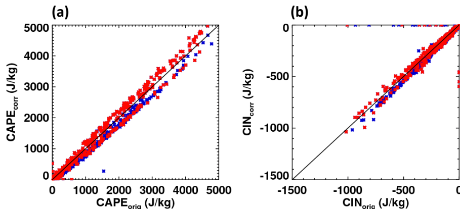
Figure 11. Scatter plots of convective levels comparing original (orig) and humidity corrected (corr) soundings for (a) CAPE and (b) CIN. Daytime soundings (12:00–23:00 UTC) are indicated with red markers while nighttime soundings are blue. CAPE and CIN are computed using the level of maximum virtual temperature in the lowest kilometer a.g.l. of the sounding.
