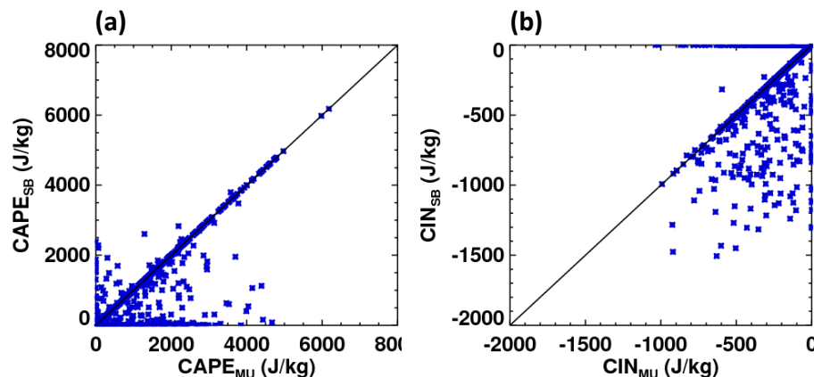
Figure 13. Scatter plots of convective levels, computed using RH corrected soundings, comparing estimates for surface parcel characteristics defined by the level with the maximum virtual temperature in the lowest kilometer (MU) and the lowest level in the sounding (SB) for (a) CAPE and (b) CIN.
