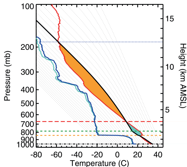
Figure 8. Graphical representation of convective indices – Central Facility radiosonde profile for 11 May 2011 02:34 UTC graphically illustrating the convective indices of CAPE (orange shading) and CIN (cyan shading) and relevant buoyancy levels including the lifting condensation level (LCL, green dashed), level of free convection (LFC, red dashed) and equilibrium level (blue dotted). The environmental virtual temperature profile is shown by the solid red line, adiabatic virtual parcel temperature is shown by the solid black line, the observed dew point temperature profile is shown with the dark blue line and the RH corrected dew point temperature profile is shown with the cyan line.
