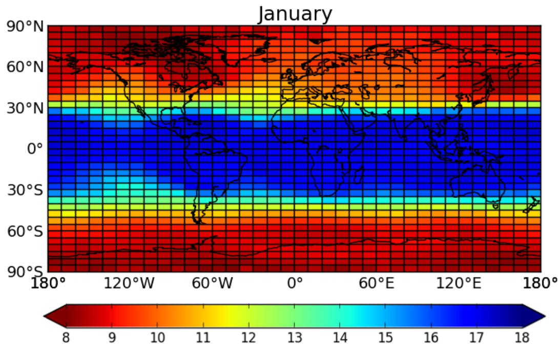
Fig. 2. Long-term monthly mean (2001 to 2013) first tropopause altitude (km) for January calculated for 5° latitude x 10° longitude grid boxes.
