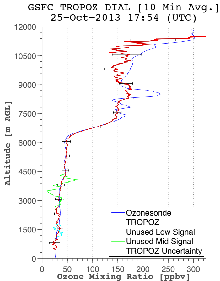
Fig. 3. Revised Ozone Profile with Channels
