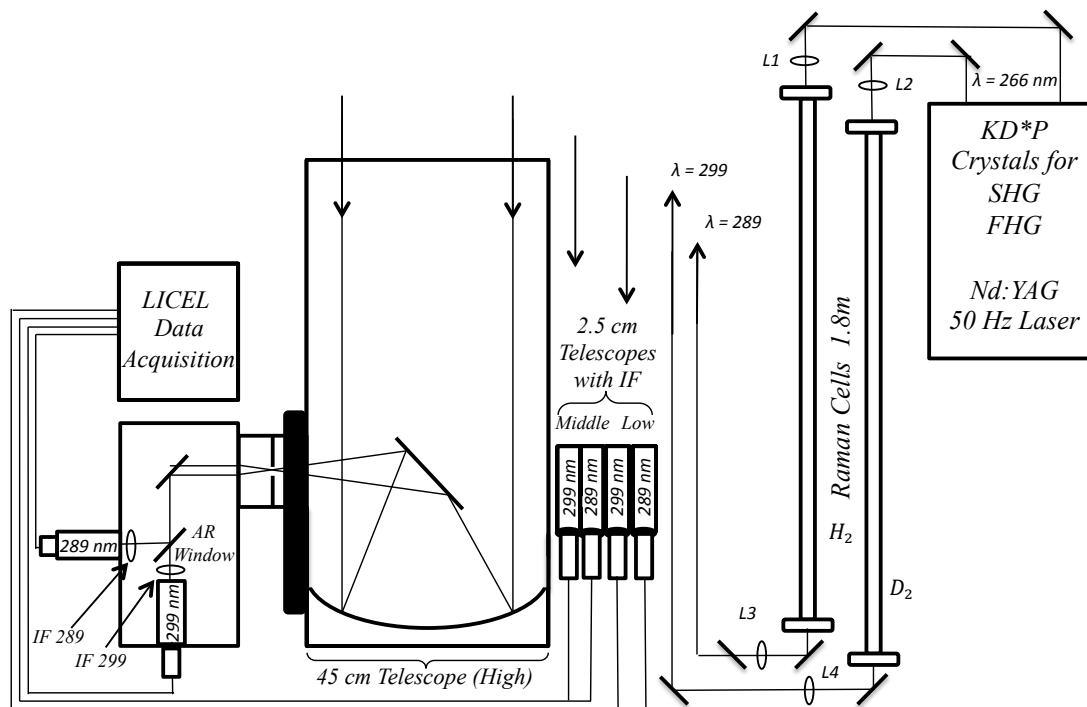
Fig. 5. Updated Hardware Schematic
