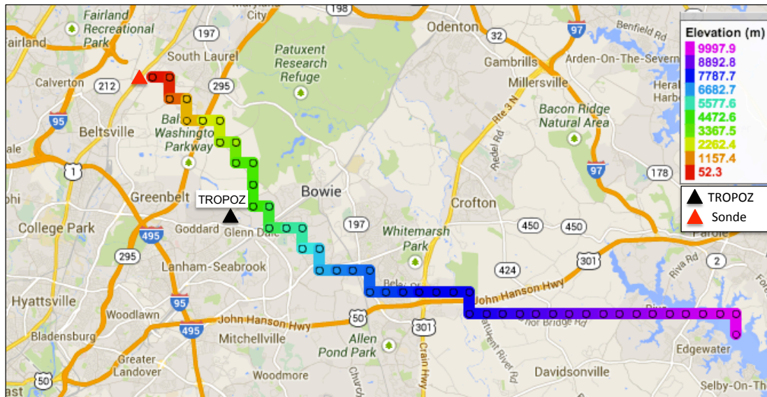
Fig. 4. Updated Sonde Map Location
