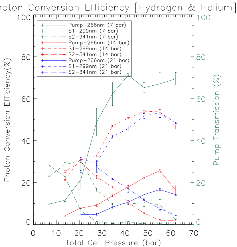
Fig. 1. Revised Raman Cell units (H2)
