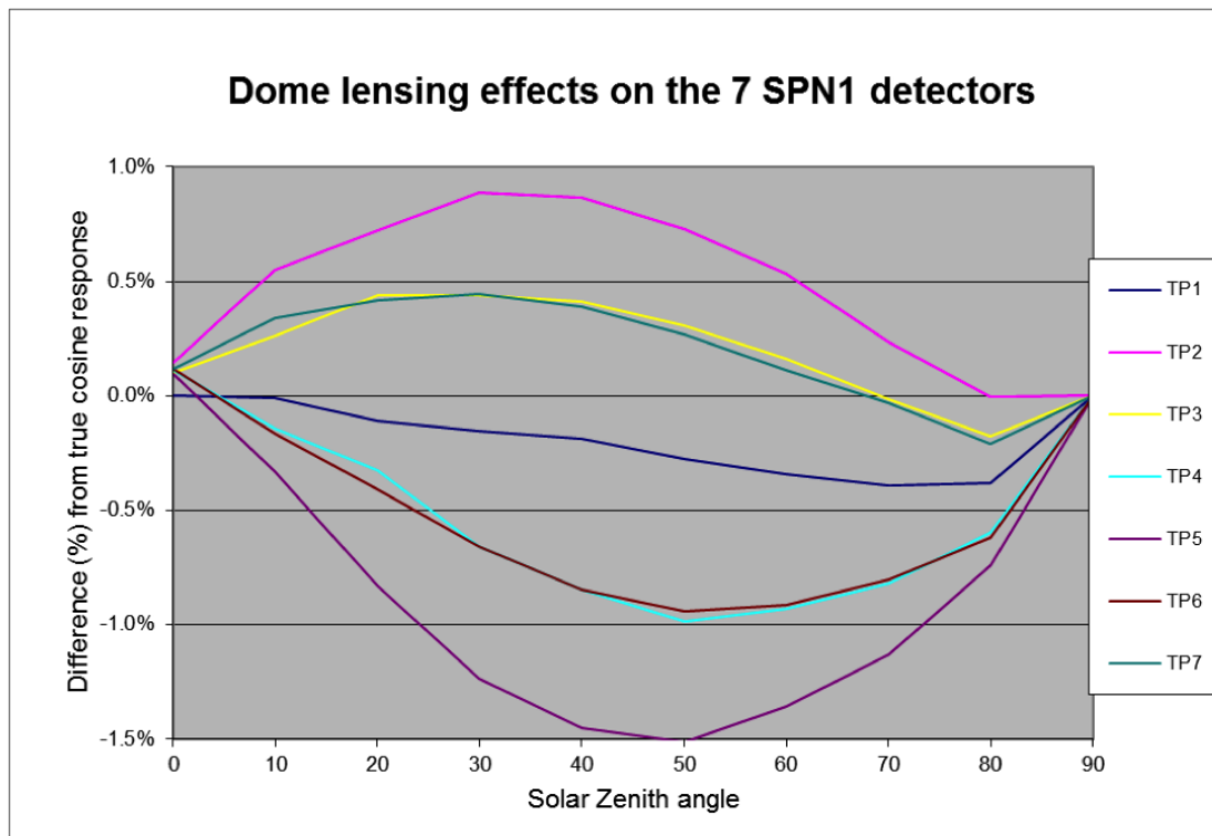
Fig. 2. Dome lensing effects on the 7 SPN1 detectors
