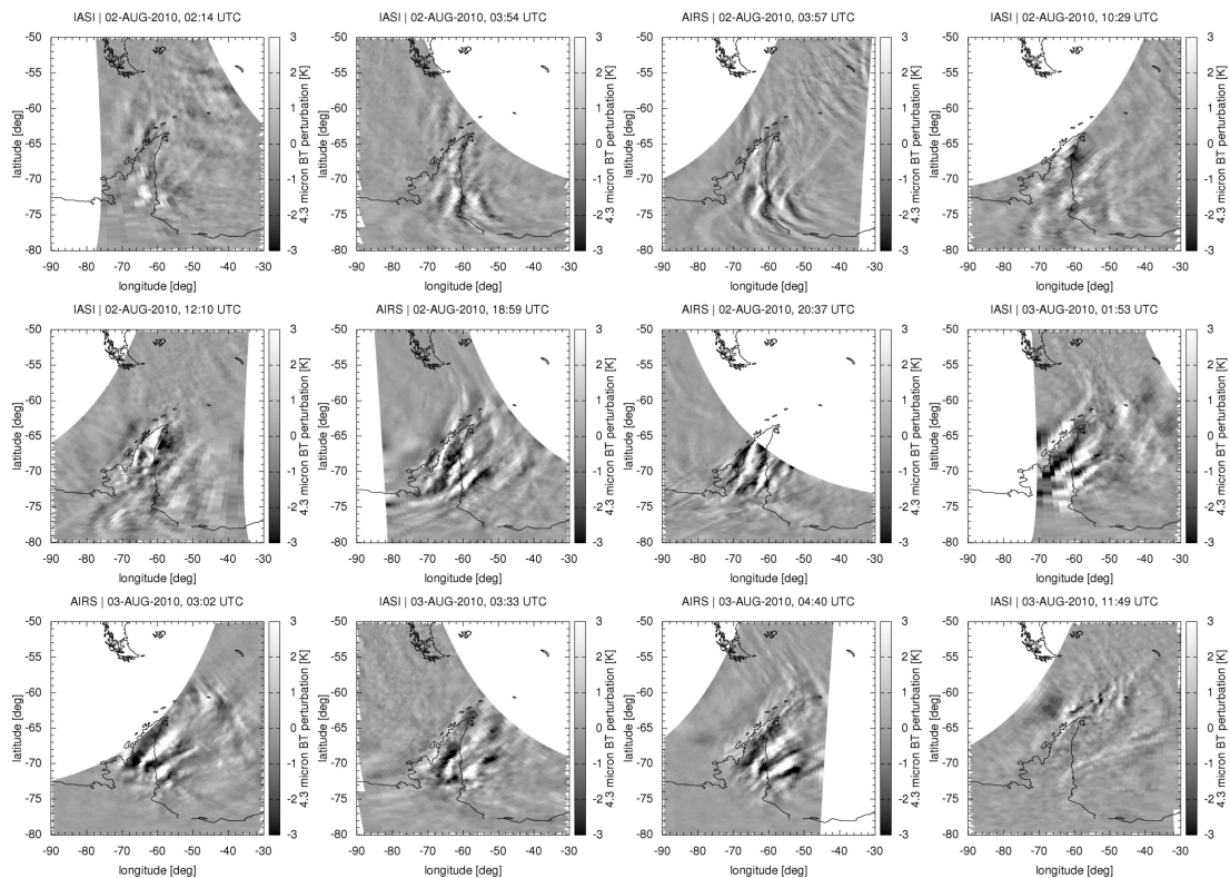
Fig. 7. 4.3 \mu\text{m} brightness temperature perturbations showing stratospheric temperature perturbations of a mountain wave event at the Antarctic Peninsula on 2–3 August 2010. Plots show observations from selected AIRS and IASI overpasses in temporal order.
