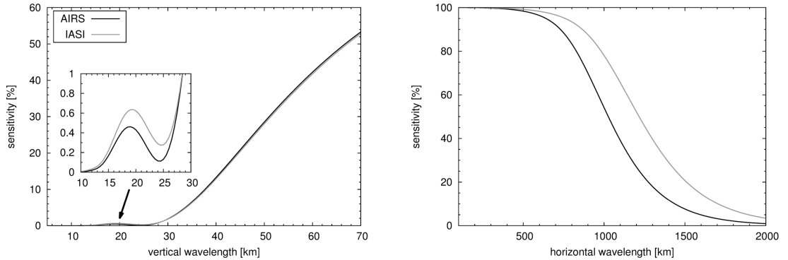
Fig. 5. Sensitivity of AIRS and IASI brightness temperature variances to wave perturbations with different vertical wavelengths (left) and horizontal wavelengths (right). Sensitivity to vertical wavelength was calculated with the spectral mean kernel functions shown in Fig. 4. Sensitivity to horizontal wavelength is determined by the detrending procedure. The plot shows the maximum horizontal sensitivity, which is obtained for gravity waves propagating in the across-track direction. Note that the sensitivity to horizontal wavelengths shorter than 100 km was not analyzed here. In this case the sensitivity is limited by the satellite footprint size (see text for details).
