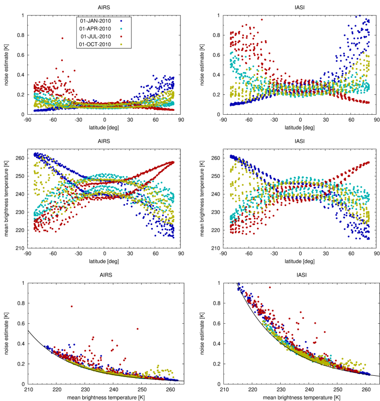
Fig. 6. Noise estimates (top) and mean scene temperatures (middle) as a function of latitude as well as correlation plots of noise and scene temperatures (bottom) for AIRS (left) and IASI (right). Individual dots represent mean values for boxes of about 2000 \times 2000 \text{ km}^2 . Colors refer to different days of measurement. Black curves show scaling of NEDT with scene temperature.
