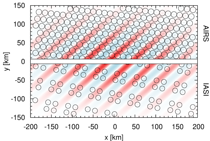
Fig. 2. Illustration of the scan patterns of AIRS (upper half of plot) and IASI (lower half) close to the nadir direction. Contour surface in the background shows a wave pattern with 50 km horizontal wavelength. Circles show individual footprints (diameter represents their size). We refer to the distance between the footprints as ‘spatial sampling’ and we refer to the size of the footprints as ‘spatial resolution’.
