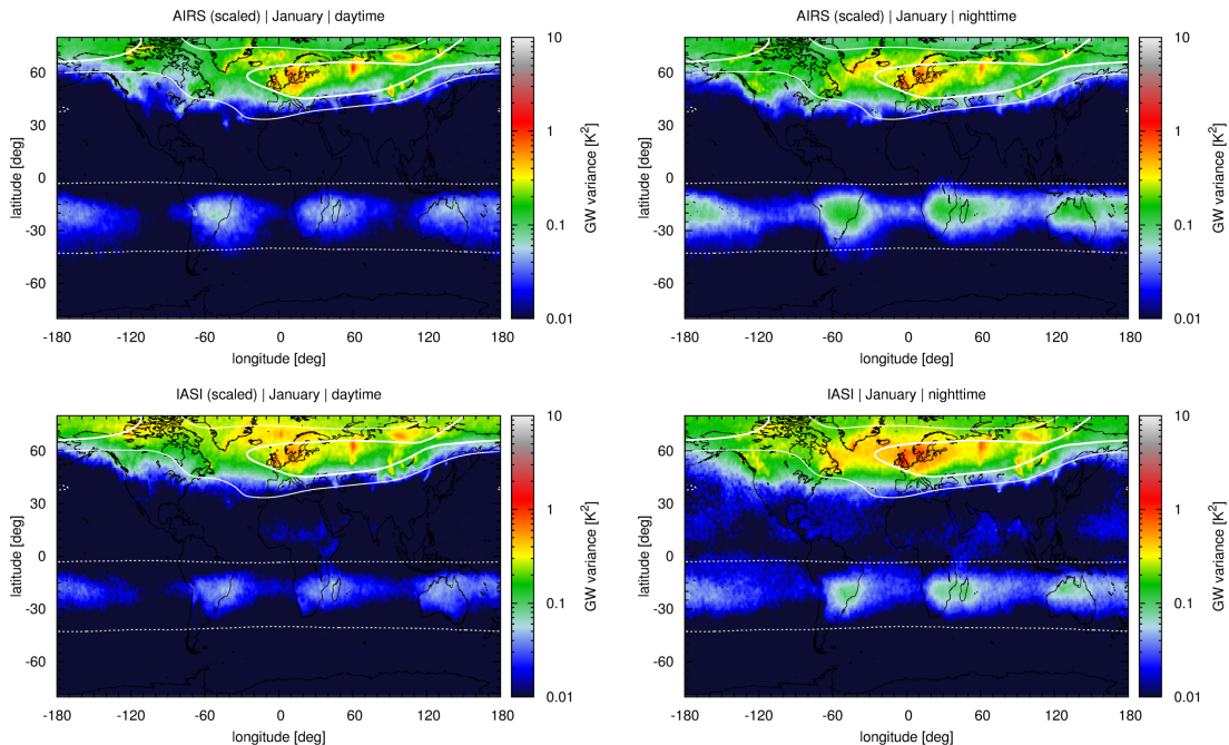
Fig. 13. Climatological maps of 4.3\ \mu\text{m} brightness temperature variances due to gravity waves in January for AIRS (top) and IASI (bottom) at daytime (left) and nighttime (right). Shown are mean variances based on the years 2008 to 2012. Data have been scaled by the factors c_{\text{ai}} and c_{\text{dn}} to better compare regional features. White contour lines show zonal winds of -20\ \text{m/s} (thin, dotted), 20\ \text{m/s} (thin, solid), and 40\ \text{m/s} (thick, solid) at 6.8\ \text{hPa} from ERA-Interim.
