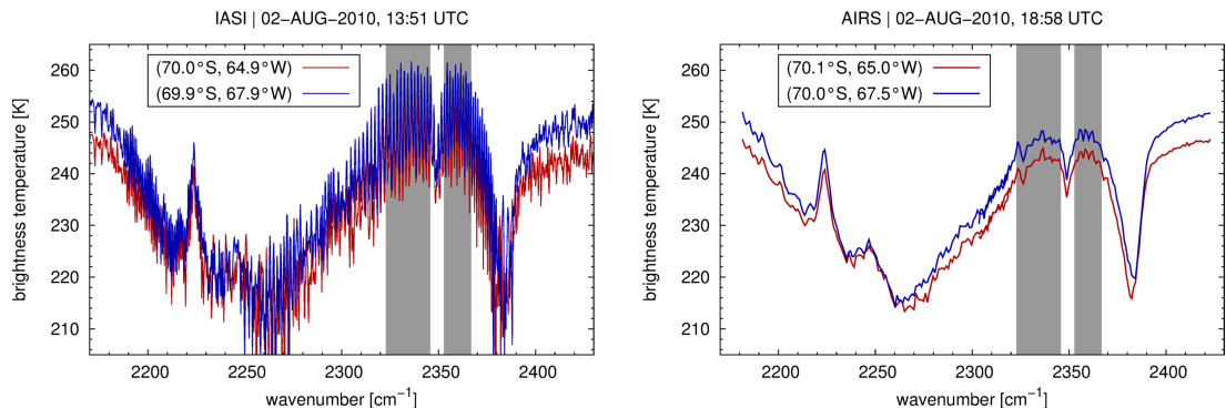
Fig. 3. IASI (left) and AIRS (right) radiance spectra measured during a mountain wave event at the Antarctic Peninsula on 2 August 2010. AIRS spectra are shown at nominal spectral resolution. IASI spectra were convolved with a Gaussian spectral response function with a full-width at half-maximum of 1.9\text{cm}^{-1} to obtain a spectral resolution similar to AIRS at 4.3\mu\text{m} . Red and blue curves show spectra measured at nearly the same time and latitude, but separated by 100 km zonal distance (half wavelength of mountain wave). Gray Spectral mean radiances in the gray shaded spectral regions are analyzed for stratospheric gravity waves.
