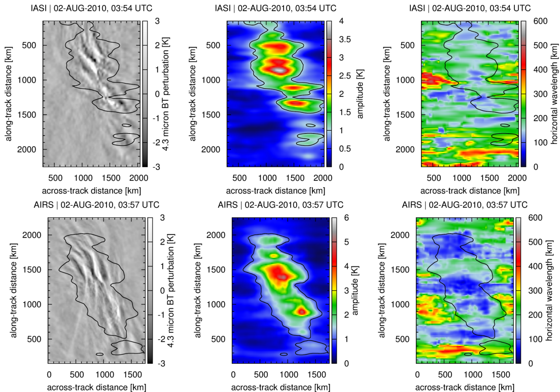
Fig. 8. Spectral analyses for two satellite overpasses of IASI (top) and AIRS (bottom) during the mountain wave event shown in Fig. 7. Data are shown on the along-track and across-track measurement grid, with a descending orbit for IASI and an ascending orbit for AIRS. Black contour lines indicate areas with wave amplitudes larger than 1 K.
