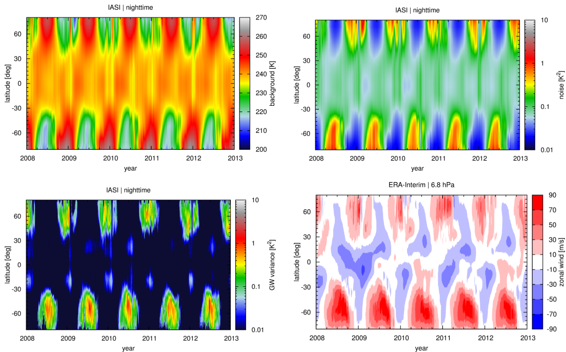
Fig. 11. Time series of 4.3 \mu\text{m} brightness temperature background levels (top, left), noise estimates (top, right), and gravity wave variances (bottom, left) from IASI nighttime observations. Time series of ERA-Interim zonal mean zonal winds at 6.8 hPa (bottom, right).
