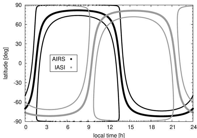
Fig. 1. Local time versus latitude of AIRS and IASI observations. Thick curves represent the nadir measurement track. Thin curves represent the outermost measurement tracks. AIRS and IASI have sun-synchronous orbits, which combine orbit altitude and inclination in such a way that the satellite ascends or descends over any given latitude at the same local time. The orbit parameters stay constant over the time period of the mission.
