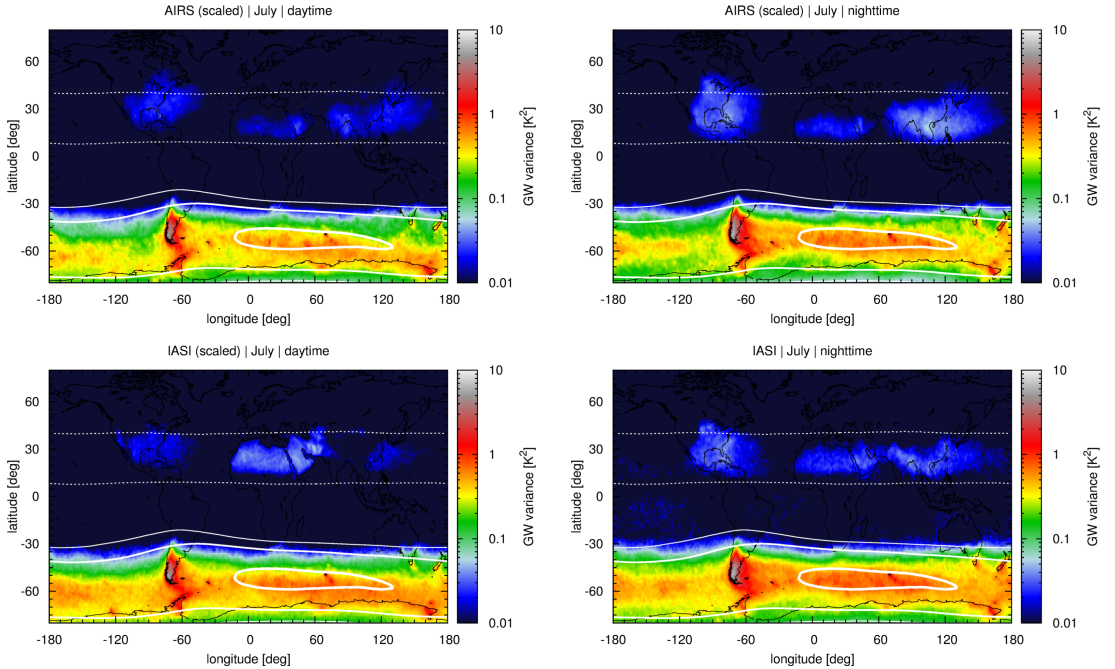
Fig. 14. Same as Fig. 13, but for July. Another thick contour line was added, showing zonal winds of 80 m/s in the southern hemisphere.
