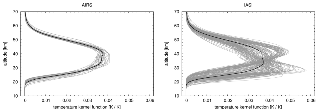
Fig. 4. Temperature kernel functions for the 4.3\ \mu\text{m} \text{CO}_2 fundamental band for AIRS (left) and IASI (right). Gray curves show kernel functions for individual channels within spectral ranges from 2322.5 to 2346.0\ \text{cm}^{-1} and 2352.5 to 2367.0\ \text{cm}^{-1} . Black curves show spectral mean kernel functions. Kernel functions were calculated for a mid-latitude reference atmosphere and the nadir geometry. Note that the absolute values of the kernel functions depend on the vertical grid spacing (1 km) and interpolation scheme (linear) applied in the radiative transfer calculations.
