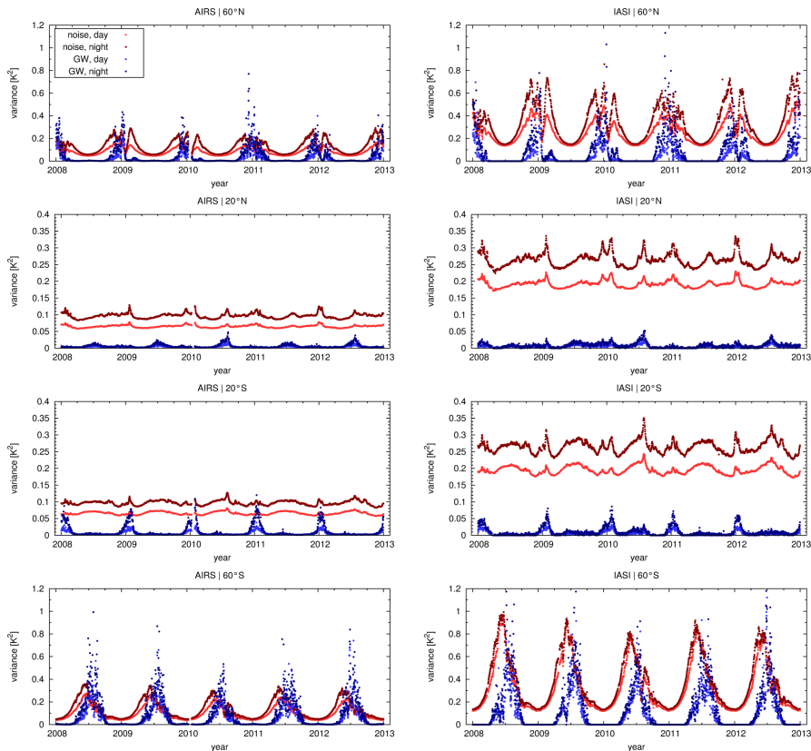
Fig. 12. Time series of 4.3 \mu\text{m} brightness temperature variances due to gravity waves and noise estimates for AIRS (left) and IASI (right) at different latitudes (see plot titles). Note that the range of variances shown here differs between the lower and higher latitudes.
