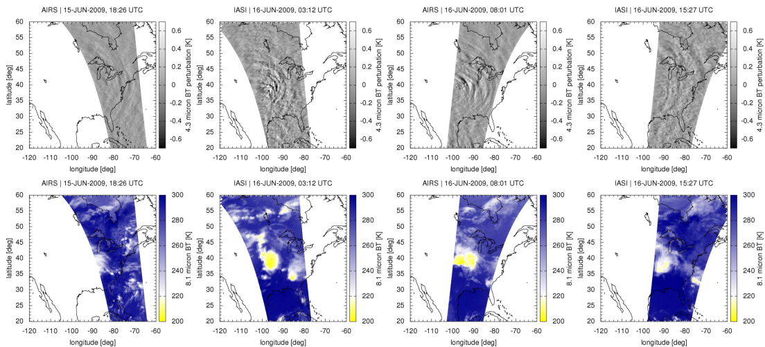
Fig. 10. 4.3\ \mu\text{m} brightness temperature perturbations (top) from a convective wave event over the North American Great Plains on 15–16 June 2009. Note that perturbations are much smaller compared with Figs. 7 and 9. The 8.1\ \mu\text{m} brightness temperature maps (bottom) show cold cloud surfaces ( < 220\ \text{K} ) related to mesoscale convective systems.
