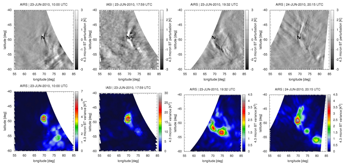
Fig. 9. 4.3\ \mu\text{m} brightness temperature perturbations (top) and local variances (bottom) related to orographic waves near Kerguelen Islands and Heard Island on 23–24 June 2010. The local variances are calculated based on the perturbations of footprints within circles with 100 km radius. Note that fixed color bar ranges are used for perturbations, whereas variable ranges are used for the variances.
