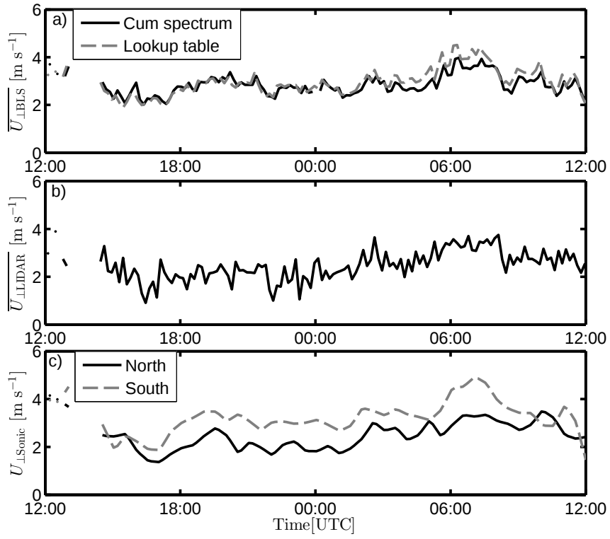
Fig. 3. Time series of U as estimated by (a) the scintillometer, (b) the Doppler lidar, and (c) the sonic anemometer for DOY 279 and 280.
