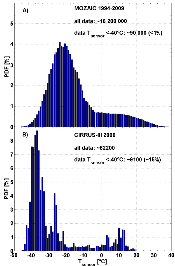
Fig. 1. Frequency of occurrence for observations of T_{\text{sensor}} during approx. 15 years of MOZAIC (top) and CIRRUS-III (bottom), respectively.
