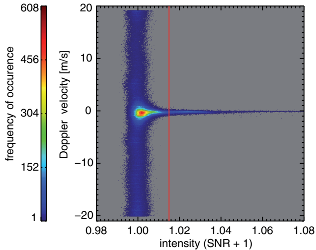
Figure 2. Intensity ( SNR + 1 ) vs. Doppler velocity plot based on Doppler lidar measurements from two measurement different time periods during stable atmospheric conditions (0600–0700 UTC 2013-07-05 6–7 UTC 2013-07-05 and 0700–0800 UTC 2013-07-22 7–8 UTC 2013-07-22) with which were characterized by quiescent atmospheric conditions, indicated by vertical velocities close to zero. The used Doppler lidar configuration was STARE, i.e. a continuous vertically pointing laser beam. For the range 0.992 < (SNR + 1) < 1.006 the Doppler velocities are uniformly distributed over the search band ( \pm 19.4 \text{ ms}^{-1} ) indicating a relatively high fraction of "bad" estimates. For SNR + 1 \geq 1.006 the Doppler lidar delivers plausible values ("good" estimates). The red line indicates the SNR-threshold (SNR + 1) = 1.015 used for the data analysis in the present paper.
