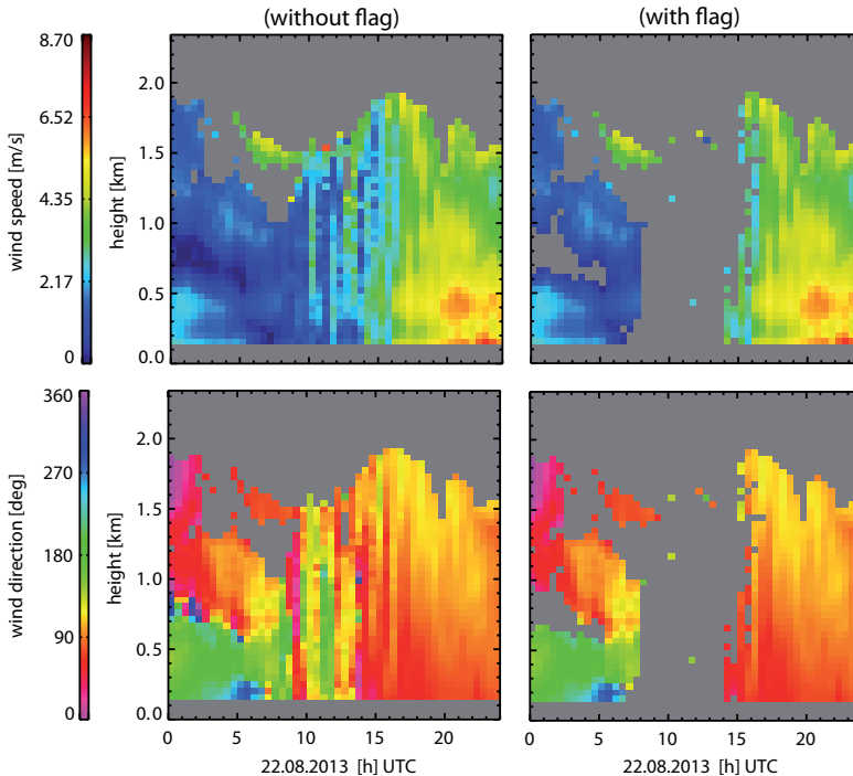
Figure 4. Left column: Example for non-quality assured wind profile retrievals (top: wind speed, bottom: wind direction) from Doppler lidar measurements for a typical summer day (2013-08-22). Each profile represents a 30 min average of VAD Doppler Lidar lidar measurements with one scan lasting about 3 minutes. Right column: Same wind retrievals as shown in the left column but where profiles with test parameters R^2 < 0.95 and CN > 10 have been discarded.
