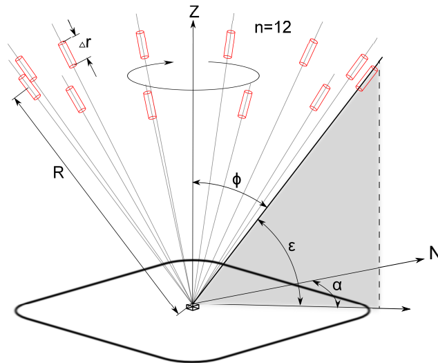
Figure 1. Example for a velocity-azimuth display (VAD) scanning technique for n = 12 beam directions. The laser beam of the Doppler Lidar-lidar points upwards with a constant elevation angle \varepsilon and rotates around the vertical Z with configurable azimuth angles \alpha . The red volumes symbolize an emitted "light"-disturbance of a specified period of time (i.e. pulse width \Delta t ) travelling along the line-of-sight (LOS). R is the range of the measurement along LOS and \Delta r defines the pulse length. The latter is related to the pulse width via \Delta r = c * \Delta t / 2 , with c denoting the speed of light.
