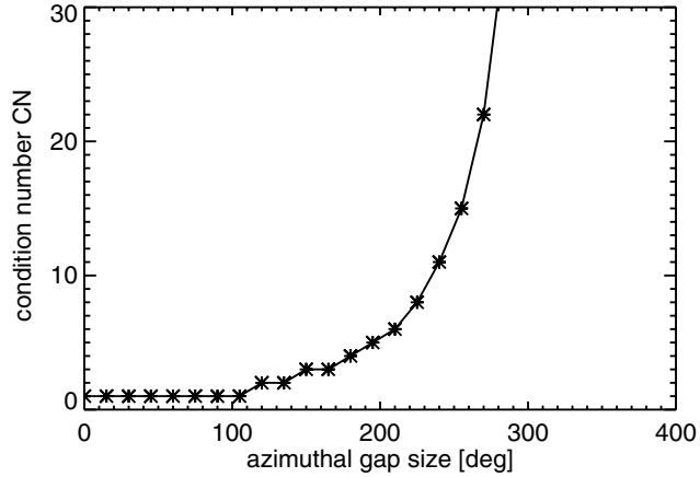
Figure 3. Condition number (CN) vs. azimuthal gap size for a VAD scan with 15^\circ intervals of azimuth \alpha and a constant elevation angle \epsilon = 75^\circ .
