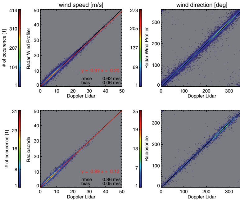
Figure 9. top: Scatter plots of one-year 30 min averaged horizontal wind speed and direction from Doppler Lidar and 482 MHz Radar Wind Profiler measurements (DLWR) bottom: Scatter plots of one-year 30 min averaged horizontal wind speed and direction from Doppler lidar and Radiosonde (DLRS). top and bottom: in principle all The scatter plots include measurements from all heights. The red line indicates the identity line.
