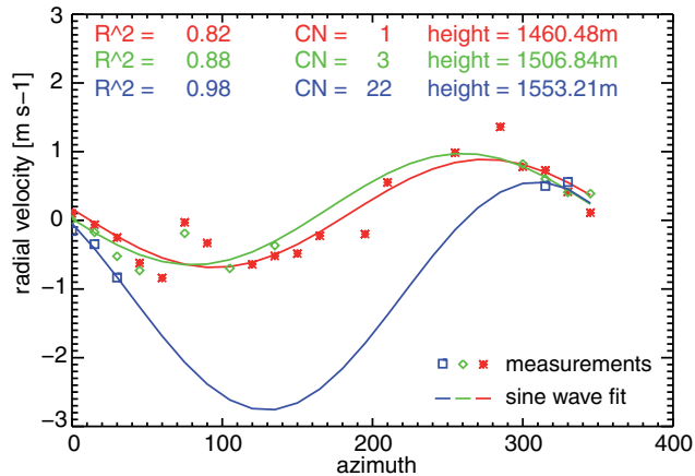
Figure 7. Examples for three sine wave fits used to reconstruct the 30 min averaged wind profiles shown in Fig. 4 at the three adjacent heights h_1 = 1460.48 \text{ m} , h_2 = 1506.84 \text{ m} and h_3 = 1553.21 \text{ m} for the single time stamp 12:02 UTC. Additionally for each fit the quality control parameters R^2 and CN are also given. The sine wave fit at h_3 has a high R^2 but due to the large azimuthal gap size within the measurements the condition number CN is relatively high indicating a high degree of multicollinearity. The latter results in implausible magnitudes of the wind speed yielding unphysical vertical gradients in the wind speed field (see also the outstanding red pixel in the wind speed profile shown in Fig. 4 at the time stamp 12:02 UTC).
