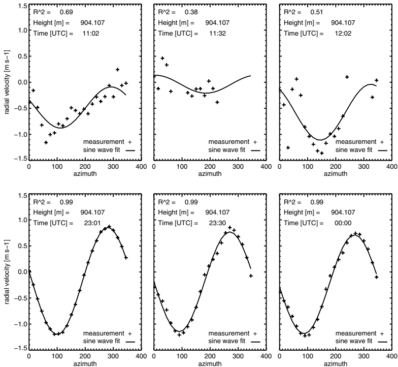
Figure 6. Examples for single sine wave fits into 30 min averaged VAD scans used to reconstruct the 30 min averaged wind profiles shown in Fig. 4 at 904 m height with the time stamps 11:02 UTC, 11:32 UTC and 12:02 UTC (upper row) and the three time stamps 23:01 UTC, 23:30 UTC and 0:00 UTC (lower row). The measurements in the upper line have been obtained during a well evolved CBL where horizontal homogeneous conditions are not met and which is also reflected in the low R^2 values. The measurements in the lower row have been obtained during stable atmospheric conditions at night. Here, the high values for R^2 indicate that the assumption of a horizontally homogeneous wind field is better fulfilled.
