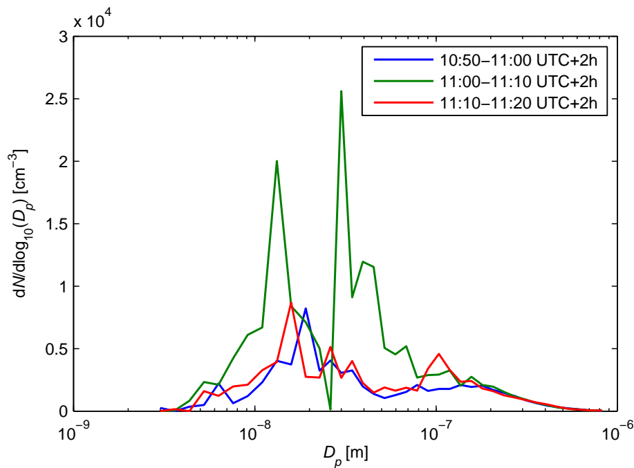
Figure 2. Three particle number size distributions from 2 March 2015 according to the old inversion algorithm, which assume stationary particles size distributions during each scan.
