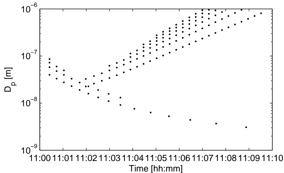
Figure 4. Training inputs for the scan on 2 March between 11:00 and 11:10 UTC +2h. For clarity we put D_p instead of u on the second axis.
