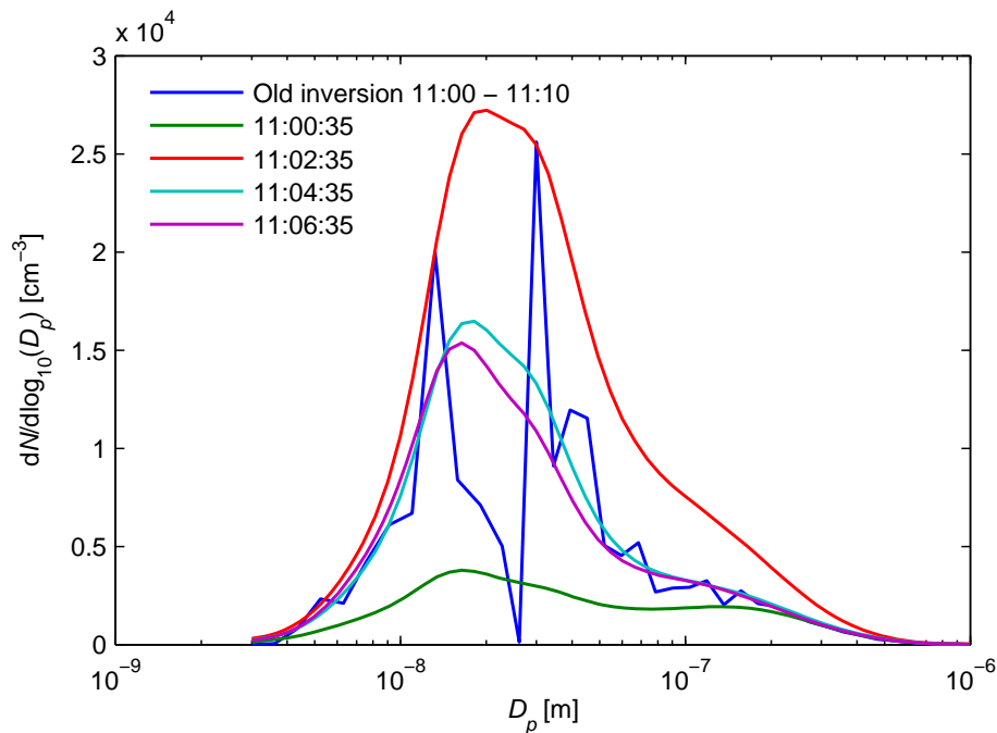
Figure 9. Expected size distribution before, during, and after the peak on 2 March at 11:03 UTC +2 h, and the result of the old inversion algorithm for the scan between 11:00 and 11:10 UTC +2 h.
