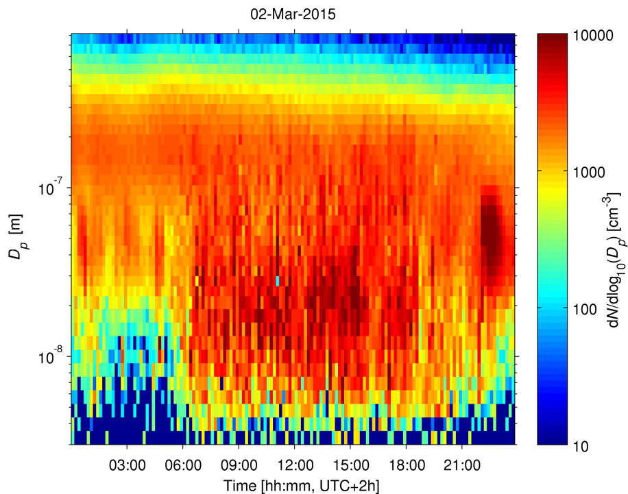
Figure 1. Size distributions from 2 March 2015 according to the old inversion algorithm, which assume stationary particles size distributions during each scan.
