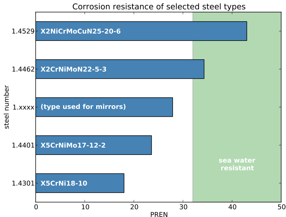
Figure 6. PREN for common stainless steel types. Steel numbers and grades are according to the European EN 10088-3 norm (European Committee for Standardization, CEN). The steel type labeled as 1.xxxx is the one that was chosen for the mirrors.
