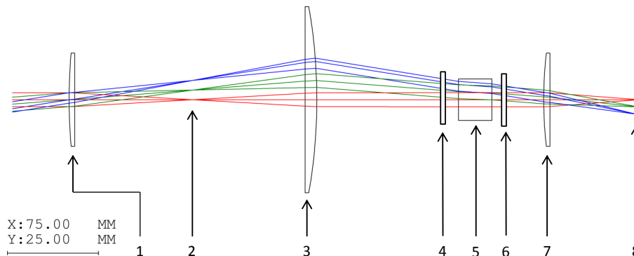
Figure 4. Ray Tracing diagram of the telescopic lens system for ALI simulated by Code V optical design software. The elements in the system are the following: (1) 150 mm length plano-convex lens. (2) Field stop. (3) 100 mm focal length plano-convex lens. (4) Vertical linear polarizer. (5) Brimrose AOTF. (6) Horizontal linear polarizer. (7) 50.4 mm focal length bi-convex lens. (8) Imaging plane.
