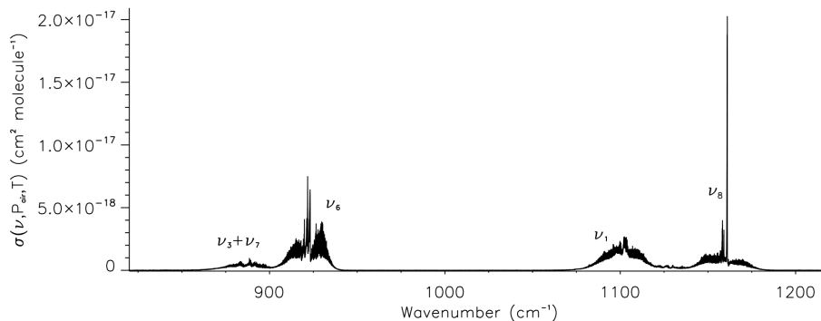
Figure 1. The IR absorption cross section of dichlorodifluoromethane/dry synthetic air at 268.9 K and 7.54 Torr, providing vibrational band assignments over the spectral range covered in this work.
