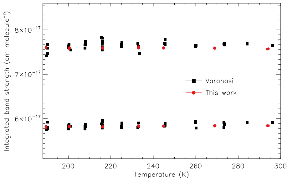
Figure 2. A plot of integrated band strength vs. temperature for each of the datasets over the wavenumber ranges 850–950 \text{cm}^{-1} (bottom) and 1050–1200 \text{cm}^{-1} (top). The Varanasi data at each temperature display a small spread in values, most likely arising from calibration errors between sets of measurements taken at different times, and problems with dichlorodifluoromethane adsorption on cell walls. Refer to the text for a more detailed discussion.
