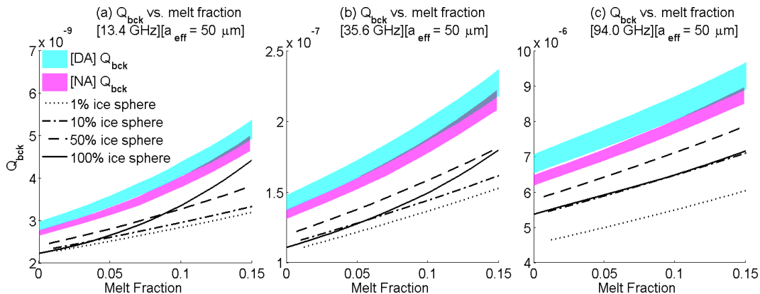
Figure 6. Similar to Fig. 4, the single-particle backscattering efficiency coefficient ( Q_{\text{bck}} ) is shown for 50 micron effective radius. Both aggregates show consistently larger backscattering efficiencies for the same mass as melt fractions compared to the spheres. Note the difference in the vertical axes on each panel.
