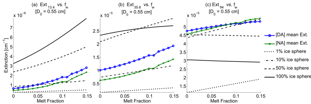
Figure 14. Same as Fig. 13 except for D_0 = 0.55 \text{ cm} . Note the different scaling on the vertical axes, including the exponents.
