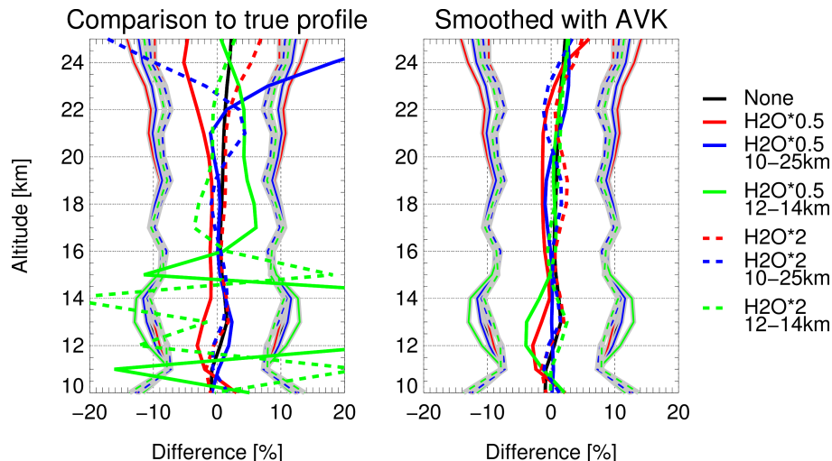
Figure 3. End-to-end tests for an unperturbed atmosphere (black lines) and for different perturbations of the water vapour profile (coloured solid and dashed lines). All lines show the difference between retrieved and reference profile divided by the reference. The coloured solid lines show the error for profiles with halved water vapour for the complete profile (0–60 km, red), the retrieval heights (10–25 km, blue), and a 2 km layer (12–14 km, green). The coloured dashed lines show the differences for doubled water vapour profiles in the same height ranges as for half of the water vapour. The left panel shows the comparison between the retrieval result and the original water vapour profile. In the right panel the original profile is smoothed with the AVK resulting from the retrieval to exclude differences caused by the resolution. The lines underlaid with a grey shading show the retrieval precision based on a constant SNR of 500.
