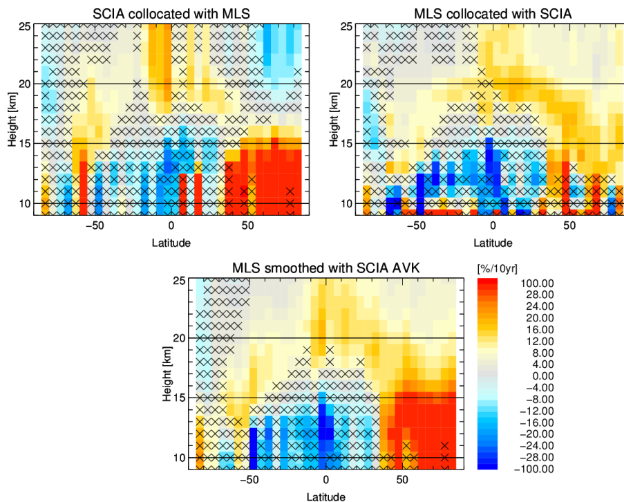
Figure 20. Linear trend for zonal monthly mean collocated data from SCIAMACHY and MLS (unsmoothed and smoothed with SCIAMACHY AVKs). Collocations are found between August 2004 and March 2012.
