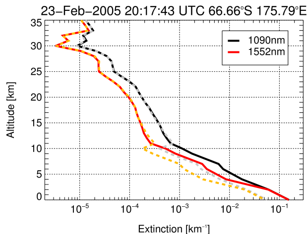
Figure 2. Aerosol extinction profiles for V3 (dashed lines) and V3.01 (solid lines) for the two wavelength used in the aerosol retrieval (1090 nm black and grey line, 1552 nm red and orange line).
