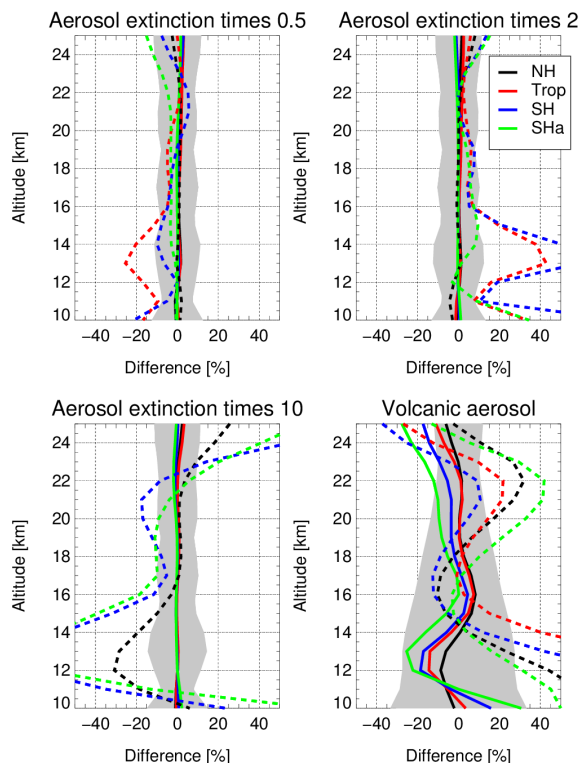
Figure 5. End-to-end test for different perturbations of the aerosol profile. In both upper panels and in the lower left panel the dashed lines show cases where the whole aerosol extinction profile (0–100 km) is perturbed by multiplying by a factor (given in the title of each panel), solid lines show cases where the perturbation is limited to 0–30 km. The lower right panel shows cases where the background aerosol profile is exchanged with cases for aged moderate (solid lines) and fresh high (dashed lines) volcanic aerosol according to the LOWTRAN model. The four colours show different observation geometries. The smoothing with the AVK is done for all cases. The grey shading shows the maximum of retrieval errors.
