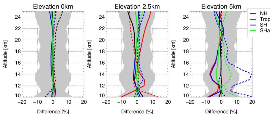
Figure 4. End-to-end test for a perturbed albedo and effective elevation. The comparison is done in similar a manner to Fig. 3 for an albedo of 0.1 (solid lines) and 0.7 (dashed lines). The different surface elevations (0, 2.5, and 5 km) are shown in the different panels. The colours mark observation geometries for different regions (NH and SH mid latitudes, tropics and SH Arctic). The smoothing with the AVK is done for all cases (but has no effect here). The grey shading shows the maximum of retrieval errors.
