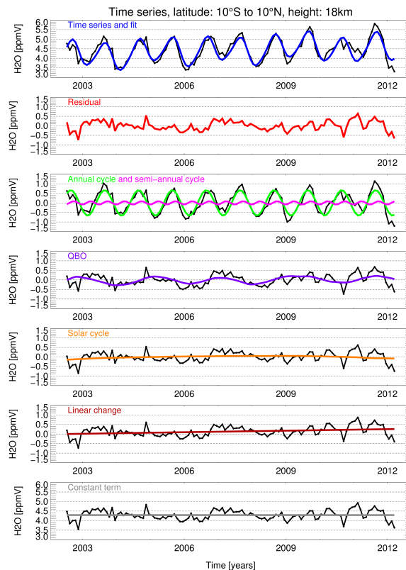
Figure 9. Monthly mean zonal mean water vapour volume mixing ratio time series from SCIAMACHY for 10°S–10°N and 18 km height. The black line in the top panel shows the SCIAMACHY time series. The coloured lines in the lower panels show the different fit parameter terms, the red line in the second panel the residual. In the lower panels the black curves show the fit parameter terms shown in the corresponding panel plus the residual shown in the second panel.
