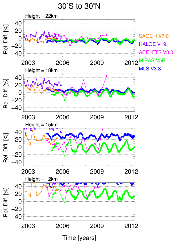
Figure 19. Like Fig. 17 for the Tropics (30° S–30° N).
