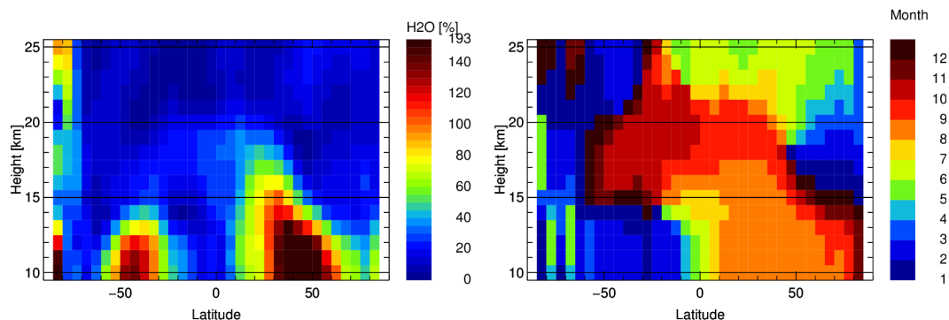
Figure 11. Amplitude and month of the maximum (1: January, 12: December) for the annual cycle from the multivariate linear regression applied to SCIAMACHY data on a 5° latitude and 1 km height grid.
