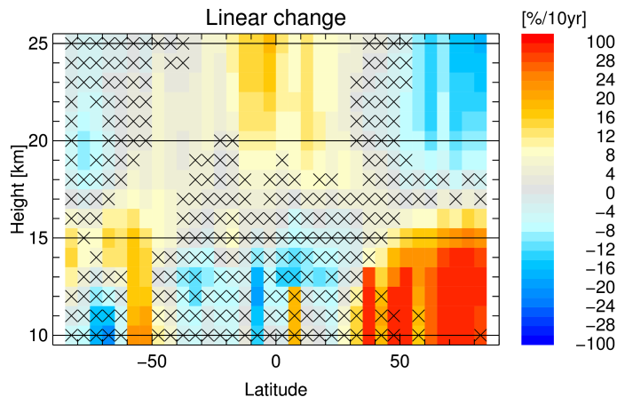
Figure 10. Linear change from the the multivariate linear regression for SCIAMACHY zonal mean data on a 5° latitude and 1 km height grid. Non significant values ( < 2\sigma ) are marked with crosses.
