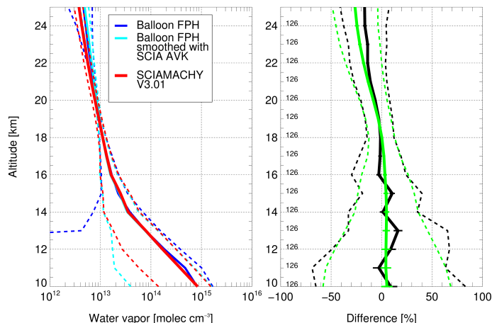
Figure 12. Left panel: Mean profiles over all collocations from SCIAMACHY and balloon borne data (the two lines show the data interpolated on the retrieval grid of SCIAMACHY and smoothed with the AVK of SCIAMACHY, respectively) and their standard deviations (dashed line). Right panel: Mean percentage difference between SCIAMACHY water vapour profiles and balloon borne profiles interpolated to the SCIAMACHY retrieval grid (black line) and smoothed with the AVK of SCIAMACHY (green line). The dotted lines show the standard deviation, the error bars (if visible) depict the standard error of the mean. The number of collocations is given for each altitude.
