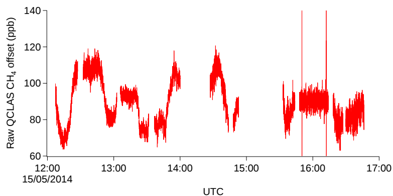
Figure 5. The offset between the raw QCLAS \text{CH}_4 data and the calibrated FGGA data (used here as our reference) during flight B848. Gradients of over 30 ppb in less than 10 min can be seen to be present.
