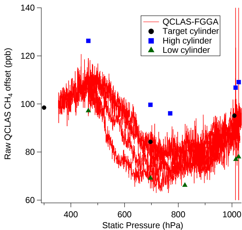
Figure 6. The offset between the raw QCLAS \text{CH}_4 measurements and both the corresponding calibrated FGGA data and the known contents of the target, high and low calibration cylinders during flight B848, shown as a function of static pressure. Although the absolute magnitude of the offset differs for these four different measurements, the same broadly repeatable pattern is exhibited by each of them.
