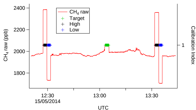
Figure 4. A selection of raw CH 4 data from flight B848, overlaid with calibration index markers to highlight the hourly calibration cycle. The target cylinder measurement (green markers) is performed approximately mid-way between the high-low span cylinder measurements (black and blue markers respectively) used to calibrate the data to the WMO scale.
