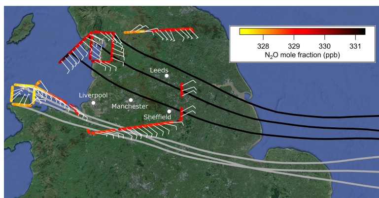
Figure 10. Aircraft flight track for flight B868, coloured by \text{N}_2\text{O} mole fraction. Average wind speeds and directions taken over 60 s are shown as a wind bars (using the convention where each full barb represents a wind speed of 10 knots). Selected HYSPLIT back trajectories are shown for a region of enhanced \text{N}_2\text{O} (black) and a contrasting region of lower \text{N}_2\text{O} (grey). Map data: Google, SIO, NOAA, U.S. Navy, NGA, GEBCO, Landsat.
