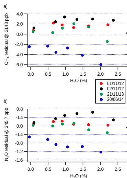
Figure 2. Residual error due to the influence of water vapour for the retrieval of (a) \text{CH}_4 and (b) \text{N}_2\text{O} after applying an empirically derived scale factor to correct the data. Data from four identical experiments is shown; the residuals are calculated as the product of the fractional error for each measurement and the average mole fraction for the dry measurements taken during all four experiments.
