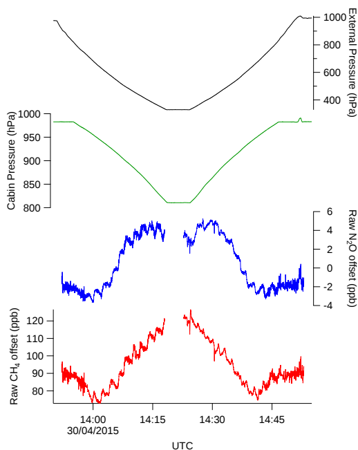
Figure 8. Time series showing the offset between the raw retrieved QCLAS mole fractions and the known content of the target cylinder being sampled. Cabin pressure and external static pressure are also shown to illustrate the systematic nature of the offset during two consecutive profiles.
