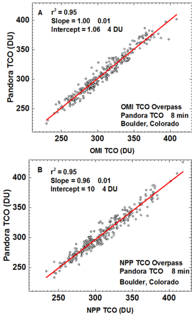
Figure 7 Scatter plot comparisons A. between Pandora ozone measurements and those from OMI and B. Pandora comparison with those from NPP.
