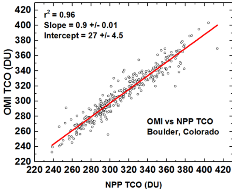
37 Figure 9 Scatter plot of NPP vs OMI TCO
