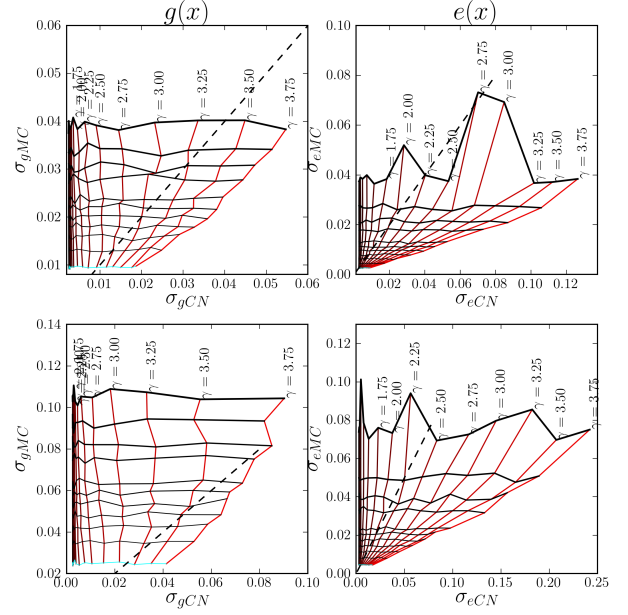
Figure 2: Results of the Monte Carlo. First column presents the results for g(x) , the second for e(x) . In the first row curves are more steep, the Gaussian curve is calculated with a standard deviation of 0.25. In the second row the curves are more gentle with the standard deviation of the Gaussian curve set to 0.5. The horizontal axes shows the average errors obtained using our methodology. The vertical axes shows the standard deviation of the location obtained using the algorithms. Almost horizontal lines define the noise applied to the curves starting from 0.5% to 10% of the maximum value which is 1000. The almost vertical lines represent different \gamma thresholds used for the calculation of U_\gamma(x_m) . The dashed line is the identity.
