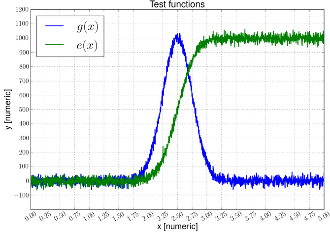
Figure 1: Two examples of curves used, a Gaussian curve g(x) and a sigmoid function e(x) set to have maximum value equal to 1000 and with applied normal noise of standard deviation =20.
