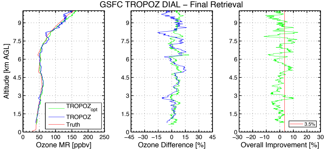
Fig. 8: The left panel compares the final retrieved ozone concentration from the previous TROPOZ retrieval and the optimized retrieval (TROPOZ opt ) to the known ozone profile used in the simulated lidar return signal. The center panel shows the differences in percentage from the known profile and retrieved TROPOZ and TROPOZ opt profiles. The right panel shows the improvement from the optimized TROPOZ opt retrieval and the original TROPOZ retrieval in percentage. The mean improvement (red line) is 3.5%.
