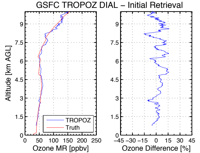
Fig. 1: The left panel shows the initial retrieved ozone concentration from the TROPOZ algorithm described in Sullivan et al. (2014) as compared to the known ozone profile used in the simulated lidar return signals. The right panel shows the percent difference from the known profile and retrieved profile.
