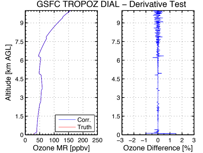
Fig. 2: The left panel shows the initial retrieved ozone concentration from the TROPOZ algorithm using the Savitzky-Golay differentiation filter for the numerical derivative as compared to the known ozone profile used in the simulated lidar return signals. The right panel shows the percent difference from the known profile and retrieved profile.
