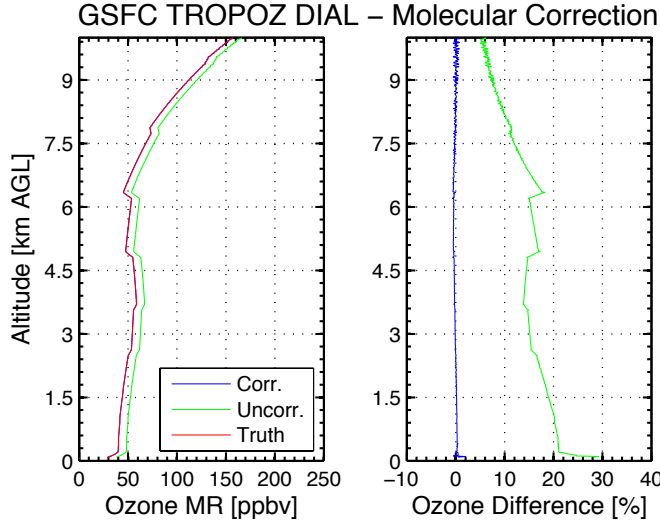
Fig. 4: The left panel shows the retrieved ozone mixing ratios from the corrected and uncorrected TROPOZ ozone profiles as compared to the known ozone profile used in the simulated lidar return signal. The right panel shows the percent difference from the known profile and retrieved profile.
