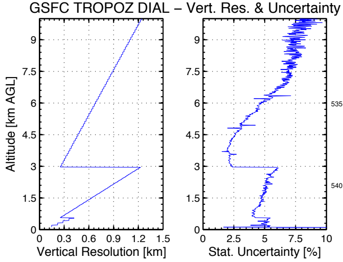
Fig. 7: The left panel shows the associated vertical resolution in the TROPOZ_{opt} retrieval algorithm which is derived from the windows size of the SG differentiation filter. The right panel shows the statistical uncertainty in the system associated with these vertical resolutions, which is an approximation for the overall uncertainty for the TROPOZ_{opt} .
