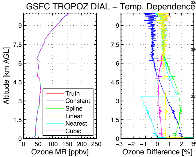
Fig. 3: The left panel shows the retrieved ozone mixing ratio from the varying TROPOZ interpolations of the temperature dependence of ozone absorption cross sections as compared to the known ozone profile used in the simulated lidar return signal. The right panel shows the percent difference from the known profile and retrieved profile.
