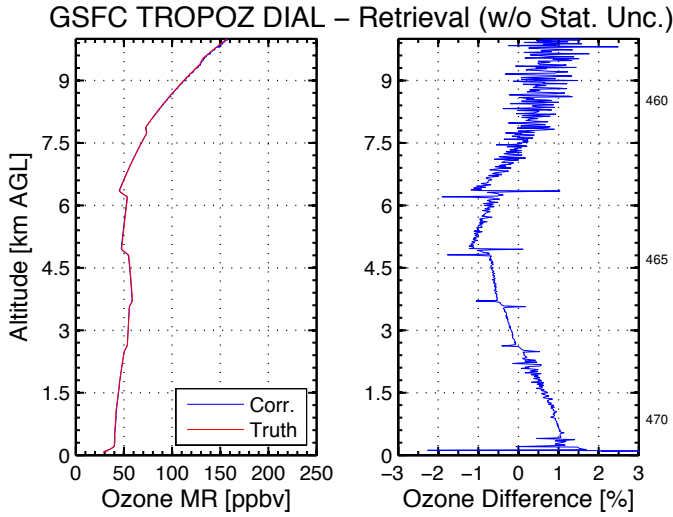
Fig. 6: The left panel shows the retrieved ozone mixing ratios from the TROPOZ opt ozone profiles as compared to the known ozone profile used in the simulated lidar return signal without the addition of statistical noise. The right panel shows the percent difference from the known profile and retrieved profile.
