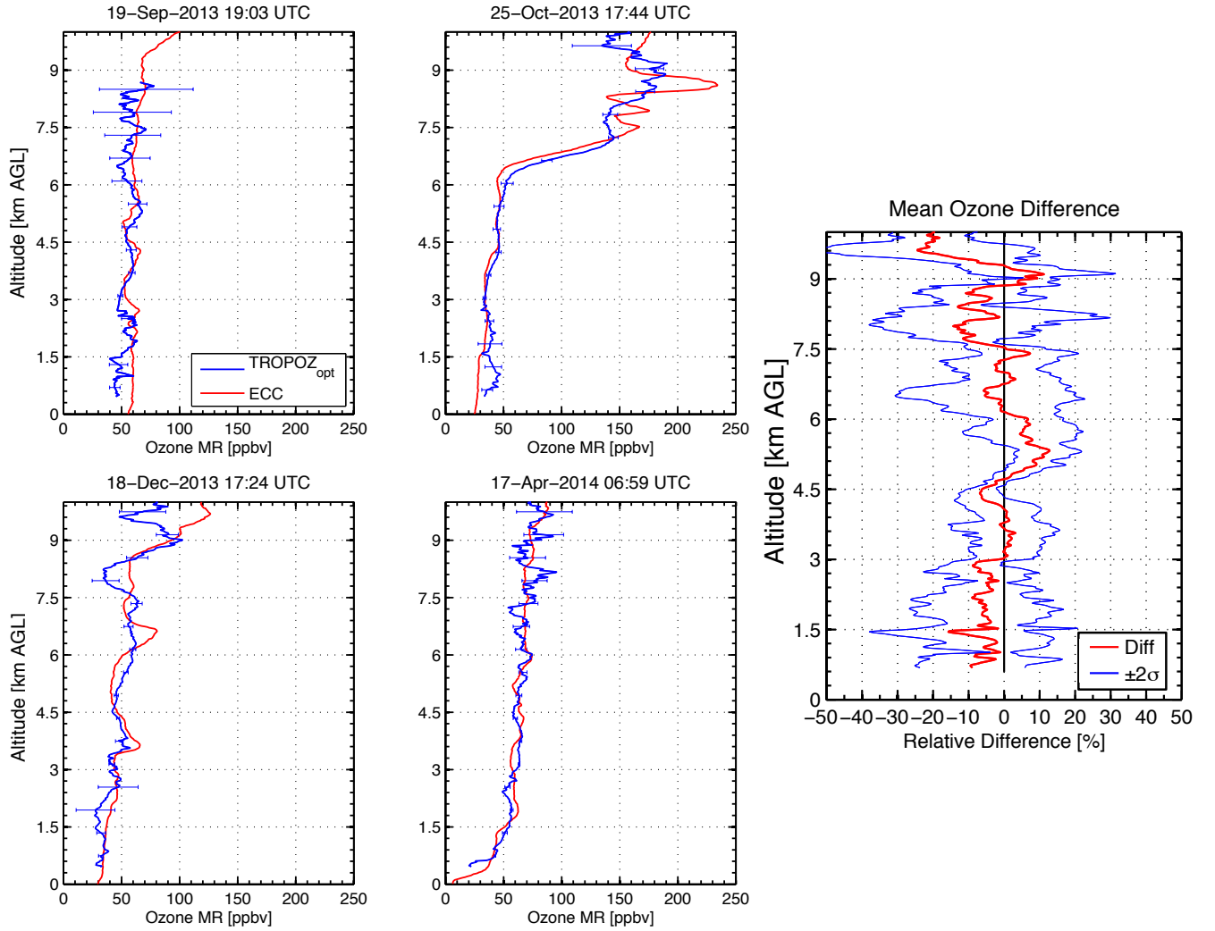
Fig. 9: Comparisons between four nearby ECC ozonesonde launches and the updated TROPOZ opt retrieval algorithm.
