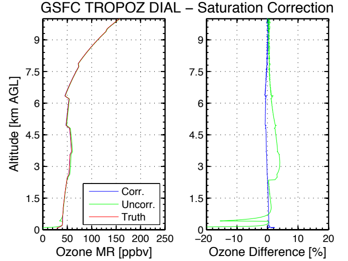
Fig. 5: The left panel shows the retrieved ozone mixing ratios from the saturation corrected and uncorrected TROPOZ ozone profiles as compared to the known ozone profile used in the simulated lidar return signal. The right panel shows the percent difference from the known profile and retrieved profile.
