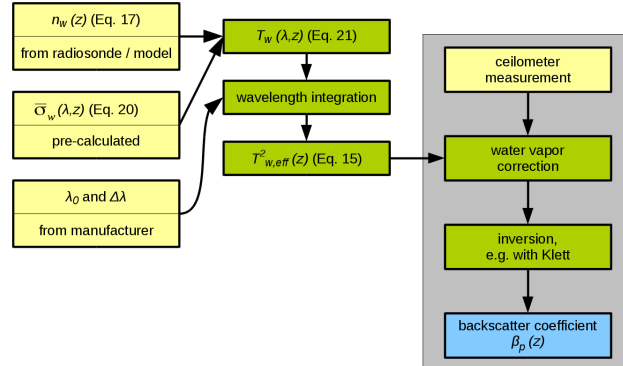
Figure 4: Flow chart of WAPL: correction for water vapor absorption in the determination of the aerosol backscatter coefficient \beta_p (blue box). The yellow boxes indicate the input required for WAPL whereas steps concerning calculations are shown in green.
