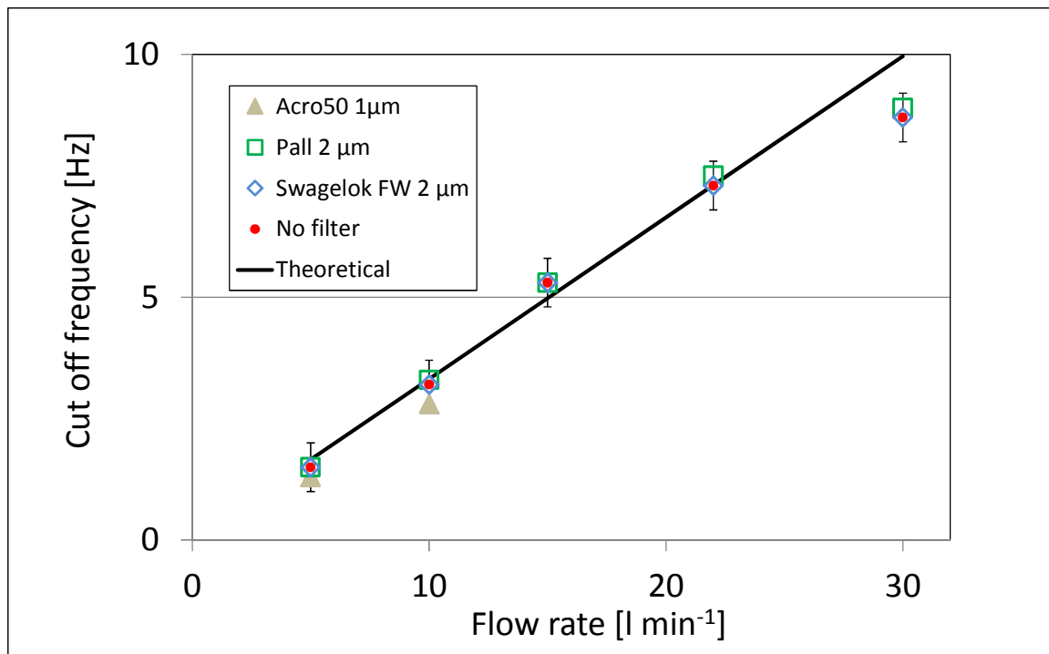
Fig 4: Cut-off frequencies [Hz] as a function of the flow rate (l/min) for LI-7200 with ACRO-50 (grey triangle), Pall 2µm (green squares), Swagelok FW 2µm (blue diamonds), and without any filter (red dots). The full line corresponds to the theoretical prediction given by equation (2).
