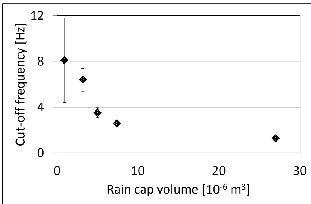
Figure 6 : relation between different rain cap volumes and GSS cut off frequency at a 15 L min -1 flow rate.
